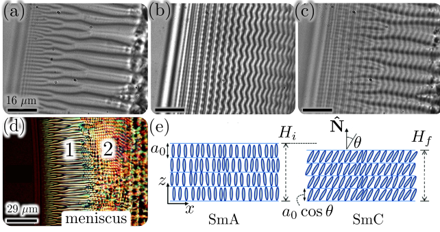
FIG. 23 (a) Bright-field (transmitted light) optical micrographs of the meniscus of a smectic- C^* film (compound SCE-9, T = 25 degrees C). (b) Interferogram of the sample at the same location as in (a), obtained with phase shifting interferometry (PSI), reveals distorted interference fringes. (c) Superposition of the micrographs in (a) and (b), show how the \mathbf{c} -director splay distortions seen in bright-field correspond to the interface undulations captured by the interferogram. (d) Polarized micrograph of the smectic- C^* meniscus reveals two regions: region 1 exhibits radial stripes, shown also in (a) and region 2 shows a two-dimensional structure of focal conic domains. (e) Schematic depicting the HH instability as a possible origin of smectic layer undulations from the smectic-A—smectic-C phase transition (left is before, right is after the transition). After the phase transition, the director tilts with an angle \theta , causing the natural layer spacing of a_0 to reduce to a_0 \cos \theta . Although the phase transition causes a decrease in the natural layer thickness, the gradient in meniscus thickness fixes in a certain number of dislocations in the system, thereby fixing in a certain number of layers and the thickness. A mechanical stress analogous to a dilation of the smectic-C layers results from this incompatibility, triggering undulations to accommodate the director tilt. Adapted from (Selmi et al. , 2017).
