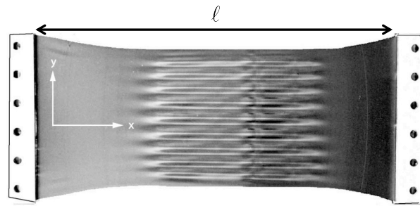
FIG. 30 Photographs of wrinkles in a stretched elastic sheet having a characteristic periodicity given by \lambda^* \approx 2\sqrt{\pi\lambda\ell} , where \ell is the film length and \lambda \sim (B/T)^{1/2} is an elastic characteristic length scale, where B is the bending stiffness and T is the tension in the film. Note how similar this wavelength is to the classic Helfrich-Hurault instability size given in Eq. (19). (Adapted from (Cerdeja and Mahadevan, 2003)).
