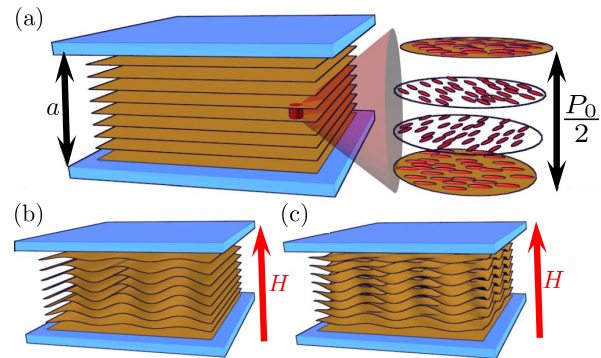
FIG. 1 Schematic of the classic Helfrich-Hurault instability in a cholesteric liquid crystal. The mesophase is confined between solid substrates with planar anchoring and can be described as a lamellar system of period P_0/2 (a). Undulation in the periodic layers of the cholesteric along a single (b) or along two perpendicular directions (c) develops under an applied magnetic field ( H ) of sufficient magnitude.
