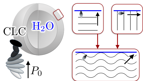
FIG. 11 Schematic of a cholesteric liquid crystal shell. The red insets illustrate how changing the anchoring at the shell interface alters the pitch axis orientation, which can lead to a HH-like instability in the bulk (bottom right). From (Lavrentovich and Tran, 2020).
