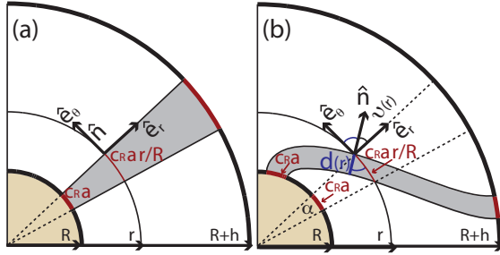
FIG. 17 Schematics of a smectic confined between two cylinders of radii R and R+h . The anchoring is planar on the confining boundaries. (a) In absence of dislocations, a radial texture necessarily induces some dilation in the thickness of a smectic layer (shaded region). (b) The absence of dilation in the bulk implies that the “orthoradial” thickness of a layer d varies with the radial coordinate r . However, some dilation is necessarily ejected to the outer surface.
