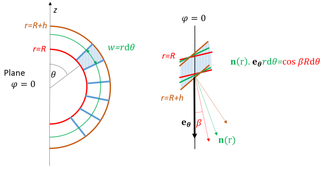
FIG. 37 Left: Cross section of a smectic shell in the plane \varphi = 0 . We consider layers (in blue) that are perpendicular to the inner and outer spheres (respectively located at r = R and r = R+h ). The apparent thickness of the layers in this plane, w , linearly increases with the radius r . Right: Because the actual thickness of the layers w\hat{e}_\theta \cdot \mathbf{n} is uniform, this constrains the form of the director to Eq. (A1).
