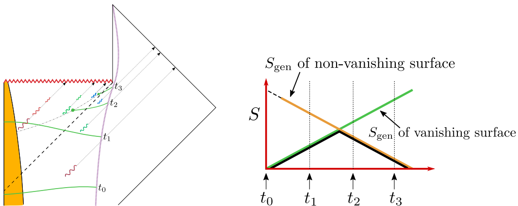
Figure 13: The Page curve for the fine-grained entropy of the black hole (shown in black) is captured by the transition between a growing contribution from the trivial surface and a decreasing contribution from a non-trivial surface near the black hole horizon.
