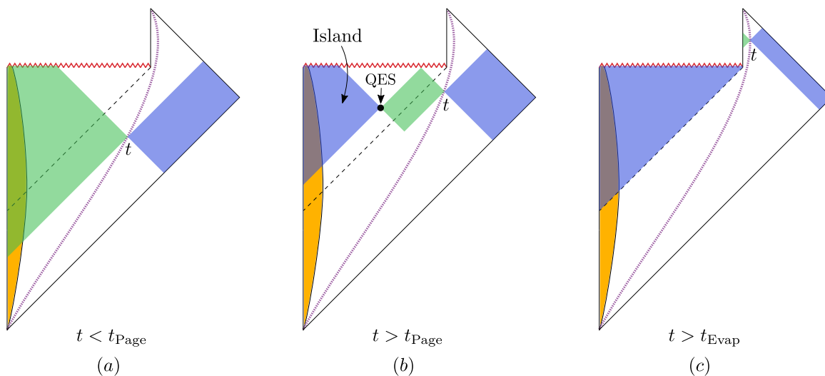
Figure 18: In green we show the entanglement wedges of the black hole and in blue the entanglement wedges of the radiation region. Different figures show the wedges at different times. They are different because there is transfer of quantum information through the cutoff surface. To describe the white regions we need information both from the black hole region and the radiation region.
