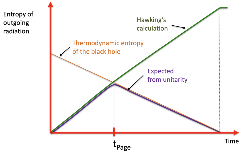
Figure 7: Schematic behavior of the entropy of the the outgoing radiation. The precise shape of the lines depends on the black hole and the details of the matter fields being radiated. In green we see Hawking’s result, the entropy monotonically increases until t_{\text{End}} , when the black hole completely evaporates. In orange we see the thermodynamic entropy of the black hole. If the process is unitary, we expect the entropy of radiation to be smaller than the thermodynamic entropy. If it saturates this maximum, then it should follow the so called “Page” curve, denoted in purple. This changes relative to the Hawking answer at the Page time, t_{\text{Page}} , when the entropy of Hawking radiation is equal to the thermodynamic entropy of the black hole.
