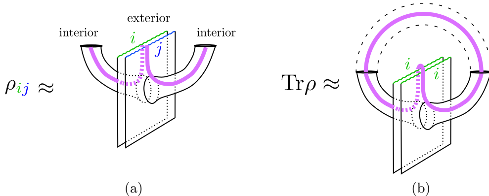
Figure 20: (a) Path integral representation of the matrix elements \rho_{ij} . (b) Path integral representation of \text{Tr} \rho . Regions with repeated indices are identified in this figure and the figures that follow. The purple line represents entanglement.
