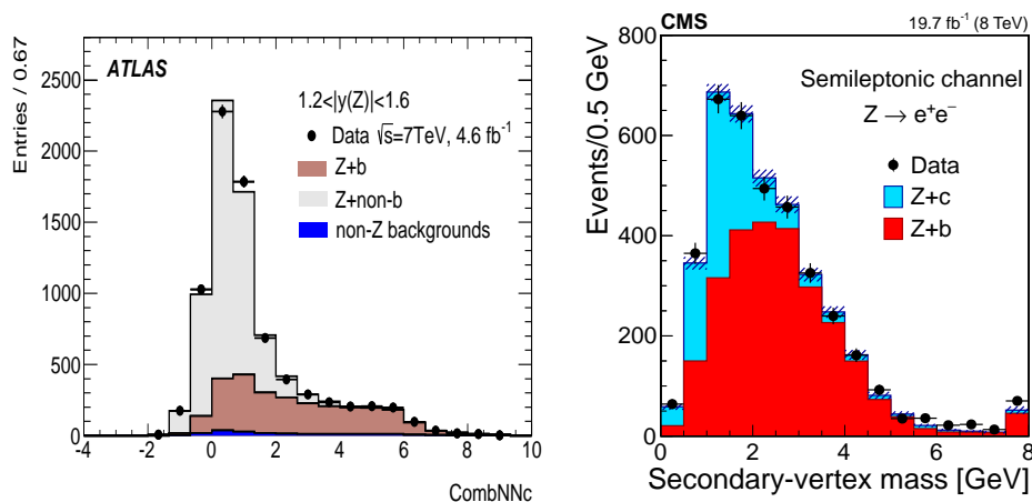
Figure 55 Combined neural network output distribution providing separation between jet flavors in Z + jet events at 7 TeV (left), figure taken from (ATLAS Collaboration, 2014b). Secondary-vertex mass distributions for jets associated to a Z boson decaying to electrons, after background subtraction, at 8 TeV (right), figure taken from (CMS Collaboration, 2018c).
