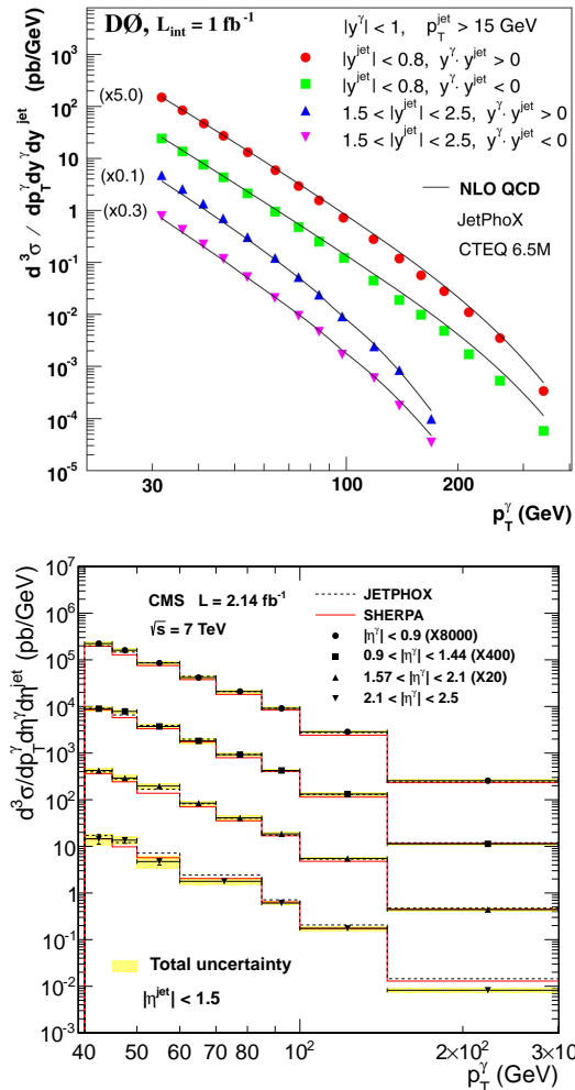
Figure 19 Triple differential cross sections as a function of p_T^\gamma in four photon rapidity intervals in p\bar{p} collisions at 1.96 TeV center-of-mass energy at the TEVATRON, figure taken from (D \phi Collaboration, 2008b) (top), and in four different ranges of \eta^\gamma for p_T^\gamma > 30 GeV and |\eta^{\text{jet}}| < 1.5 in pp collisions with 7 TeV center-of-mass energy at the LHC (bottom), figure taken from (CMS Collaboration, 2014e). The measured cross sections are compared with the NLO pQCD calculation by JETPHOX and with the LO MC SHERPA simulation (bottom).
