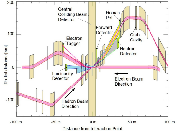
FIG. 20 Layout of the eRHIC interaction region. The length scales for the horizontal and vertical axis are very different. Beams cross with a crossing angle of 25 mrad. The IR design integrates focusing magnets for both beams, luminosity and neutron detectors, electron taggers, spectrometer magnets, near-beam detectors (Roman pots for hadrons), crab cavities, and spin rotators for both beams (from (Willeke et al. , 2019)).
