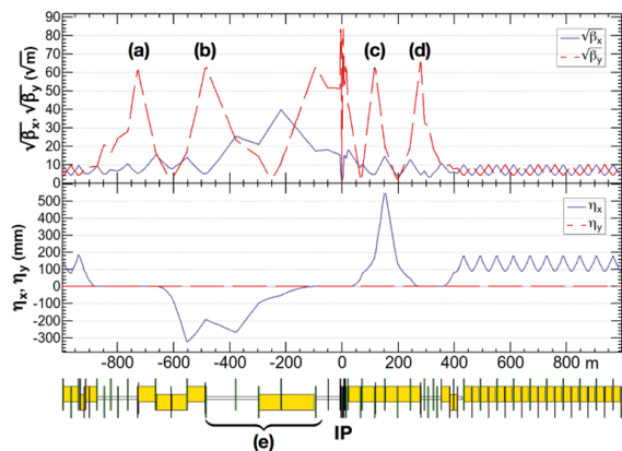
FIG. 27 Asymmetric final-focus optics of FCC-ee, featuring four sextupoles (a–d) for local vertical chromaticity correction combined with a virtual crab waist (see text for details) (Benedikt et al. , 2019a; Oide et al. , 2016).
