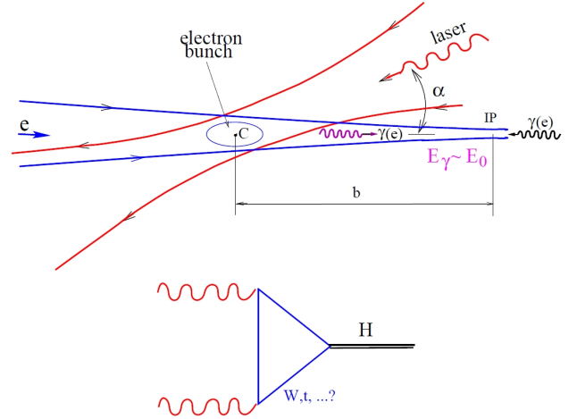
FIG. 40 (top) Scheme of \gamma\gamma , \gamma e collider; (bottom) Higgs production diagram in \gamma\gamma collisions (from Ref. (Tel'nov, 2014)).
