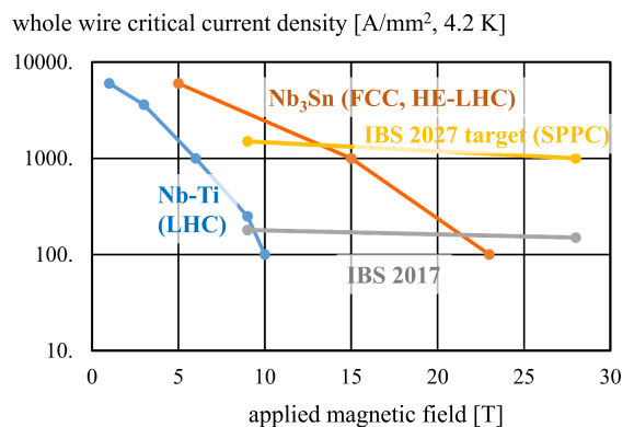
FIG. 30 Field limits for LHC-type Nb-Ti conductor, Nb 3 Sn conductor as used for HL-LHC, FCC-hh and HE-LHC, and iron-based superconductor (present and 10-year forecast) for SppC (after P.J. Lee (P.J.Lee (NHMFL), Engineering Critical Current Density vs. Applied Field), and private communication J. Gao, from Ref. (Benedikt and Zimmermann, 2018)).
