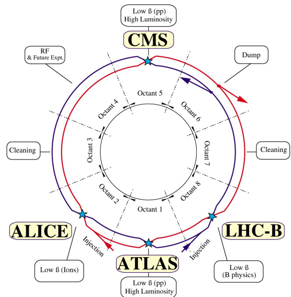
FIG. 14 Layout of the LHC double ring, with its eight long straight sections hosting two general and two special-purpose experimental detectors and/or devoted to specific accelerator functions, such as betatron collimation (cleaning), momentum collimation, beam extraction, RF systems and diagnostics, and injection (Image credit: CERN, 1997 (LHC-PHO-1997-060-1), under license CC-BY-4.0).
