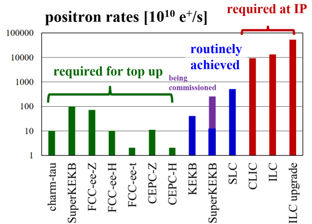
FIG. 26 Positron production rates achieved at the SLC, KEKB and SuperKEKB compared with the need for top-up injection at future circular and linear e^+e^- colliders (adapted from Ref. (Benedikt et al. , 2020), license CC-BY-4.0).
