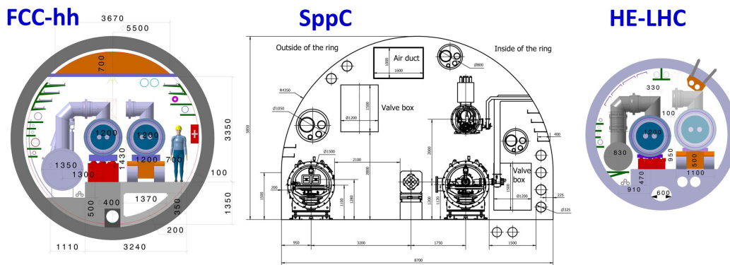
FIG. 32 Tunnel cross sections for FCC-hh, SppC, and HE-LHC, approximately to scale (from Ref. (Benedikt and Zimmermann, 2018)).
