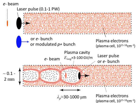
FIG. 37 Concept of the plasma wakefield acceleration driven either by a short laser pulse (LWFA), or by a short electron bunch or by long(er) modulated proton bunch (PWFA), adapted from (Assmann and Grebenyuk, 2014), under license CC-BY-3.0).
