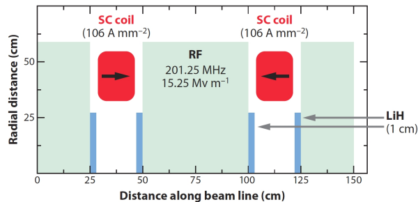
FIG. 35 Ionization cooling-channel section. 200 MeV muons lose energy in lithium hydrate (LiH) absorbers (blue) that is replaced when the muons are reaccelerated in the longitudinal direction in RF cavities (green). The few-Tesla SC solenoids (red) confine the beam within the channel and radially focus the beam at the absorbers. Some representative component parameters are also shown (from Ref. (Geer, 2009)).
