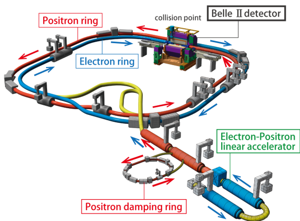
FIG. 12 Schematic of SuperKEKB (Image credit: KEK).
