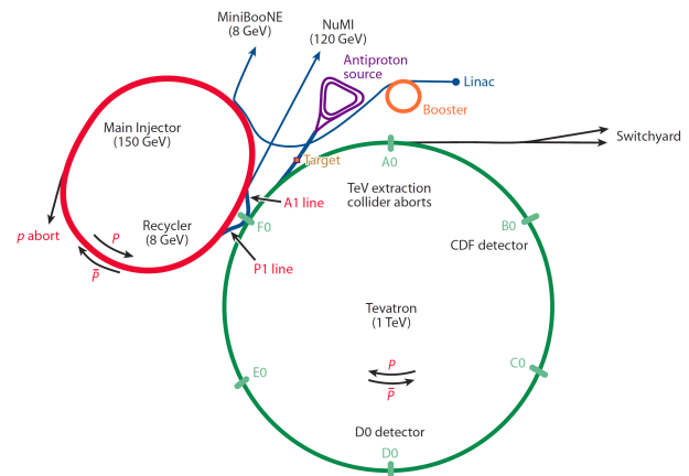
FIG. 10 Layout of the Fermilab accelerator complex. The accelerators are shown to scale; the radius of the Tevatron is 1.0 km. Proton beam energy out of the linac is 400 MeV and 8 GeV out of the Booster synchrotron; the energy of antiprotons in the antiproton source (triangular shape Debuncher and Accumulator) is also 8 GeV (from (Holmes and Shiltsev, 2013)).
