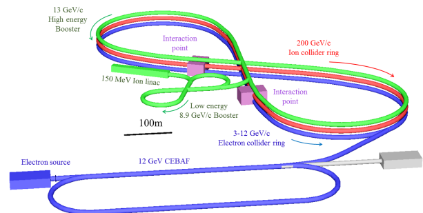
FIG. 18 Layout of the Jefferson Lab Electron-Ion Collider (JLEIC) (adapted from (Zhang, 2019), license CC-BY-3.0).
