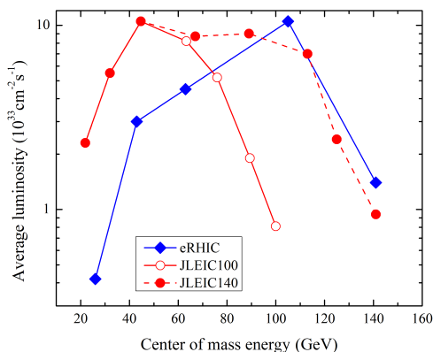
FIG. 19 Average e - p luminosity of JLEIC and eRHIC as a function of c.m.e. The JLEIC average luminosity takes into account a 75% operational duty factor and is given for both baseline design (open circles) and for a potential future upgrade with a 400 GeV proton ring (solid circles). The eRHIC luminosity is averaged over the data-taking cycle and equals 95% of the peak luminosity.
