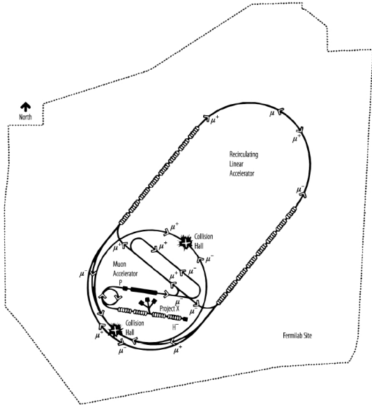
FIG. 34 Schematic of a 4 TeV Muon Collider on the 6×7 km FNAL site (from Ref. (Myers and Schopper, 2013, Ch. 12.2)).
