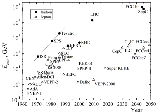
FIG. 2 Center of mass energy reach of particle colliders vs their start of operation. Solid and dashed lines indicate a ten-fold increase per decade for hadron (circles) and lepton (triangles) colliders (adapted from (Shiltsev, 2012a)).
