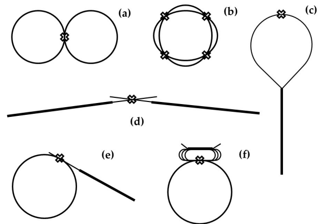
FIG. 1 Schematics of particle collider types.
