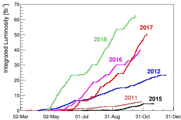
FIG. 15 Integrated yearly luminosity between 2011 and 2018 for proton operation (from (Steerenberg et al. , 2019), under license CC-BY-3.0).
