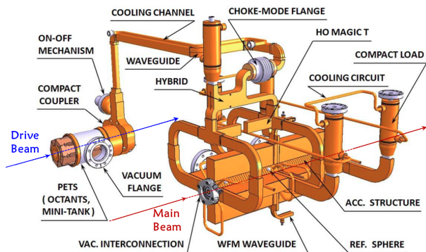
FIG. 23 3D model of the CLIC two-beam RF module (adapted from (Aicheler et al. , 2012), image credit: CERN, license CC-BY-3.0).
