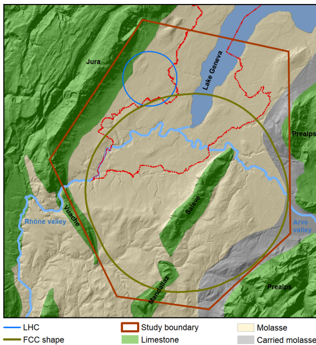
FIG. 29 Study boundary (red polygon), showing the main topographical and geological structures, LHC (blue line) and FCC tunnel trace (brown line) (Benedikt et al. , 2019a,c).
