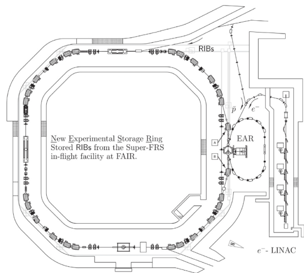
FIG. 17 Conceptual layout of the planned electron(antiproton)-ion collider hosting the ELISe experiment. The intersection region A - B is situated in a bypass section to the New Experimental Storage Ring (NESR) and hosts a dedicated spectrometer (from (Antonov et al. , 2011)).
