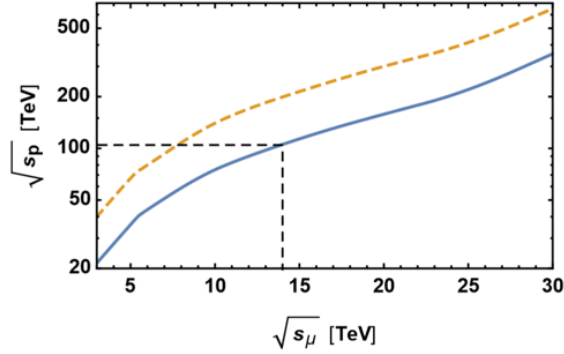
FIG. 33 Energy reach of muon-muon collisions: the energy at which the proton collider cross-section equals that of a muon collider (from Ref. (Delahaye et al. , 2019)). The plot compares the pair production cross-sections for heavy particles with mass M approximately equal to half the muon collider energy \sqrt{s_\mu}/2 . The dashed yellow line assumes comparable processes for muon and proton production, while the continuous blue line accounts for the possible QCD enhancement on the proton production.
