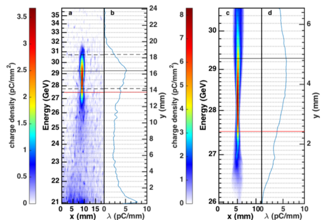
FIG. 38 A 0.1 nC electron bunch gained a maximum energy of 9 GeV in a 1.3 m-long electron plasma wakefield accelerator driven by a 20.35 GeV e^- beam at the FACET facility at SLAC: (a)–(d) show the energetically dispersed transverse charge density profile spectra and the horizontally integrated spectral charge density profiles as observed on the wide-field of view Cherenkov screen and on the order of magnitude more sensitive Lanex screen, respectively (from Ref. (Litos et al. , 2016), license CC-BY-3.0).
