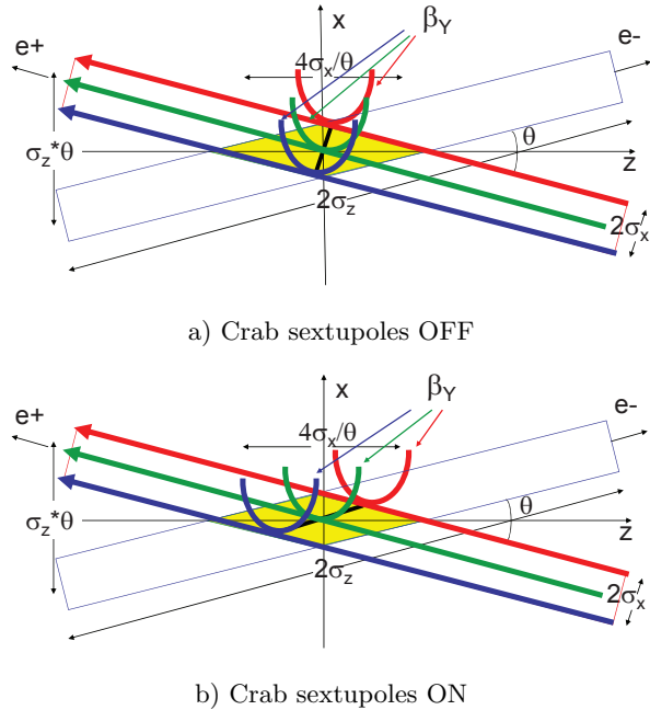
FIG. 11 Crab waist collision scheme (Raimondi et al. , 2008) (license CC-BY-3.0).
