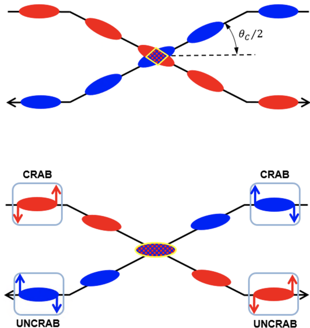
FIG. 9 Top: beam collision scheme with crossing angle suffers from geometric luminosity reduction. Bottom: crab-crossing scheme that results in full bunch overlapping and thus maximum luminosity. Deflecting RF cavities generate a null kick to the center of the bunch while its head and tail receive opposite transverse kicks (adapted from (Verdu-Andres et al. , 2016)).
