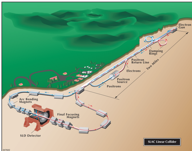
FIG. 7 The Stanford Linear Collider (SLC). Polarized electrons are produced by photoemission from a Ti:sapphire laser and a GaAs photocathode at the electron gun, accelerated to 1.2 GeV, injected into a damping ring (DR) to reduce e^- beam emittance (size), then kicked back into the 3 km long linac to be accelerated together with positrons to 46.6 GeV, then separated magnetically and transported along two arcs and collide head-on at the IP. The positrons are produced by a fraction of 30 GeV e^- beam which is stopped in a target. e^+ 's are then collected and returned to the upstream end of the linac for many-fold emittance reduction in another DR (Image credit: SLAC).
