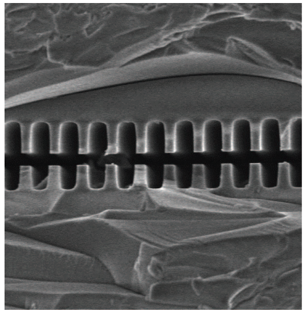
FIG. 41 Scanning electron microscope image of the longitudinal cross-section of a dielectric laser acceleration structure with 400 nm gap (Peralta et al. , 2013).
