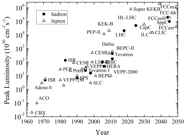
FIG. 3 Luminosities of particle colliders (triangles are lepton colliders and full circles are hadron colliders, adapted from (Shiltsev, 2012a)). Values are per collision point.
