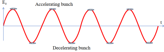
FIG. 39 Basic ERL principle: accelerating bunches take energy from SRF linac, while decelerating bunches return energy back (Litvinenko et al. , 2019).
