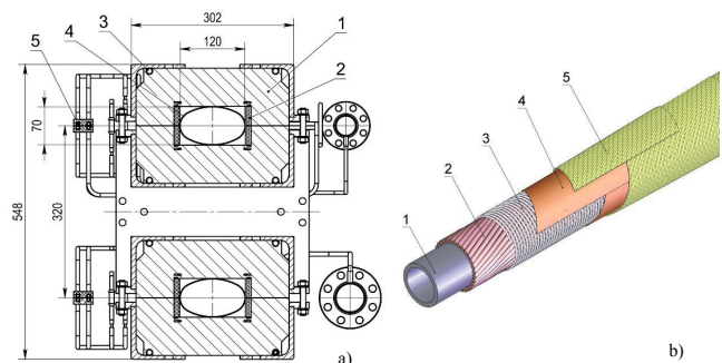
FIG. 16 Superferric 1.8 T magnets of the NICA collider: a) (left) cross-section of the magnet, based on a cold, window-frame iron yoke and a hollow superconductor winding: 1 — lamination, 2 — SC cable, 3 — yoke cooling tube, 4 — beam pipe, 5 — current carrying bus bars. The magnets are placed in a 4.5 K cryostat (not shown); b) (right) 10.4 kA SC cable: 1 — 3 mm diameter cooling tube, 2 — Nb-Ti SC wire, 3 — Ni-Cr wire, 4 and 5 — insulation tapes (adapted from (Khodzhibagiyani et al. , 2019)).
