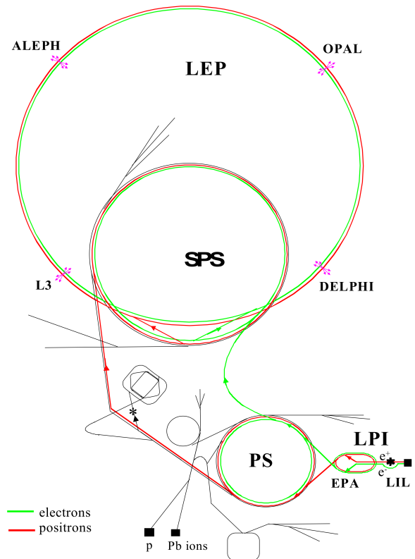
FIG. 8 Schematic view of the LEP injector chain of accelerators and the LEP storage ring (Baudrenghien and Collier, 1996) with the four experiments ALEPH, DELPHI, L3, and OPAL. The first part of the chain of injectors, the LEP pre-injector (LPI), consisted of two LEP injector linacs (LIL) and an electron/positron storage ring (EPA). Eight positron bunches, followed by eight electron bunches, were ejected from EPA to the Proton Synchrotron (PS), and then accelerated plus extracted to the Super Proton Synchrotron (SPS) for further acceleration. Positrons and electrons were injected into LEP from the SPS, initially at a beam energy of 20 GeV, and later (since 1995) at 22 GeV, to boost the bunch current, which was limited at injection by the TMCI. In its last year of operation (2000), the LEP reached a maximum e^+e^- collision energy of 209 GeV. (Image credit: P. Collier, CERN; available under license CC-BY-3.0).
