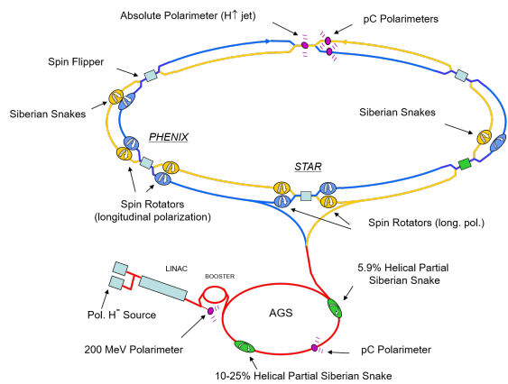
FIG. 13 Layout of the RHIC collider with its injector complex (adapted from (Ranjbar et al. , 2004)). The two RHIC rings cross in six points. The two principal experiments still running are PHENIX and STAR. The smaller experiments PHOBOS, BRAHMS and PP2PP have been completed. The LINAC is the injector for polarized protons into the Booster/AGS/RHIC chain. A jet target is used for precision beam polarization measurements. A tandem injector for ions has been replaced by an Electron Beam Ion Source (EBIS) starting with the 2012 run (Image credit: T. Roser, BNL).
