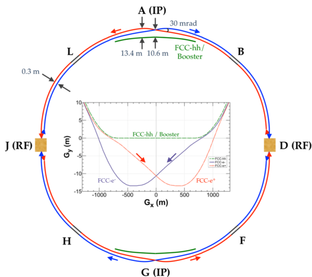
FIG. 28 Layout of the FCC-ee double ring collider with two long RF straights and two interaction points, sharing a tunnel with the full-energy top-up booster (Benedikt et al. , 2019a; Oide et al. , 2016).
