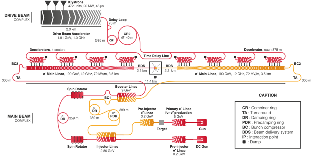
FIG. 24 CLIC accelerator complex layout at \sqrt{s}=380 GeV (S.Stapnes, Future Linear Colliders, presented at the CERN Council Open Symposium on the Update of European Strategy for Particle Physics (13-16 May 2019, Granada, Spain)) (Image credit: CERN).
