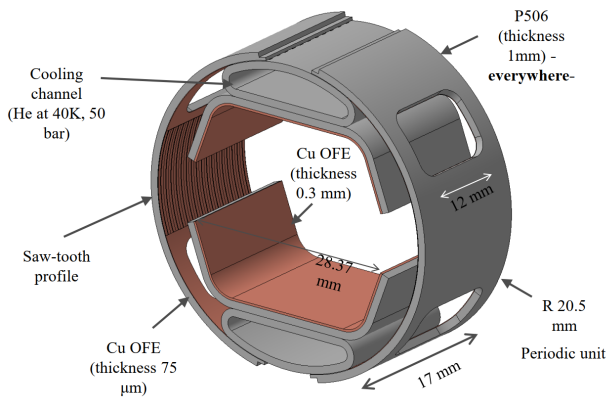
FIG. 31 A periodic unit of the FCC-hh vacuum beam screen, which will be mounted inside the magnet cold bore (1.9 K) (M. Morrone, Update of the design and thermal mechanical study of the FCC-hh beam screen, presented at FCC Week 2019 (Brussels, 26 June 2019)). This beam screen will be operated at an elevated temperature of about 50 K for efficient removal of the heat from synchrotron radiation (Image credit: M. Morrone, CERN).
