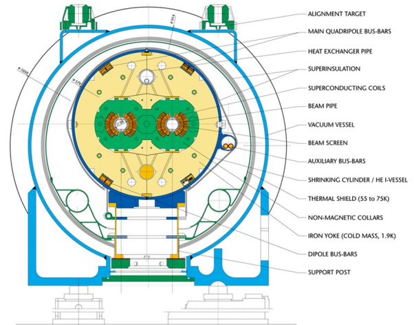
FIG. 4 Cross section of the 14.3 m long superconducting magnet of the Large Hadron Collider (Evans, 2016), The design field of 8.33 T is vertical and opposite in the two 56 mm diameter bores for the two counter-rotating beams, with a horizontal beam-to-beam separation of 194 mm. The LHC comprises 1232 main dipoles, each weighing about 35 tons. (Image CERN, 1999 (CERN-DI-9906025), made available under license CC-BY-4.0, and under permission from ELSEVIER).
