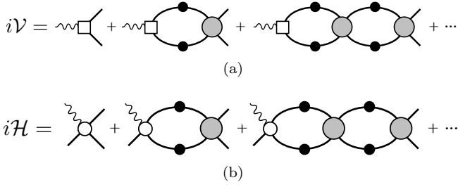
FIG. 21 Shown are the diagrammatic definitions of the (a) 0 \rightarrow 2 and (b) 1 \rightarrow 2 transition amplitudes. The fully dressed propagators and kernels are defined in Fig. 2. The empty squares and circles denote electroweak kernels, which are purely real below multiparticle thresholds.
