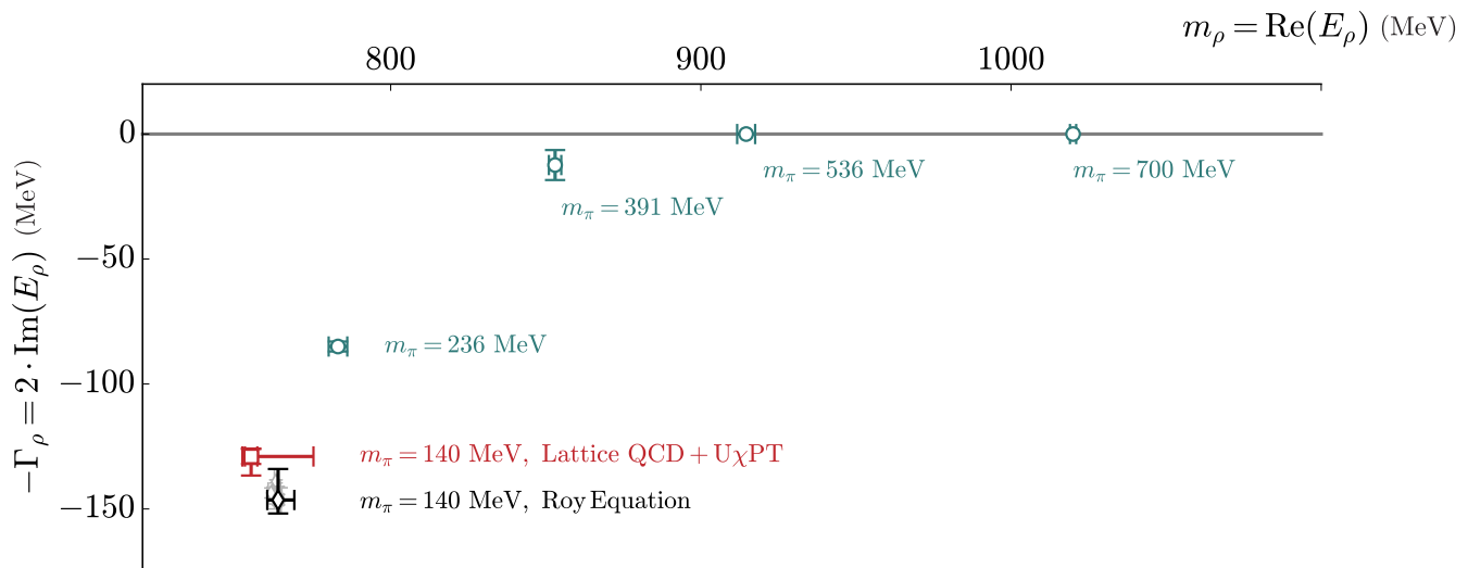
FIG. 1 The pole position of the \rho resonance with varying light-quark mass (expressed in terms of the resulting pion mass) from lattice QCD calculations (blue circles, (Dudek et al. , 2013a,b; Lin et al. , 2009; Wilson et al. , 2015a)) and highly-constrained analysis of experimental data (black diamond, (Ananthanarayan et al. , 2001; Colangelo et al. , 2001; Garcia-Martin et al. , 2011; Masjuan et al. , 2014; Masjuan and Sanz-Cillero, 2013; Zhou et al. , 2005)). Also shown (red square), the result of extrapolating the lattice QCD data down to the physical light quark mass using unitarized chiral perturbation theory (U \chi PT) (Bolton et al. , 2016) (U \chi PT is discussed in Sec. VII.D). A transition from the \rho being a stable bound state to being an unstable resonance is clearly visible.
