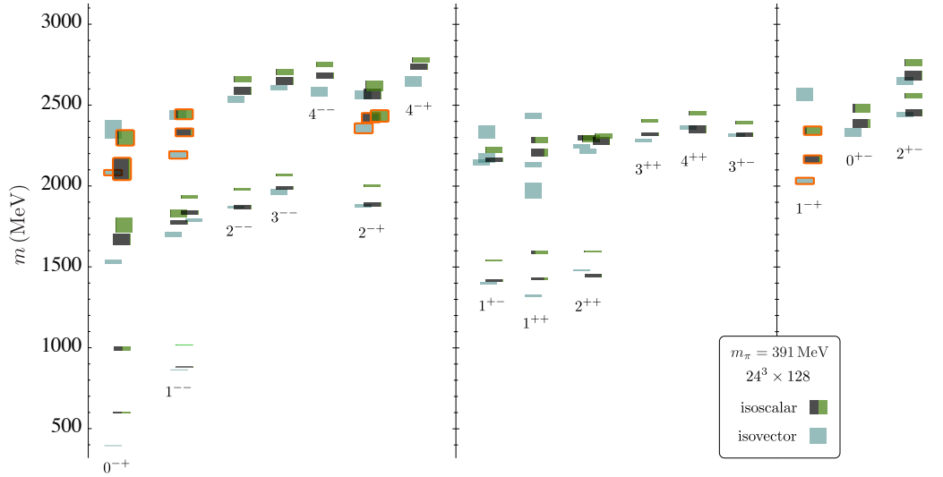
FIG. 8 Spectrum of isoscalar (black/green boxes) and isovector (blue boxes) mesons extracted from variational analysis of large matrices of correlation functions in (Dudek et al. , 2013a). Degree of black/green indicates the hidden light ( u\bar{u} + d\bar{d} ) versus hidden strange ( s\bar{s} ) content of each state determined from relative sizes of operator overlap. Orange outlines indicate lightest set of states having significant overlap with operators featuring a chromomagnetic gluonic construction, suggested to be a signal for them being hybrid mesons .
