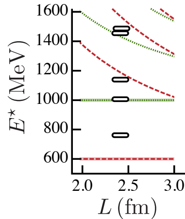
FIG. 20 Rest-frame spectrum in a (2.4 \text{ fm})^3 lattice for the amplitude plotted in Fig. 7.
