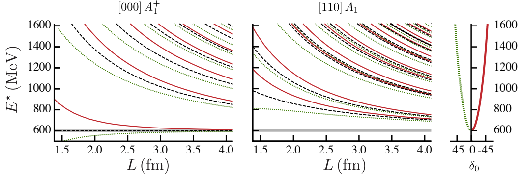
FIG. 4 Finite volume spectrum in a rest-frame irrep and a moving-frame irrep for weak attractive (green dotted lines) and repulsive (solid red lines) elastic scattering. Non-interacting energy levels are indicated by the dashed black lines and the gray band shows the kinematic threshold ( 2m_\pi ). Scattering particles have mass 300 MeV and the scattering length is |a| = 0.32 fm. Rightmost panel shows the corresponding elastic phase-shift in degrees.
