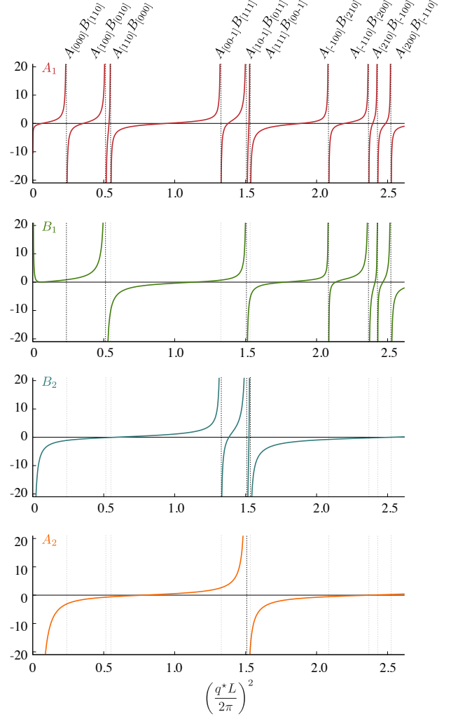
FIG. 25 f_{\ell n; \ell' n'}^A for \mathbf{d} = [110] . From top to bottom: f_{01;01}^{A_1} , f_{11;11}^{B_1} , f_{11;11}^{B_2} , f_{21;21}^{A_2} , which are in each case the lowest \ell subduced into that irrep. The scattering particles ‘A’, ‘B’, are chosen to have masses 300 MeV, 500 MeV, respectively and L is chosen to be 3.6 fm. The divergences can be seen to correspond to the energies of non-interacting AB pairs having momenta of the type shown at the top of the diagram.
