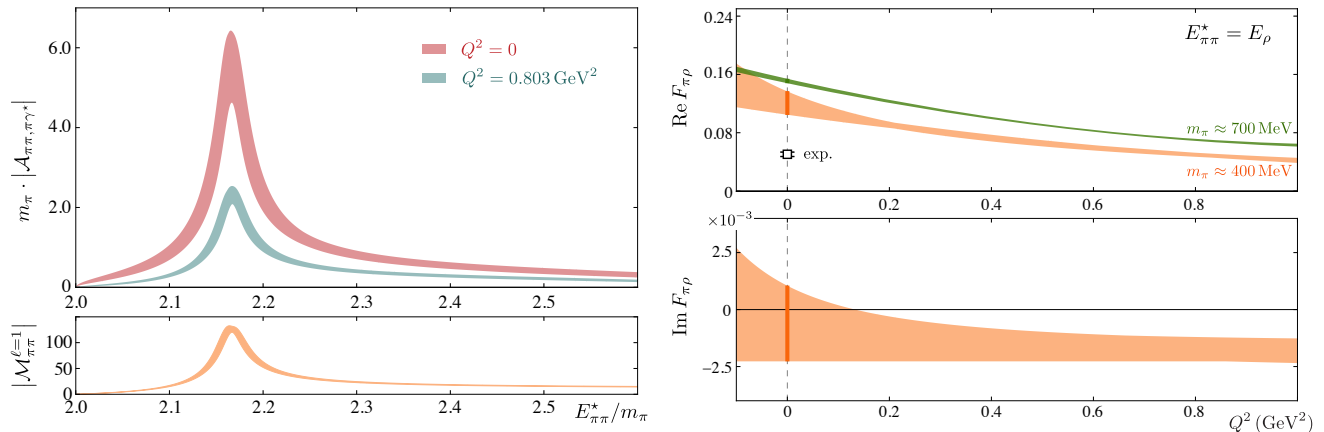
FIG. 24 Left panel: shown is the \pi\gamma^* \rightarrow \pi\pi transition amplitude as a function of the c.m. energy of the system for two values of the photon virtuality obtained (Briceno et al. , 2015a, 2016). This is compared to the elastic \pi\pi scattering amplitude. Right panel: Shown are the real and imaginary components of the \pi \rightarrow \rho form factor obtained for quark masses where the \rho is stable (Shultz et al. , 2015) and when the \rho is unstable (Briceno et al. , 2015a, 2016). This is compared to the experimental photocoupling (Capraro et al. , 1987; Huston et al. , 1986).
