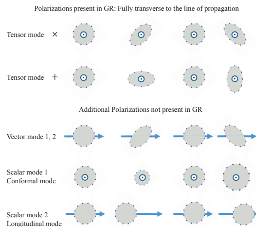
FIG. 1 The six modes for a massive spin-2 field. The two tensor modes and the scalar conformal mode are propagating out of the page; the two vector modes and the longitudinal scalar mode are propagating to the right (taken from (de Rham, 2014)).
