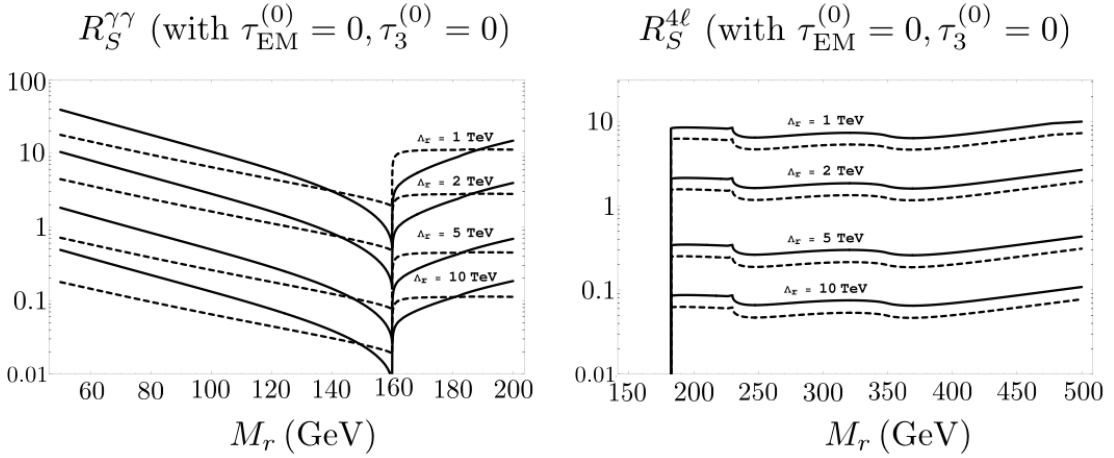
FIG. 15 Ratio of discovery significance for the radion in the realistic RS model (solid), and RS1 model (dashed) to that of a Higgs with the same mass, from (Csáki et al. , 2007).
