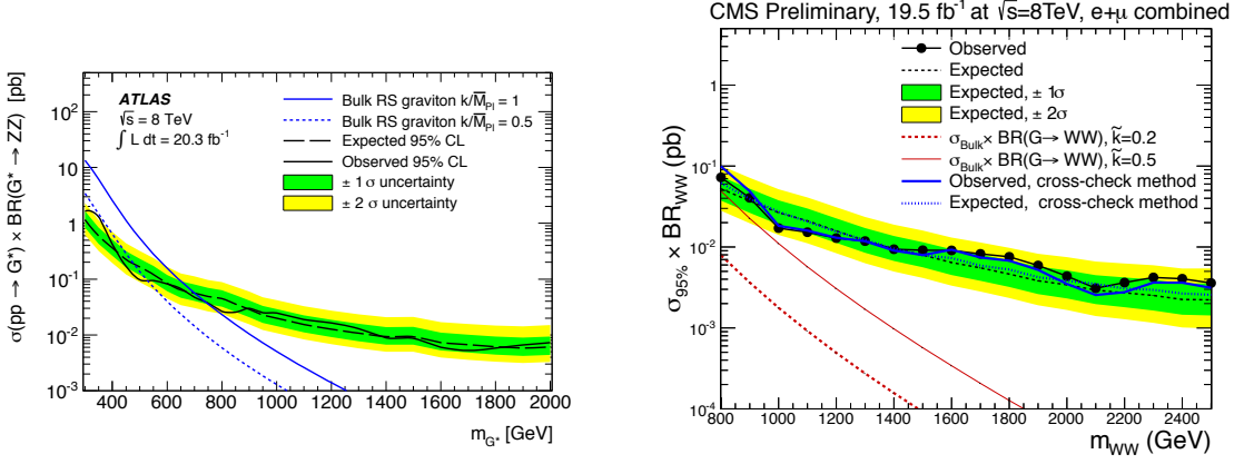
FIG. 14 Bound on KK graviton from the llq\bar{q}lvq\bar{q}' and channel in the “bulk RS” model for different coupling strengths k/\bar{M}_{\text{Pl}} , from (Aad et al. , 2015; Chatrchyan et al. , 2013). Color online.
