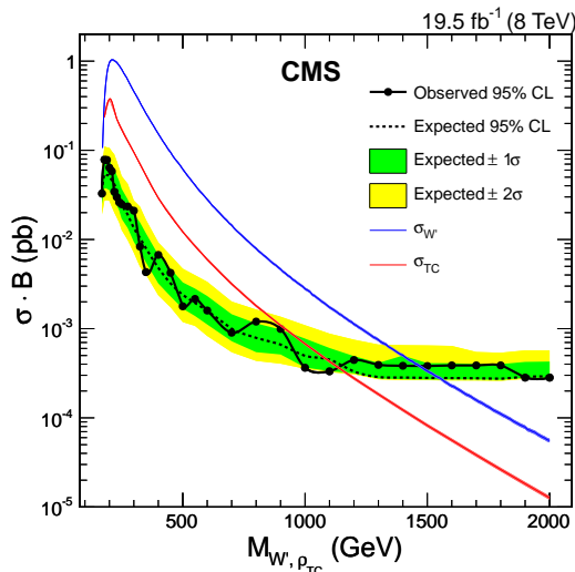
FIG. 19 CMS bound on the W' mass, from (Khachatryan et al. , 2015d). Color online.
