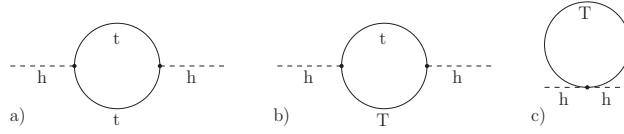
FIG. 23 Cancellation of the quadratic divergences in the top loop for “little” Higgs models, from (Perelstein, 2007).
