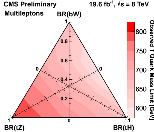
FIG. 30 CMS mass bound on the T-even top partner as a function of branching fractions into bW , tH , tZ , from (Chatrchyan et al. , 2014a). Color online.
