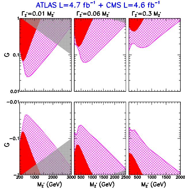
FIG. 20 Model independent bounds on neutral spin-1 resonances in the mass-coupling plane for different Z' widths, from (Gonzalez-Fraile, 2012). Color online.
