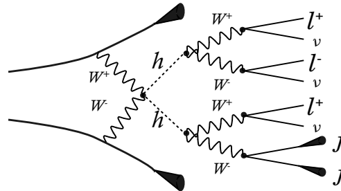
FIG. 33 Difficult 4 W search channel for a pseudo-Goldstone boson Higgs from strong double Higgs production by vector boson fusion, (Contino et al. , 2010).
