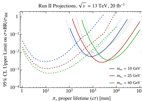
FIG. 35 Expected sensitivity of Run II displaced searches for displaced Higgs decays. The vertical axis is the branching fraction of the Higgs into the displaced decays, while the horizontal is the lifetime of the metastable decay products, for three different values of the mass of these intermediate states, from Csáki et al. (2015). (Color online.)
