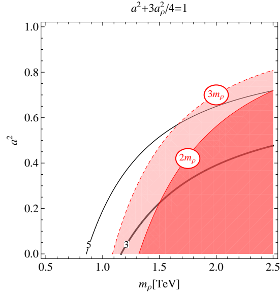
FIG. 22 Higgs and unitarity bounds combined to put an upper bound on the spin-1 resonance, \rho , for different cutoffs \Lambda = 3 \text{ TeV} , 5 \text{ TeV} , 2m_\rho , 3m_\rho , from (Bellazzini et al. , 2012). Here a is the strength of the Higgs coupling to WW relative to the SM. Color online.
