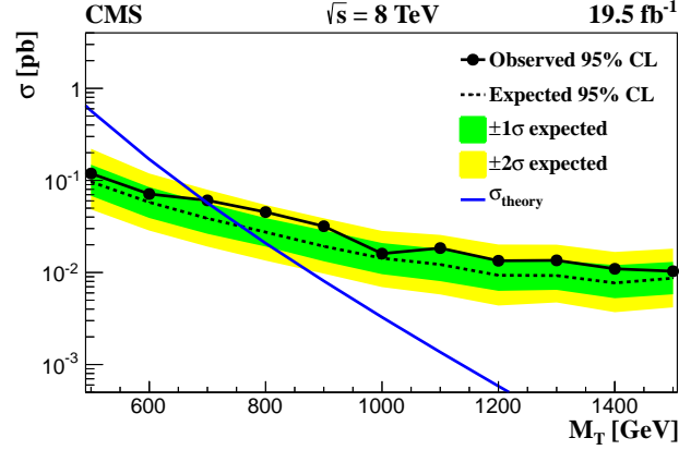
FIG. 29 CMS bound on the T-even top partner production cross section for branching fractions into bW , tH , tZ of 50%, 25%, and 25% respectively, from (Chatrchyan et al. , 2014a). Color online.
