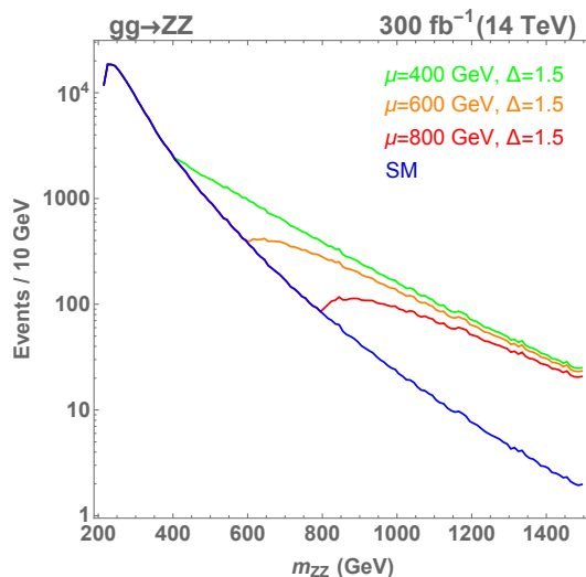
FIG. 37 The effects of a quantum critical Higgs two point function in the production of on-shell Z -boson pairs, with different values of the threshold \mu (Bellazzini et al. , 2015). (Color online.)
