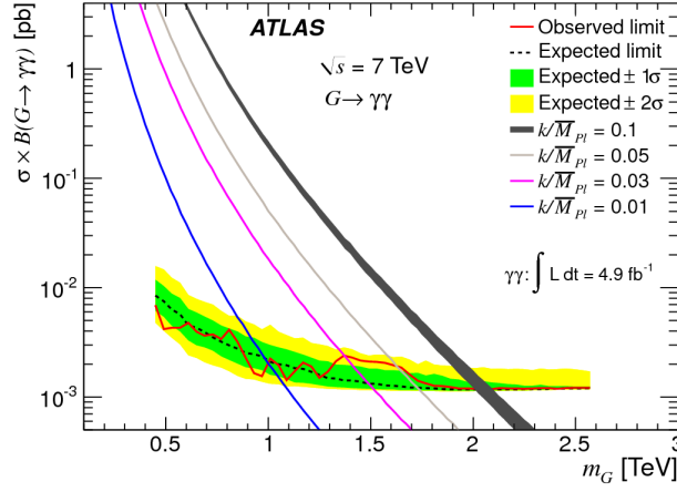
FIG. 13 Bound on KK graviton from the diphoton channel in the RS model for different coupling strengths k/\bar{M}_{Pl} , from (Aad et al. , 2013b). Color online.
