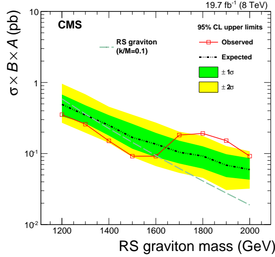
FIG. 12 Bound on the KK graviton from the dijet channel in the RS model, from (Khachatryan et al. , 2015f). Color online.
