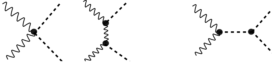
FIG. 32 Double Higgs production in composite pseudo-Goldstone boson Higgs models have contributions that grow with the square of the center-of-mass energy.
