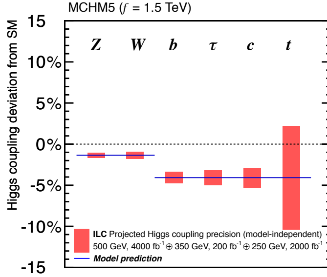
FIG. 31 Examples of deviations from the SM predictions of the Higgs couplings in the minimal composite models (Fujii et al. , 2015). The red bars denote the sensivity of these couplings at the ILC.
