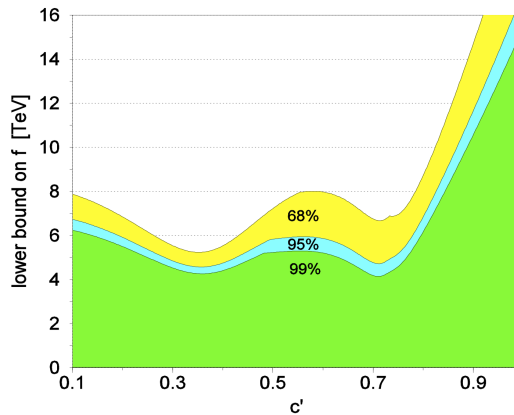
FIG. 25 Lower bound on the “littlest” Higgs scale f , from (Csáki et al. , 2003b).
