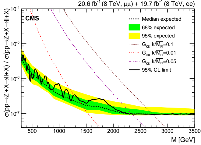
FIG. 11 Bound on the KK graviton from the dilepton channel in the RS model for different coupling strengths k/\bar{M}_{Pl} , from (Khachatryan et al. , 2015e). Color online.
