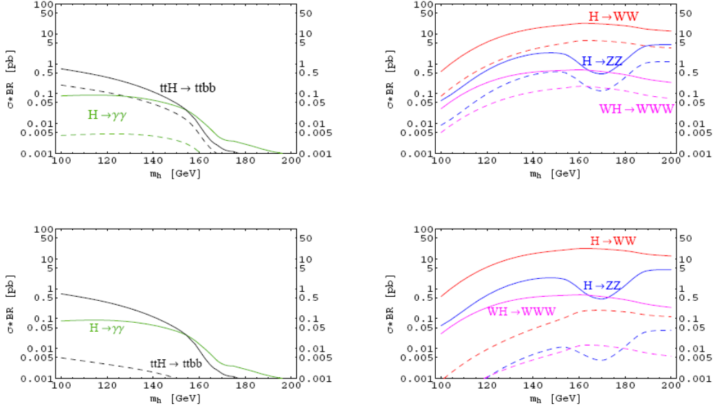
FIG. 17 Cross sections times branching ratios for various Higgs production and decay channels for the SM (solid lines) and bulk Higgs (dashed lines) for \beta = 2 with V = 300 (top) and V = 500 (bottom), from (Cacciapaglia et al. , 2007). Color online.
