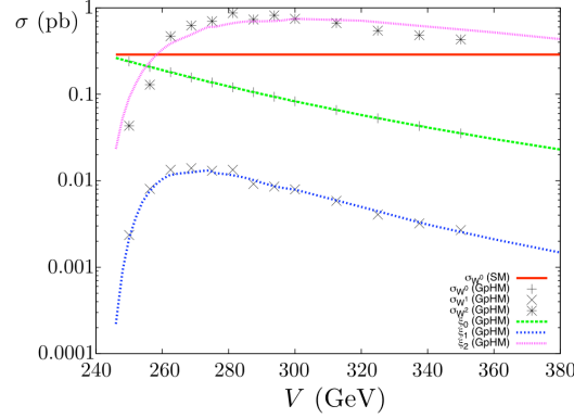
FIG. 21 Approximate contribution to pp \rightarrow WH from an intermediate W' , from (Galloway et al. , 2009a). Color online.
