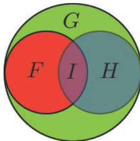
FIG. 26 Coset space for global symmetry group G spontaneously broken to H . If G has a weakly gauged subgroup F then I will be the unbroken gauge group, from (Cheng, 2007). Color online.
