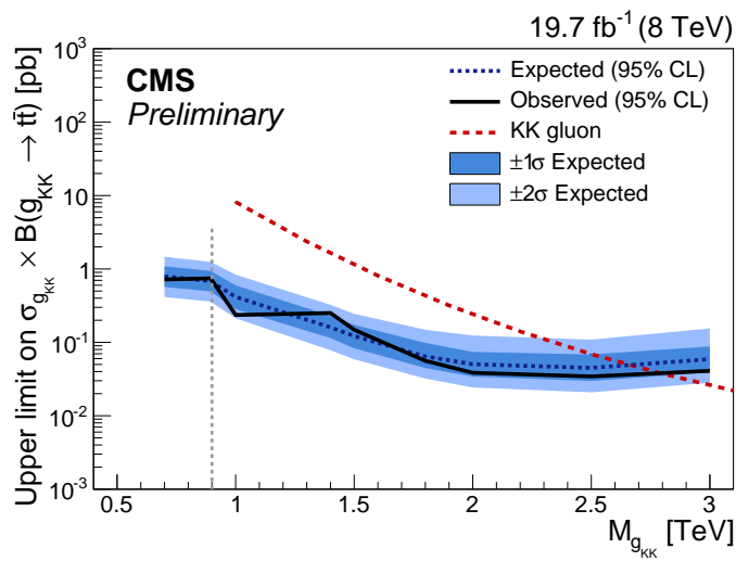
FIG. 7 CMS bound on KK gluon production, from (Khachatryan et al. , 2015a). Color online.
