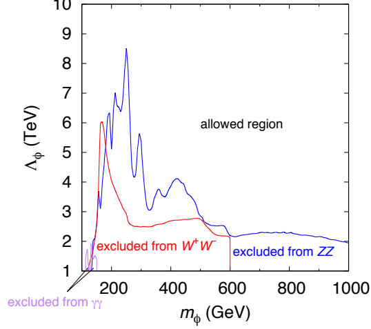
FIG. 16 Bound on the mass of the RS radion ( m_\phi ) as a function of its coupling ( \Lambda_\Phi ), where the coupling is given by \frac{\Phi}{\Lambda_\Phi} T_\mu^\mu , from (Cho et al. , 2013). Color online.
