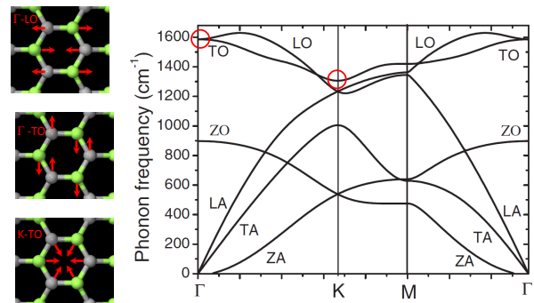
FIG. 7 (color online) DFT calculated phonon dispersion relations for monolayer graphene. The insets on the left show the phonon displacements associated with the optically active LO (top) and TO (middle) phonon modes at the \Gamma point and the K point TO phonon mode (bottom), corresponding to the modes highlighted by red circles. Adapted from Ref. (Yan et al. , 2008).
