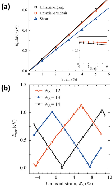
FIG. 12 (color online) Band gap opening E_{gap} as a function of strain for (a) graphene (a) and (b) an armchair nanoribbons. The inset to panel (a) shows the variation of the Poisson ratio \nu along the armchair and zigzag directions. Adapted from Ref. (Li et al. , 2010b).
