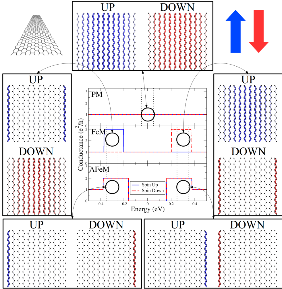
FIG. 36 (color online) Quantum conductance as a function of energy (center) for the PM, FeM, and AFEM states in a 12-ZGNR (full blue curves correspond to spin-up and red dashed lines to spin-down). For each state we present local current plots corresponding to \mu_1 = -0.35 eV and \mu_2 = -0.25 eV and to \mu_1 = +0.25 eV and \mu_2 = +0.35 eV for both the AFEM and FeM states and \mu_{1/2} = \pm -0.05 eV for the PM case (chemical potential windows marked by vertical black dotted lines), both to spin-up (blue) and -down (red) states. Adapted with permission from Ref. (Girão et al. , 2013).
