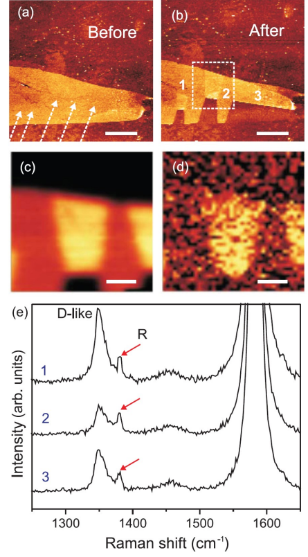
FIG. 27 (color online) (a) Atomic force microscopy image of monolayer graphene sitting on a Si/SiO 2 substrate. The white arrows stand for the directions over which the AFM tip was used in contact mode to scan the graphene sheet and to generate defects. (b) Three regions of folded graphene (labeled 1, 2 and 3) were obtained with the AFM tip. Panels (c) and (d) denote, respectively, the G-band and R-band map intensities for the boxed area in panel (b). (e) Raman spectra of tBLG obtained from the regions 1, 2 and 3 defined in (b). The scale bars are 4 \mu\text{m} (panels (a) and (b)) and 1 \mu\text{m} (panels (c)-(d)). Adapted from Ref. (Carozo et al. , 2013).
