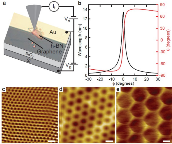
FIG. 30 (color online) (a) Schematic of the measurement setup showing the STM tip and an optical microscope image of a graphene/h-BN heterostructure where the graphene layer is on the top of the h-BN layer. (b) Superlattice wavelength (black) and rotation (red) as a function of the angle \phi between the graphene and h-BN lattices. (c-e) STM topography images for three different Moiré patterns with the wavelength of the periodic potential \lambda = (c) 2.4 nm, (d) 6.0 nm, and (e) 11.5 nm. The white scale bars in all images are 5 nm. Adapted from Ref. (Yankowitz et al. , 2012).
