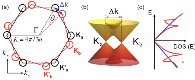
FIG. 24 (color online) (a) Brillouin zone for a twisted bilayer graphene (see Fig. 23) rotated by \theta where the circles represent the iso-energies for Dirac cones from the bottom layer (black) and from the top layer (red). (b) The energy dispersion for each Dirac cone close to the K point and in the vicinity where the two cones overlap, giving rise to van Hove singularities as shown in (c). The two Dirac cones are separated in reciprocal space by \Delta k which depends on \theta , as shown in (a). Adapted from Ref. (Kim et al. , 2012).
