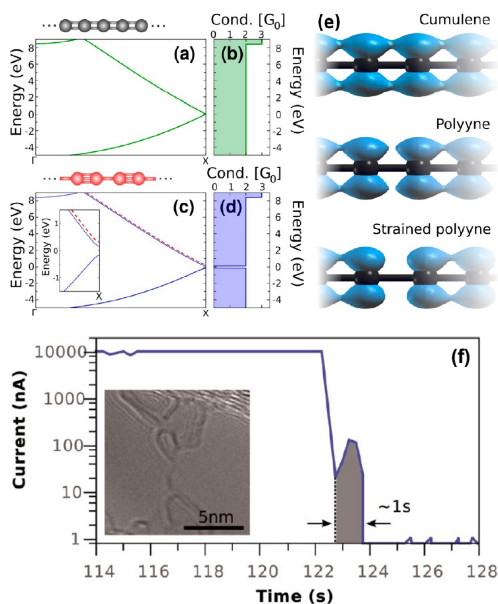
FIG. 41 (color online) (a) and (c) Calculated electronic band structure and (b) and (d) quantum conductance of cumulene and polyynes chains. In (e) the electronic densities for cumulene, polyynes, and strained polyynes chains are shown. (f) Time dependent electrical current measurements made during the formation of a carbon chain. The inset to panel (f) shows the TEM images of the formed chains, just after the sudden drop is observed in the electrical current. Reproduced with permission from Ref. (Cretu et al. , 2013).
