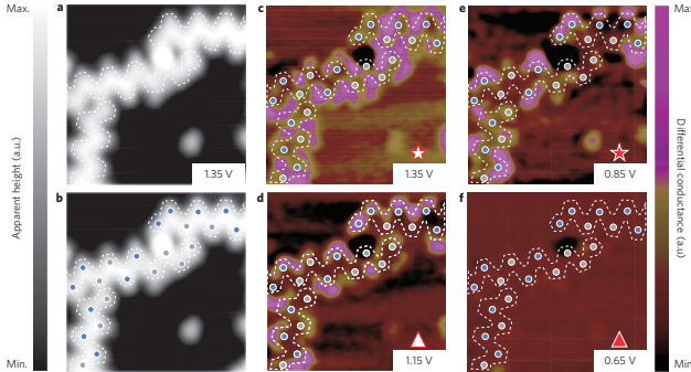
FIG. 38 (color online) Differential conductance maps of an intra-molecular junction between a pristine (p) and nitrogen-doped GNR heterostructures. Heterostructures are artificially outlined by white dashed lines for clarity for the reader. The 10 \times 10 \text{ nm}^2 STM images recorded at T = 5 \text{ K} , U = 1.35 \text{ V} , I = 0.15 \text{ nA} are shown in (a) and (b). In (b), the p- and N-GNR units are indicated by gray and blue dots, respectively. Images (c)–(f) are selected examples of conductance maps at energy positions around the conductance band minimum. The analysis of the results shows that the heterojunction features a type-II alignment with a sharp transition region. Reproduced with permission from (Cai et al. , 2014)
