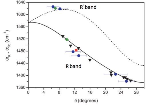
FIG. 29 (color online) R and R'-band frequency ( \omega_R(\theta) and \omega'_R(\theta) ) as a function of the twist angle \theta . The solid circles, square, diamonds and triangles are experimental data from Refs. (Carozo et al. , 2013), (Havener et al. , 2012), (Kim et al. , 2012) and (Wang et al. , 2013a), respectively. Adapted from Ref. (Carozo et al. , 2013).
