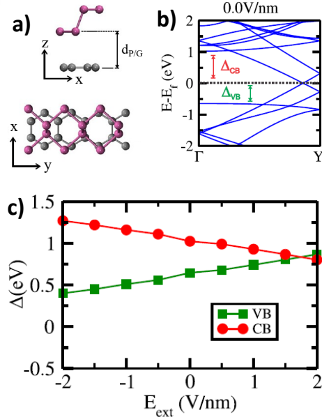
FIG. 31 (color online) (a) Side and top views of a single layer of phosphorene (magenta) on top of graphene (gray), where d_{PG} is the distance between the graphene and phosphorene layers. (b) Band structure of the phosphorene/graphene heterostructure near the Fermi energy. The energy differences between the energy of the graphene Dirac point and the band edges of the phosphorene conduction ( \Delta_{CB} ) and valence ( \Delta_{VB} ) bands are shown as a function of wave-vector from \Gamma to one corner of the Brillouin zone Y . (c) Evolution of the band edges, as a function of the field relative to the graphene Dirac point, for single-layer phosphorene. Adapted from Ref. (Padilha et al. , 2015).
