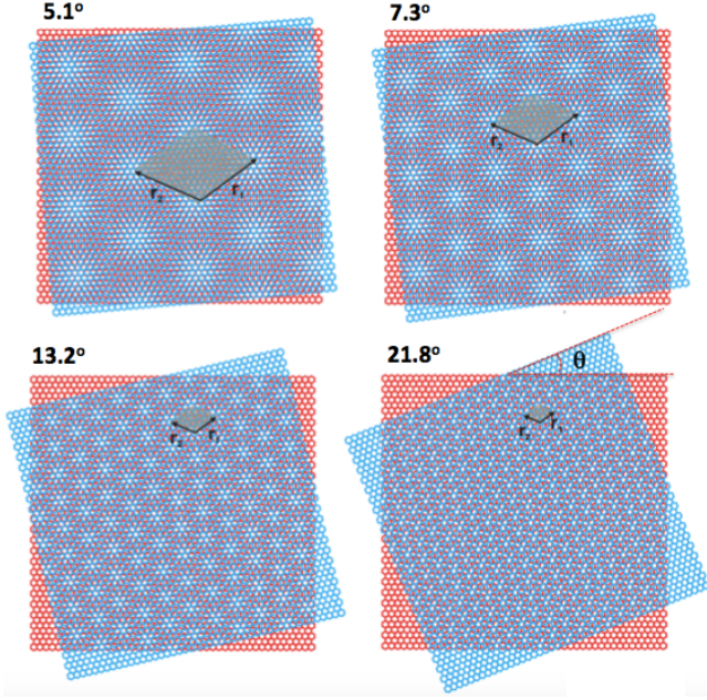
FIG. 23 (color online) Schematic diagram of the Moiré patterns that are formed by twisting bilayer graphene with the twist angles \theta as 5.1^\circ ; 7.3^\circ ; 13.2^\circ and 21.8^\circ . The gray area highlights the unit cell, which decreases as the twisting angle \theta increases. Adapted from Ref. (Carozo et al. , 2013).
