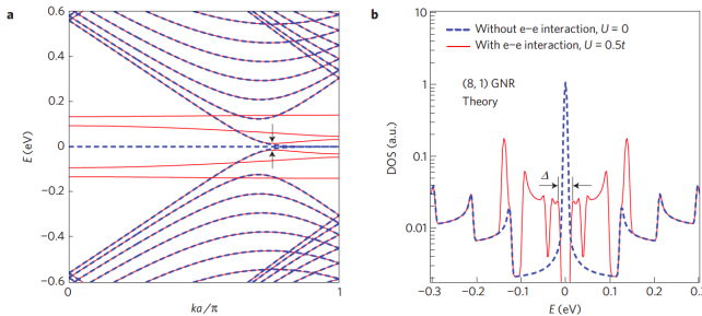
FIG. 18 (color online) (a) Electronic band structure and (b) the corresponding electronic density of states for the (8,1) graphene nanoribbons, calculated using a Hubbard-like model without (blue lines) and with (red lines) electron-electron interaction. The calculated energy splitting of \Delta=29 meV in (b) is comparable to the experimentally observed value of 23.8\pm 3.2 meV. Reproduced with permission from Ref. (Tao et al. , 2011).
