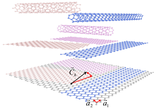
FIG. 2 (color online) Structural models for three carbon nanotubes (top), three graphene nanoribbons (middle), compared to their mother structure graphene (bottom). The chiral vector \vec{C}_h and in-plane vectors \vec{a}_1, \vec{a}_2 are shown.
