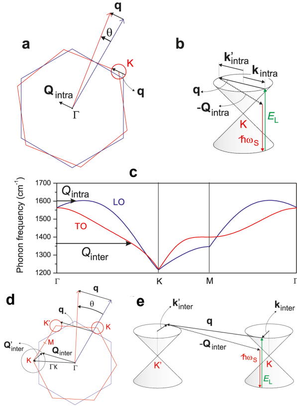
FIG. 28 (color online) (a) Brillouin zones for the top and bottom graphene layers, rotated from each other by a small twist angle \theta . (b) The intra-valley double-resonance process involving elastic electron scattering by the static potential generated by the Moiré pattern. (c) High energy in-plane transverse (TO) and longitudinal (LO) optical phonon branches along high symmetry directions in the 1 st Brillouin zone of graphene (Adapted from Ref. (Venezuela et al. , 2011)). The scattering phonon wave-vectors \mathbf{Q}_{intra} and \mathbf{Q}_{inter} stand for scattering the electron or hole within the same valley and different valleys, respectively. The electron-phonon coupling is stronger for the LO and TO phonon branches near the \Gamma and K points, respectively, and relevant \mathbf{Q}_{intra} and \mathbf{Q}_{inter} wave-vectors are outlined in (d). Adapted from Ref. (Carozo et al. , 2011).
