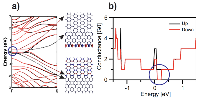
FIG. 39 (color online) (a) Band structure of a hybrid graphene nanoribbon with both zigzag and armchair edges. The arrows point to the wave-function plot of the states around the Fermi energy, displaying the edge state associated with the zigzag edge. The lower arrow points to the junction. (b) Electronic transport plot for this nanoribbon of conductance versus energy, revealing that the nanoribbon can be used as a spin filter on an energy window just above the Fermi energy. Adapted with permission from (Botello-Mendez et al. , 2009).
