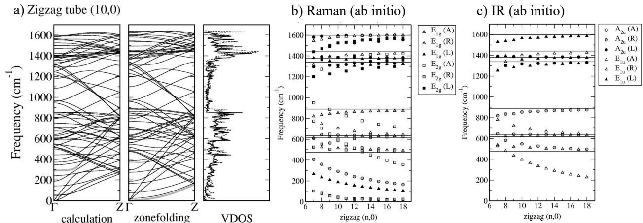
FIG. 8 (a) Phonon dispersion of a (10,0) carbon nanotube obtained by DFT calculations (left panel) and zone folding (middle panel) together with the vibrational density of states (VDOS) for both approaches (right panel), solid and dashed lines are for data obtained with DFT calculations and the zone folding scheme, respectively. Dependence of the frequencies of the (b) Raman active and (c) IR active phonon modes on their n nanotube index for selected (n, 0) zigzag nanotubes. Adapted from Ref. (Dubay and Kresse, 2003).
