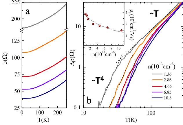
FIG. 32 (color online) Temperature ( T ) dependence of the resistivity \rho(T) for different charge carrier densities in graphene. The measured sample resistivity increases linearly with temperature T in the high temperature limit, thereby indicating that a quasi-classical phonon distribution is responsible for the electron scattering. As T decreases, the resistivity decreases more rapidly, following a T^4 dependence. This low temperature behavior is described by a Bloch-Grüneisen model, taking into account the quantum distribution of the two-dimensional acoustic phonons in graphene, as explained by Fuhrer (Fuhrer, 2010). Reproduced with permission from (Efetov and Kim, 2010).
