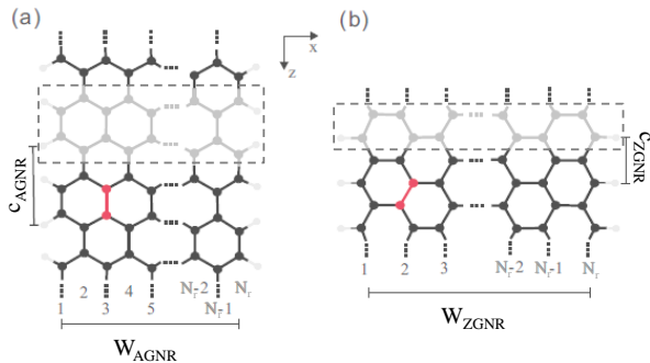
FIG. 3 (color online) Structure of (a) a N-AGNR and (b) a N-ZGNR. In each case, one dimer is highlighted in red. The unit cells are emphasized by a gray box. W_{\text{AGNR}} and W_{\text{ZGNR}} are the armchair and zigzag nanoribbon widths, respectively, while C_{\text{AGNR}} and C_{\text{ZGNR}} show the lengths of the translational vectors for the ribbon unit cells. Adapted from Ref. (Gillen et al., 2009).
