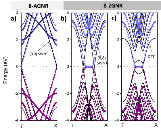
FIG. 6 (color online) (a) Electronic band structure of (a) an armchair edged (8-AGNR) and (b) a zigzag edged graphene nanoribbon (8-ZGNR) calculated using an orthogonal simple tight binding model (symbols) compared to the zone folded bands (solid lines) for the corresponding carbon nanotubes ((9,0) and (8,8), respectively). (c) Comparison between the electronic bands of a 8-ZGNR obtained by tight binding (symbols) and by density function theory calculations (solid line), showing the effects of edges on the electronic energy band structure.
