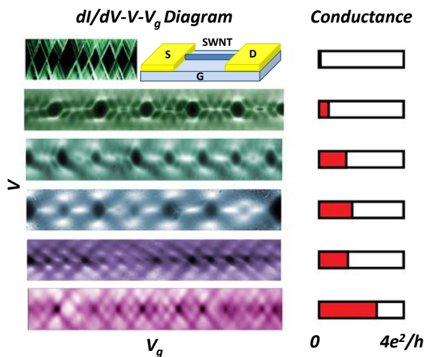
FIG. 34 (color online) Differential conductance dI/dV as a function of gate (G) voltage and source (S) – drain (D) bias. Various quantum transport regimes of a single tube connected to metallic leads are illustrated depending on the coupling strength between the leads and the nanotube conduction channel. The coupling continuously changes from highly reflective (top) to highly transmissive (bottom). The diamond shapes shown on top are typical manifestations of the Coulomb-blockade effect where the addition of one charge to the nanotube corresponds to each diamond. The bottom panel corresponds to a Fabry-Perot-type interference pattern of a one-dimensional standing wave. The amount of conductance in each case is shown on the right. Reproduced with permission from Ref. (Liang et al. , 2005).
