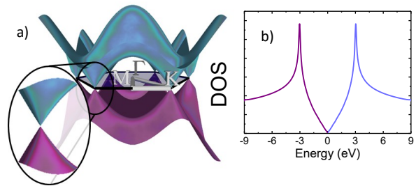
FIG. 4 (color online) (a) Electronic band structure calculated using an orthogonal tight-binding model and only considering nearest neighbor atom interactions. The inset on the lower left highlights the conical energy band dispersion near the Fermi energy. (b) The corresponding energy dependence of the electronic density of states (DOS). For a neutral graphene sample, the Fermi level E_F is located at the Dirac point corresponding to zero energy (Saito et al. , 1992).
