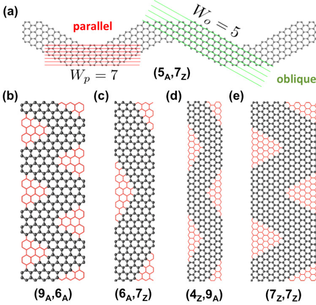
FIG. 21 (color online) (a)-(e) Structural model and nomenclature for graphene nanowiggles, which are made up of successive oblique and parallel cuts in armchair (A) or zigzag (Z) patches. Panel (a) illustrates how the widths of the parallel ( W_p ) and oblique ( W_o ) sectors are defined in terms of number of C-C lines. W_p and W_o refer, respectively, to the number of parallel atomic rows that are present in a nanowiggle in the two indicated directions. Reproduced with permission from Ref. (Costa Girão et al. , 2011).
