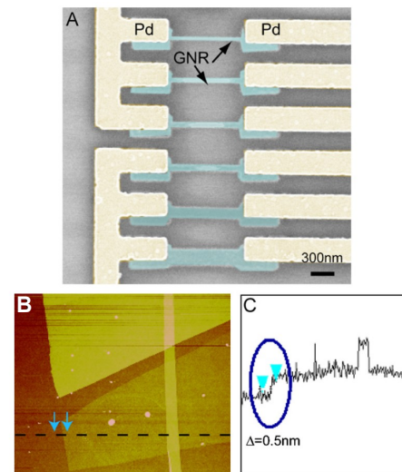
FIG. 35 (color online) (a) SEM micro-graph of GNR devices with various channel widths fabricated on a 200 nm thick \text{SiO}_2 substrate. The widths of the GNRs from top to bottom are 20, 30, 40, 50, 100, and 200 nm. Each GNR was prepared by a lithographic process. (b) AFM image of a single layer graphene sample before lithographic thinning. (c) Cross-section measurement of the AFM along the dashed line shown in (b) indicating that the sheet is a single layer of graphene. Reproduced with permission from (Chen et al. , 2007).
