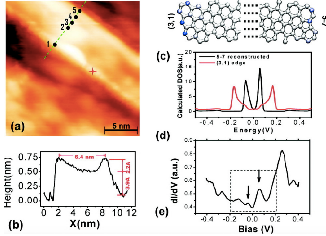
FIG. 19 (color online) (a) STM image and (b) a line profile of height measurements of a CVD-grown 6.4 nm wide nanoribbon. (c) An atomic model is shown for the ribbon with the (3,1) chirality on one edge and a pentagon-heptagon reconstructed edge on the other side. The local density of electronic states is calculated as a function of energy in (d) considering the different edges shown in (c). In (e) the experimental dI/dV measurements measured at the edges of the nanoribbon are shown (see cross + in panel (a)). Reproduced with permission from Ref. (Pan et al. , 2012).
