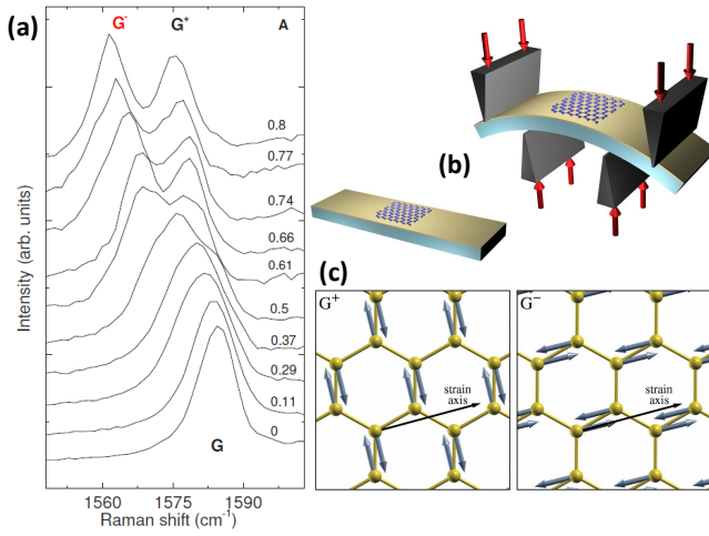
FIG. 14 (color online) (a) G-band evolution as a function of amount of strain applied (numbers on the right side of panel (a)) to a graphene layer immersed in a polymer matrix, as illustrated in panel (b). (c) Eigenvectors for the G^- and G^+ modes obtained by DFT based-calculations in strained graphene. Adapted from Ref. (Mohiuddin et al. , 2009).
