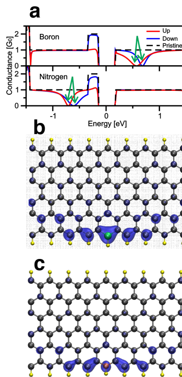
FIG. 40 (color online) (a) DFT calculated electronic transport of boron and nitrogen doped graphene nanoribbons. Green arrows indicate the energy of the calculated donor-like (boron) and the acceptor-like (nitrogen) states. Local density of states (LDOS) plots for (b) nitrogen and (c) boron localized states at the energies indicated by the arrows on the plot (a). Adapted with permission from (Cruz-Silva et al. , 2011a)
