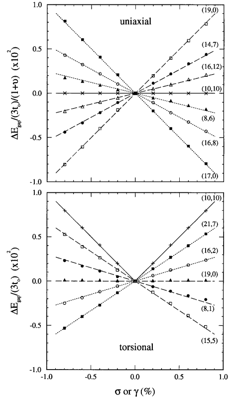
FIG. 15 Effects of uniaxial and torsional strain on the band gap of several (n, m) nanotubes. Lines are for the analytical model and points are simulation data using the tight-binding method. Adapted from Ref. (Yang and Han, 2000).
