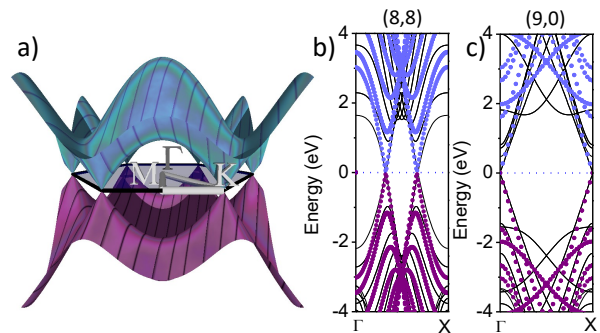
FIG. 5 (color online) (a) Electronic band structure of graphene showing the cutting lines corresponding to nanotube's allowed states in black. Electronic band structure of (b) an (8,8) armchair and (c) a (9,0) zigzag carbon nanotube obtained both from zone folding (solid circles) and ab initio calculations (solid lines).
