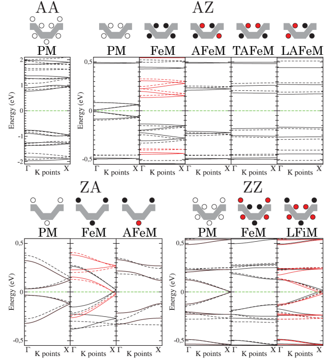
FIG. 22 (color online) Electronic band structures calculated by using DFT (dashed lines) and tight-binding (solid lines) methods corresponding to the different magnetic states for the representative AA, AZ, ZA and ZZ graphene nanowiggles, shown in Fig. 21(b)-(e). The schematic spin distributions (red: down, black: up) are shown on top of each panel. Reproduced with permission from Ref. (Costa Girão et al. , 2011).
