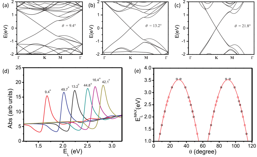
FIG. 25 (color online) (a)-(c) Electronic band structure for twisted bilayer graphene for three distinct twist angles \theta ( 9.4^\circ , 13.2^\circ , and 21.8^\circ , respectively) taken over the range of energy -2.0 eV to +2.0 eV. (d) Calculated optical absorption spectra near the absorption peak as a function of twist angle \theta . (e) \theta dependence for the optical absorption peaks at E_L^{max} , according to the results calculated in panel(d), and others not shown. Squares denote calculated data and circles are values replicated by symmetry. The solid line is a fit to the equation E_L^{max} = E_0 |\sin(3\theta)| . Adapted from Ref. (Carozo et al. , 2013).
