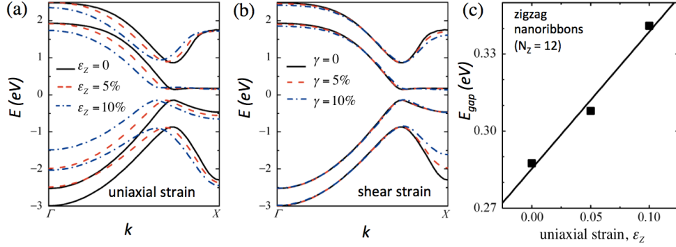
FIG. 13 (color online) Electronic band structure considering spin polarization effects for a zigzag nanoribbon as a function of uniaxial (a) and shear (b) strain. (c) Band gap opening as a function of strain for the band structure shown in (a). Adapted from Ref. (Li et al. , 2010b).
