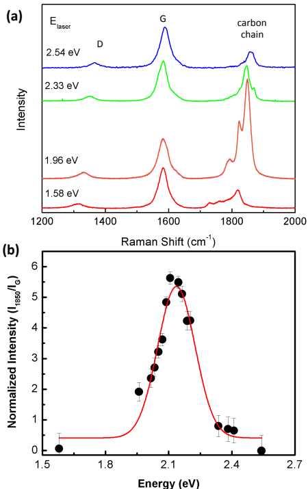
FIG. 42 (color online) (a) Resonance Raman spectra of linear carbon chains encapsulated in multi-wall carbon nanotubes. The D- and G-band Raman modes from carbon nanotubes are here shown along with the bands from the chain. (b) Resonance window of the linear carbon chain mode. Reproduced with permission from Refs. (Andrade et al. , 2015a,b).
