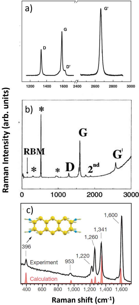
FIG. 9 (color online) Raman spectra of (a) graphene, (b) an isolated single-wall carbon nanotube, and (c) a N_r=7 AGNR. Adapted from (Malard et al., 2009b), (Jorio et al., 2001) and (Cai et al., 2010).
