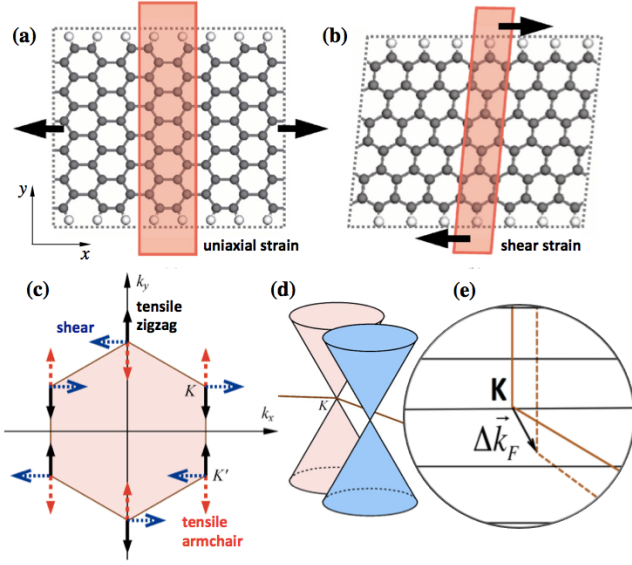
FIG. 11 (color online) (a) A uniaxial and (b) shear strain applied to graphene nanoribbons in real space. The red shaded rectangles denote the unit cell of the strained structures. In panel (c), the displacement of the K point in reciprocal space due to the tensile strain (along the armchair and zigzag directions) and the shear strain is shown. The effect of strain is to displace the Dirac cone from the K point to another position of the Brillouin zone (panel d). In panel (e), the allowed states for low-dimensional nanostructures, such as nanoribbons and nanotubes, are illustrated by the cutting lines. The effect of strain on those structures can be interpreted based on the displacement of the Fermi points by a vector \Delta\mathbf{k}_F . Adapted from Ref. (Li et al. , 2010b).
