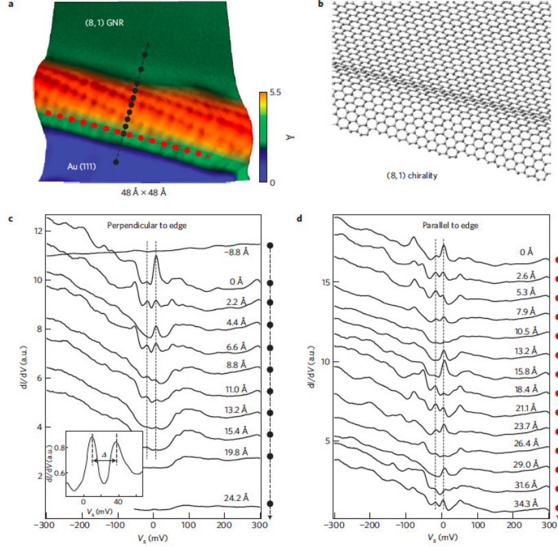
FIG. 17 (color online) Scanning tunneling microscopy (STM) measurements on graphene nanoribbons obtained by unzipping carbon nanotubes. (a) STM topographical image ( V_s=0.3 V, I = 60 pA, T=7 K) of the edge of an (8,1) graphene nanoribbon over an Au(111) surface and (b) its corresponding structural model. STS measurements of the graphene nanoribbon measured along a line (c) perpendicular (black points) and (d) parallel (red points) to the ribbon edge. The inset to panel (c) shows a high-resolution dI/dV spectrum for another nanoribbon with a (5,2) geometry, thus showing the energy-splitting \Delta of the edge states. Reproduced with permission from Ref. (Tao et al. , 2011).
