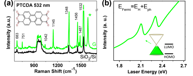
FIG. 10 (color online) (a) Raman spectra of 5 Å PTCDA on graphene (colored line) and on a blank \text{SiO}_2/\text{Si} substrate (black line) with a 532 nm excitation laser wavelength ( E_{\text{laser}} = 2.33 eV). The inset shows the structure of the PTCDA molecule. Reproduced with permission from Ref. (Huang et al., 2015). (b) Calculated Raman intensity as a function of laser excitation energy for E_F = E_H + \hbar\omega_q . A homogeneous broadening of \gamma = 0.03 eV is considered. Adapted from (Barros and Dresselhaus, 2014).
