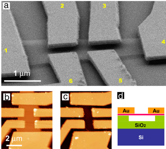
FIG. 33 (color online) (a) Off-side view of a scanning electron microscopy (SEM) image using a suspended six-probe graphene device. (b) Atomic Force Microscopy image of the suspended device before the measurements, and (c) after the measurements with graphene removed by a short oxygen plasma etch. (d) Side view of the device (schematic). The doped silicon gate, partly etched \text{SiO}_2 , suspended single-layer graphene and Au/Cr electrodes are shown, respectively, in blue, green, pink, and orange. The white rectangle denotes vacuum. Reproduced with permission from Ref. (Bolotin et al. , 2008b).
