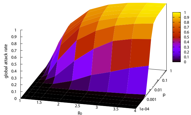
FIG. 12 (color online) Global threshold in a heterogeneous metapopulation system. The left panel shows a 3D surface representing the value of the final epidemic size in the metapopulation system as a function of the local threshold R_0 and of the diffusion probability p . If R_0 approaches the threshold, larger values of the diffusion probability p need to be considered in order to observe a global outbreak in the metapopulation system. Figure adapted from Colizza & Vespignani, 2007.
