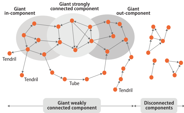
FIG. 4 (color online) Component structure of a directed graph. Figure adapted from Dorogovtsev et al. (2001).
