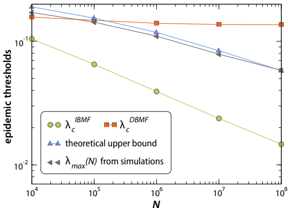
FIG. 6 (color online) Numerical thresholds for the SIS model as a function of the network size N in power-law distributed networks with degree exponent \gamma = 3.5 , computed from the average lifetime method proposed by Boguñá et al. (2013). Numerical data are compared with different theoretical approaches as well as with the the upper bound obtained from the DBMF theory with long range dynamical correlations, developed by Boguñá et al. (2013). Figure adapted from Boguñá et al. (2013).
