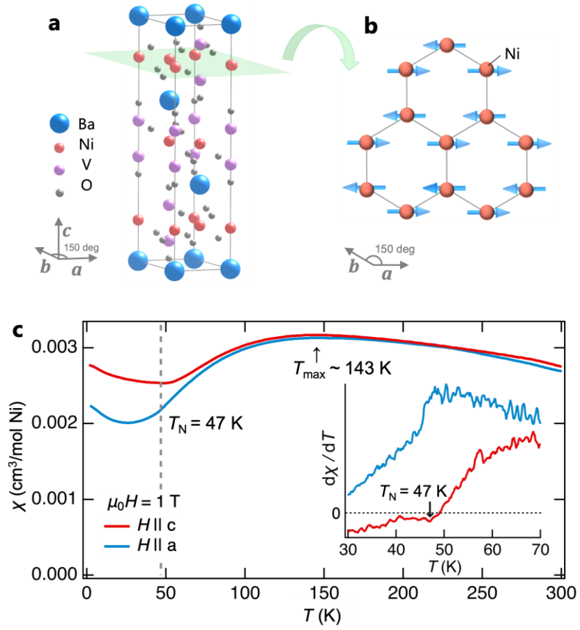
Fig. 1 (a) Crystal structure of \text{BaNi}_2\text{V}_2\text{O}_8 . (b) Magnetic structure of a \text{Ni}^{2+} honeycomb plane. Each magnetic moment lies approximately in the honeycomb plane. (c) Temperature dependence of magnetic susceptibility \chi at 1 T. The inset shows temperature dependence of \frac{d\chi}{dT} and the definition of T_N .
