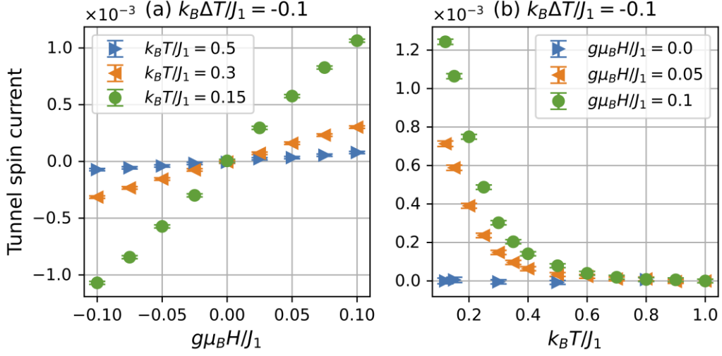
Fig. 4 (a) Magnetic-field and (b) temperature dependences of numerically calculated tunnel spin currents in the bilayer model of a 2D antiferromagnet ( 10 \times 10 size) and a metal. Results of larger size systems also exhibit the same H and T dependences as the above panels (a) and (b) (see SM [45]). The temperature difference \Delta T is defined as \Delta T = T_{\text{metal}} - T_{\text{magnet}} , where T_{\text{metal}} and T_{\text{magnet}} are respectively the temperatures of the metal and the antiferromagnet. Here, g\mu_B H = \frac{e\hbar}{m}\mu_0 H . If we set J_1 \simeq 12.3 meV \simeq 143 K following Ref. [41], k_B T/J_1 = 0.15 , 0.3, and 0.5 respectively correspond to k_B T \simeq 21 , 43, and 72 K. In addition, a magnetic field regime |g\mu_B H|/J_1 < 0.1 corresponds to |H| < 10.5 T. The BKT transition point has been evaluated as k_B T_{\text{BKT}} \sim 0.3 J_1 at g\mu_B H/J_1 \rightarrow 0 [41]. From previous studies of Refs. [31,32], k_B T_{\text{BKT}} is expected to be around 0.2 J_1 < k_B T_{\text{BKT}} < 0.4 J_1 in a weak-field regime |g\mu_B H|/J_1 < 0.1 . The error bars indicate the confidence range of 99.73%.
