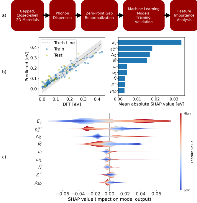
FIG. 2. a) ML workflow. b) ERT train and test set accuracy and feature-dependent SHAP values averaged over all materials. The \sim 95\% confidence interval is shown in the shaded region, represented as two times the standard deviation of the residual error. The value for this interval is 60 meV. c) Violin plot of feature-dependent SHAP values per material. The SHAP value in b) can be interpreted as the average contribution of each feature to the final ZPR, while the violin plot displays the contribution for each material and illustrates (anti) correlation of the feature with ZPR.
