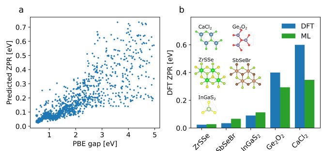
FIG. 3. a) Predicted ZPR as a function of DFT-PBE bandgap for 1302 materials from the C2DB database. b) Comparison of ML and DFT-predicted ZPR five randomly selected materials studied.
