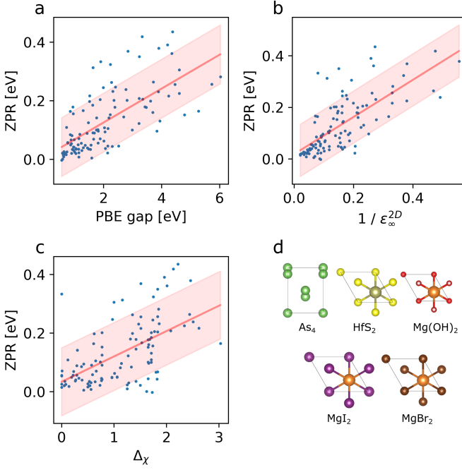
FIG. 1. Dependence of the ZPR on (a) DFT-PBE gap, (b) in-plane electronic dielectric constant, and (c) ionicity. Linear fit to the data is shown via a red line with two times the standard deviation of the residual error associated shown in the shaded region. The slope of the fitted line is 0.06, 0.72, and 0.09 for a), b), and c), respectively. (d) Atomistic geometries of a few representative systems in the training database as shown in Table I.
