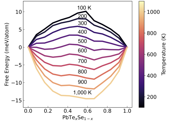
FIG. 9. The \Delta G_{mix} of \text{PbSe}_{1-x}\text{Te}_x gradually becomes more concave with increasing temperature, reaching full convexity at 700 K (within a tolerance of 2\sigma_{\bar{H},n} ). Here, the alloy compositions are sampled at 1/12 increments.
