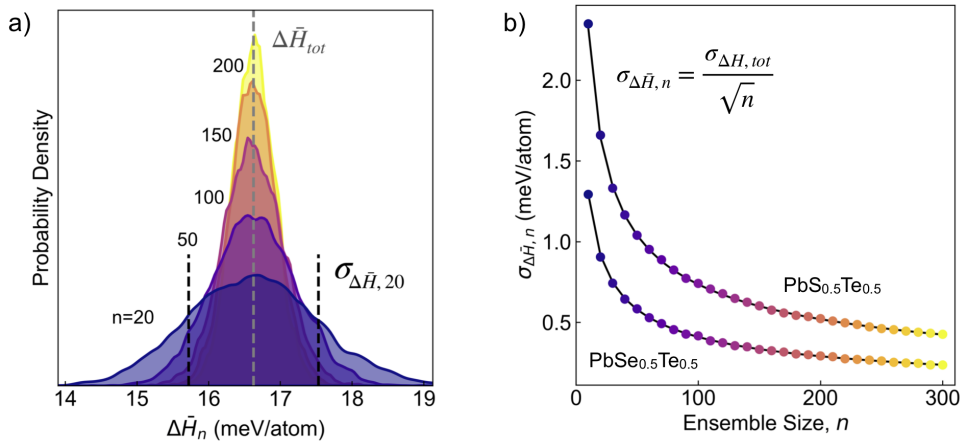
FIG. 4. To illustrate the CLT, we start with the composition \text{PbSe}_{0.5}\text{Te}_{0.5} and highlight in (a) that the distribution of \Delta\bar{H}_n values for any given n forms a Gaussian centered around the true value, \Delta\bar{H}_{tot} . The standard deviation of each Gaussian, \sigma_{\Delta\bar{H},n} , decreases with increasing n . Each Gaussian arises from calculating \Delta\bar{H}_n of 10,000 ensembles. Each point in (b) is determined by taking the standard deviation in \Delta\bar{H} from 10,000 ensembles, including the Gaussians in (a). In (b), this decrease in \sigma_{\Delta\bar{H},n} can be modeled using the central limit theorem (black line). By simply knowing the ensemble size and \sigma_{\Delta H,tot} , \sigma_{\Delta\bar{H},n} can be determined. The procedure is repeated for \text{PbS}_{0.5}\text{Te}_{0.5} to illustrate the importance of chemical composition. Since \sigma_{H,tot} is larger, \text{PbS}_{0.5}\text{Te}_{0.5} requires more configurations to reach the same level of uncertainty.
