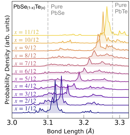
FIG. 10. Bond length distributions in \text{PbSe}_{1-x}\text{Te}_x smear as we move towards x -values of 6/12 , highlighting the increased structural disorder in these alloys. The peak of each distribution corresponds well to Vegard’s law. All distributions are shown in the high-temperature limit, and are generated from 50 configurations.
