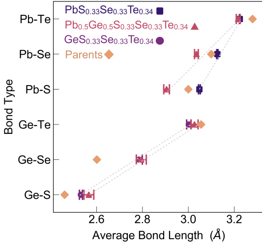
FIG. 13. Local distortion resulting in alloy bond lengths deviating from their parent bond lengths. Further complications arise when mixing parent compounds with different structures. Average bond lengths, broken up by type, are shown for various compositions. The bars denote the standard deviation in the bond lengths for a given type and composition. For reference, the parent bond lengths are included as well. We are invoking the high-temperature limit by taking simple averages. All averages are generated from 50 configurations.
