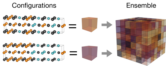
FIG. 1. Alloys are represented as an ensemble of configurational states within the Independent Cell Approximation. Post hoc application of statistical mechanics then predicts the alloy’s local structure, thermodynamic stability and material properties.
