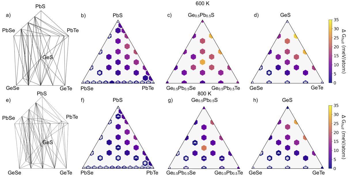
FIG. 12. (a) The (\text{Pb}_{1-x}\text{Ge}_x)(\text{Te}_y\text{Se}_z\text{S}_{1-y-z}) phase space is visualized as a prism with cation composition varying along the axis. Pseudo-ternaries (b-d) show three slices of this prism with discrete sampling; the color scheme denotes the free energy above the convex hull. Hexagons with a silver point inside indicate that they are on the hull; hexagons with a triangle denote compositions whose distance from the hull is less than their uncertainty ( 2\sigma_{\bar{E},n} , as determined by the CLT). Calculating the convex hull at 600 K using the coarse sampling of (b-d) fills the interior of the prism with four-phase tetrahedra. At this temperature, the x=0.5 compositions are not on the hull and the resulting tetrahedra of (a) span from x=0 to x=1 compositions. (e-h) The lower row shows the results at 700 K. At this temperature, far more compositions are on the hull, including in the interior of the prism (g), where many of the compositions exhibit significant entropy stabilization.
