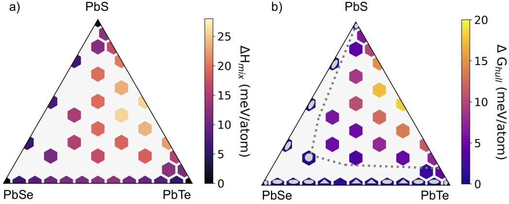
FIG. 11. (a) The calculated enthalpy of mixing ( \Delta H_{mix} ) for the \text{PbS}_x\text{Se}_y\text{Te}_{1-x-y} space is shown. \Delta H_{mix} is particularly high for PbS-PbTe-rich compositions. (b) The free energy above the convex hull ( \Delta G_{hull} ) finds that compositions rich in both PbS and PbTe are at energies above the hull. They are thus subject to decomposition to PbS and PbTe alloys. Grey circles denote being on the hull, and grey triangles signify being that the composition is on the hull within the uncertainty from random sampling (ie. \Delta G_{hull} < 2\sigma_{\Delta H} ). The simulated results are corroborated by experimental findings, although there is a temperature offset. Both \Delta H_{mix} and \Delta G_{hull} were calculated at 600 K. The grey dashed line is an experimental result showing the region of immiscibility at 773 K [52].
