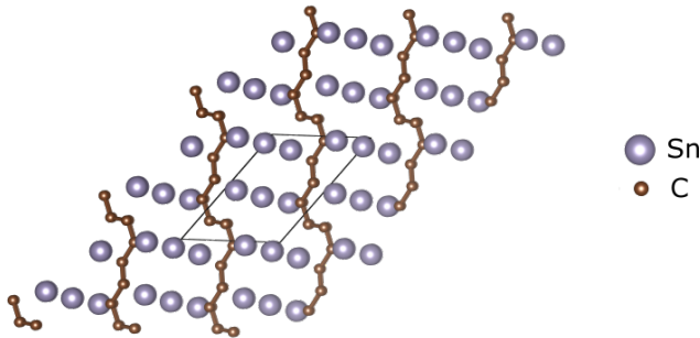
FIG. 5. The most probable structure of SnC. The Sn layers which include atoms coordinated only to other Sn atoms and the thin C layers clearly indicated that this structure has phase separated to the degree possible within a twelve-atom cell. This structure has a positive enthalpy of formation of 1.36 eV/formula unit.
