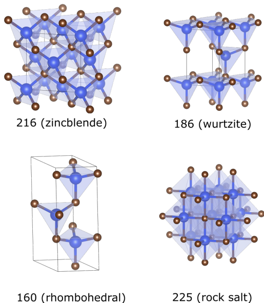
FIG. 1. The 4 known structure types of SiC, zincblende (s.g. #216 or 3C), wurtzite (s.g. #186 or 2H), rhombohedral (s.g. #160 or 9R), and rocksalt (s.g. #225). The numbers in the labels for the H and R structures denote the number of formula units in the conventional unit cell (may be less in the primitive cell).
