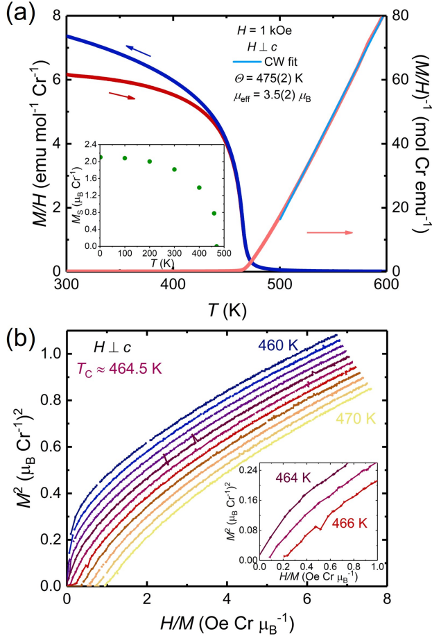
Figure 3: (a) Temperature dependence of M/H (left axis) and (M/H)^{-1} (right axis). The light blue line marks the Curie-Weiss fit to the data above 500 K. The inset shows the spontaneous magnetization ( M_s ) estimated from the M(H) data as a function of temperature. (b) Arrot plots between 460–470 K. The inset shows a closeup of the data between 464–466 K.
