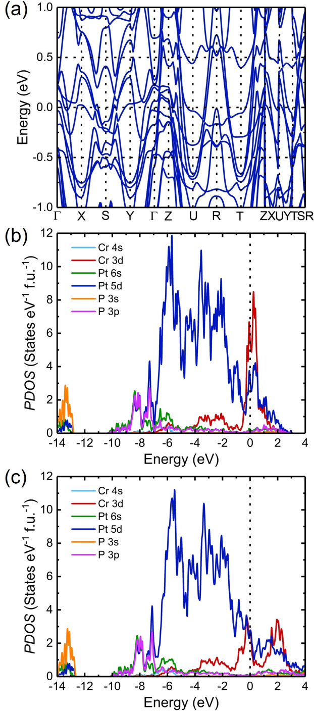
Figure 5: (a) Electronic band structure for \text{CrPt}_5\text{P} in the ferromagnetic phase (with moments along the a -axis). (b) Density of states in the non-magnetic phase. (c) Density of states in the ferromagnetic phase. The calculations assume the ideal 1-5-1 composition (no Cr-Pt site disorder)
