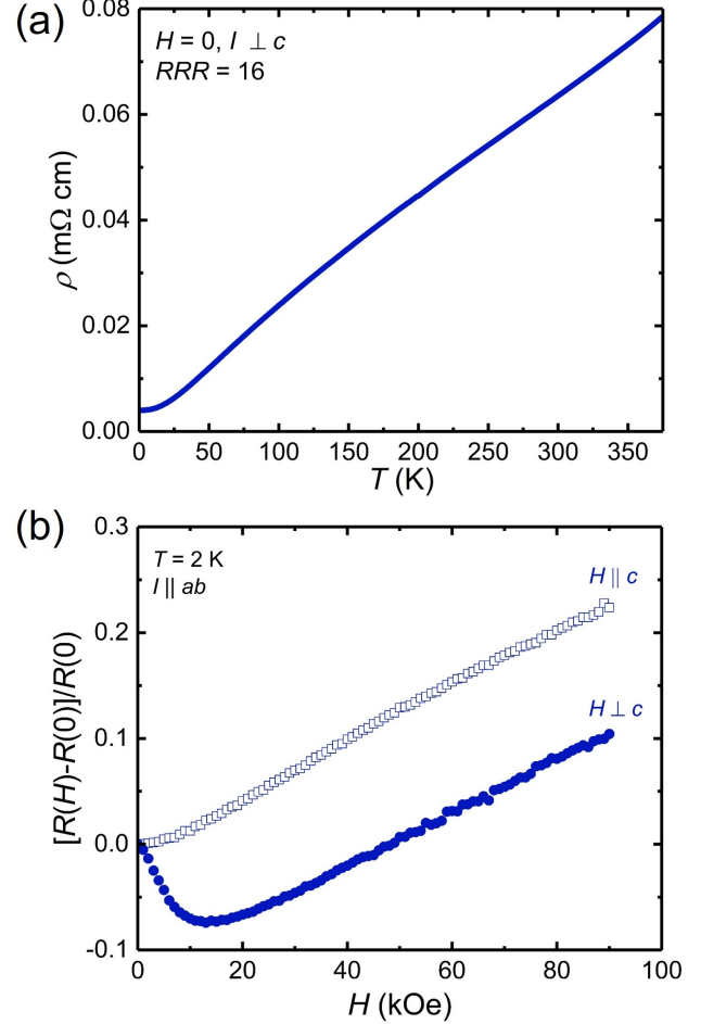
Figure 4: (a) Temperature dependent resistance of \text{CrPt}_5\text{P} between 1.8–375 K. (b) Transverse magnetoresistance at 2 K.
