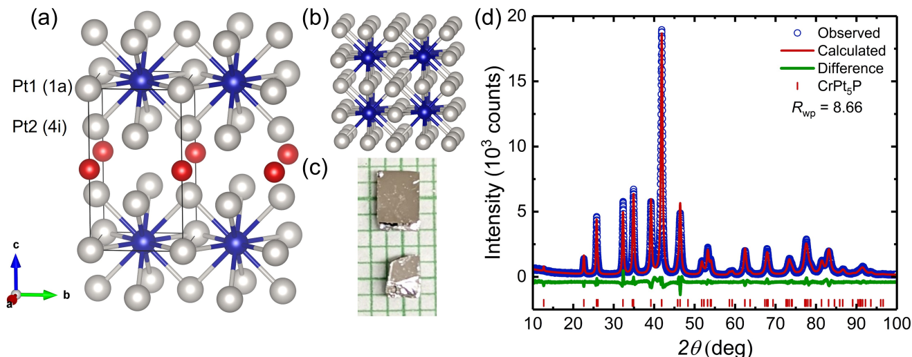
Figure 1: (a) Crystal structure of (a) \text{CrPt}_5\text{P} and (b) \text{CrPt}_3 . The color code is blue = Cr, grey = Pt, and red = P. (c) Pictures of several \text{CrPt}_5\text{P} single crystals on a mm grid. (d) Powder X-ray diffraction pattern and Le Bail refinement for \text{CrPt}_5\text{P} .
