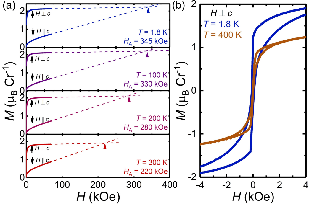
Figure 2: (a) Field dependent magnetization isotherms at temperatures between 1.8–300 K. The solid points are the data and the dashed lines are extrapolations to estimate the anisotropy fields. (b) Full magnetization isotherms in the easy direction ( H \perp c ) at 1.8 K and 400 K showing hysteresis when raising/lowering the field.
