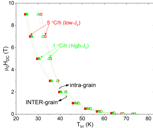
FIG. 8 Irreversibility lines of the low and high- J_c Bi-2212 wires estimated for both the intra-grain and the INTER-grain contribution to the dissipation.
