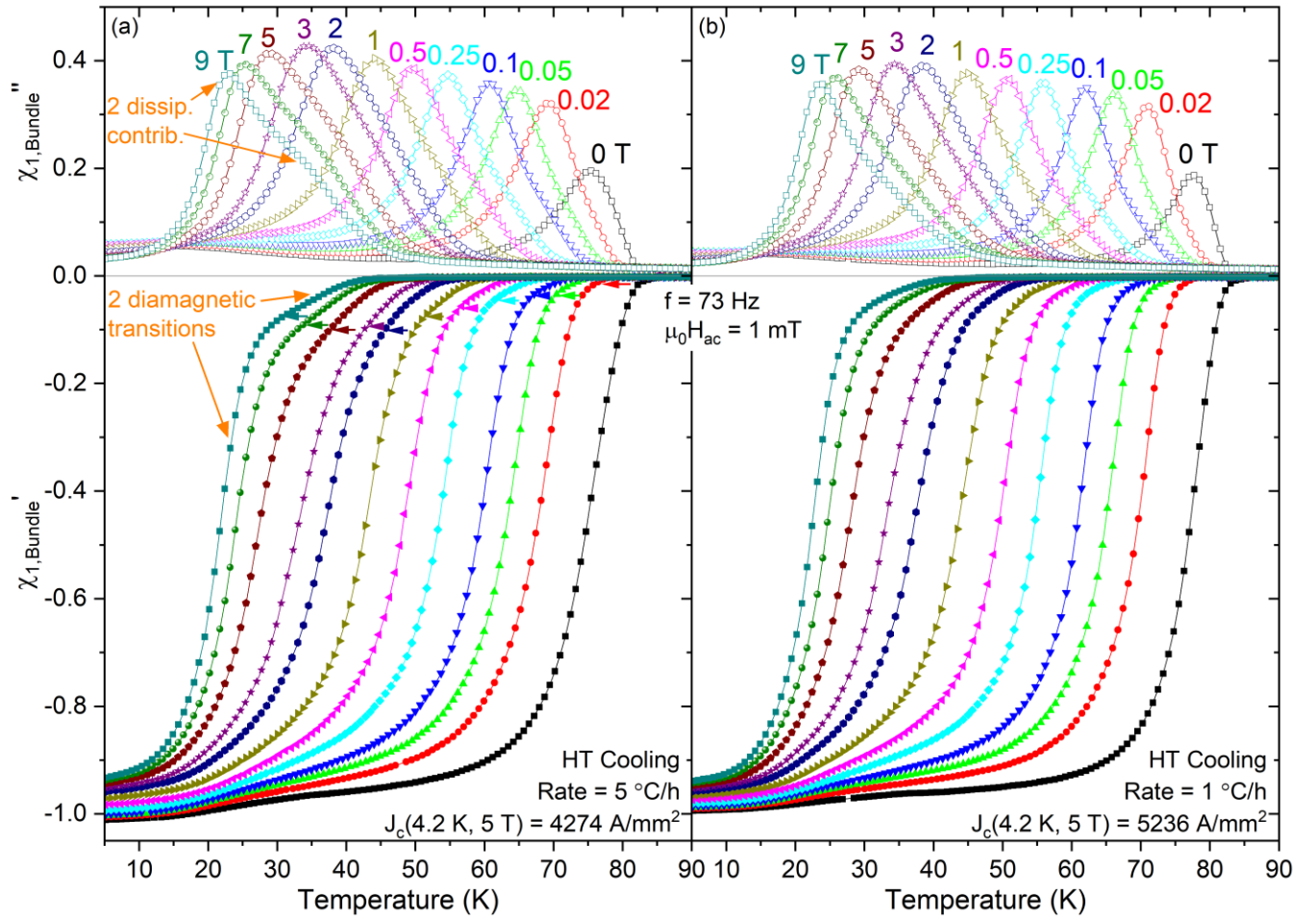
FIG. 5 Temperature dependence of the AC susceptibility (evaluated on the bundle-scale) of the (a) low- J_c and (b) high- J_c Bi-2212 1.2 mm wires, measured with different DC-fields for H \perp wire. In (a) the 2 diamagnetic transitions and two dissipation contributions are highlighted for the 9 T data; the small arrows next to the \chi'_1 curves indicate the approximate locations of the INTER-grain onset. The higher-temperature diamagnetic transition and dissipation contribution are slightly less evident in the high- J_c wire.
