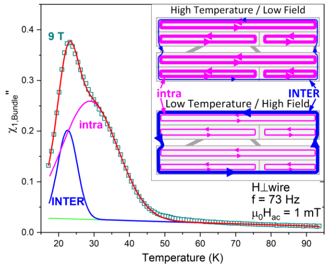
FIG. 6 Temperature dependence of \chi_1'' (evaluated on the bundle-scale) for a Bi-2212 wire ( 5^\circ\text{C/h} ) measured at \mu_0 H_{DC} = 9 T, fitted with a 2-Gaussian curve. The insets represent the changes in the intra-/INTER-grain relative currents, induced into the grains (sketched as small rectangles) and into the bundles (sketched as bridged filaments), as field and temperature are changed.
