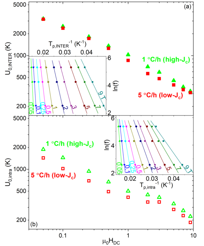
FIG. 10 DC field dependence of the pinning energies, U_0 , for the (a) INTER- and (b) intra-grain contributions of the low and high- J_c 2212 wires, estimated from the \mu_0 H_{ac} = 1 mT data. In the insets, the INTER- and intra-grain Arrhenius plots of a Bi-2212 wire.
