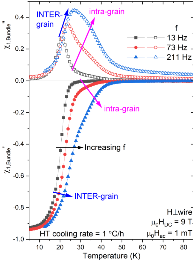
FIG. 9 Temperature dependence of the AC susceptibility (evaluated on the bundle-scale) of a Bi-2212 wire, measured at different frequencies, showing the weak variation on the features associated to the INTER-grain contribution and a stronger change in the intra-grain properties.
