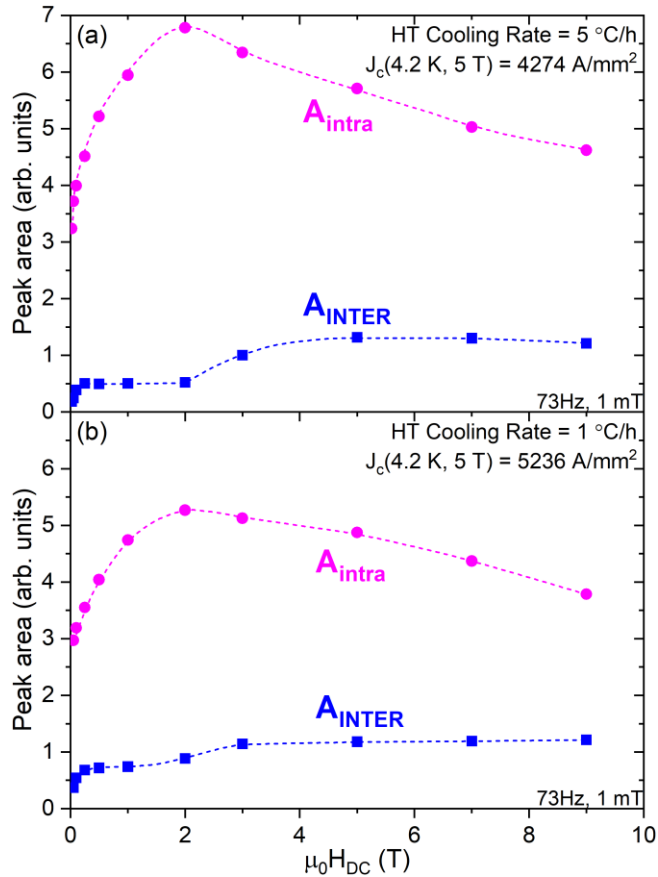
FIG. 7 Peak areas of the intra- and INTER-grain contributions as a function of H_{DC} for the (a) low- and (b) high- J_c 1.2 mm Bi-2212 wires
