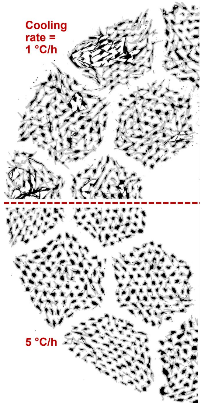
FIG. 1 Threshold images of the Bi-2212 phase; shown are \frac{1}{4} of the Bi-2212 wire cross-sections (1.2 mm-diameter) after heat treatments with different cooling rates at 1 (top) and 5 °C/h (bottom). The perimeters of discrete elements in the cross-section are colored grey to highlight the different filament bridging behavior.
