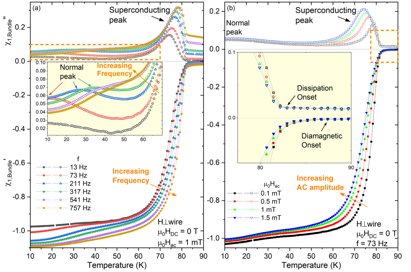
FIG. 3 Temperature dependence of the AC susceptibility of a Bi-2212 wire ( 5^\circ\text{C/h} ) for H \perp wire, evaluated using the bundle rather than filament-scale (see text), measured at different (a) frequencies and (b) AC amplitudes at zero DC field. The real, \chi'_{1,Bundle} , and imaginary, \chi''_{1,Bundle} , parts are plotted. The inset in (a) highlights the rapid shift toward high temperature of the normal eddy-current peak with increasing frequency. The inset in (b) highlights the difference between the dissipative and the diamagnetic onsets.
