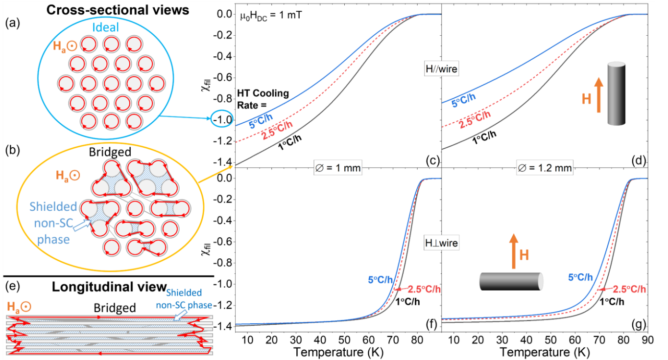
FIG. 2 (a)-(b) 2D schematics (not to scale) of shielding in a multifilamentary Bi-2212 conductor, for H//wire, in the ideal (a) and the bridged (b) cases showing filaments (circles), bridges (straight lines joining the filaments) and the shielding currents (paths with arrows); in (b), striped regions between filaments represent a non-superconducting phase shielded by supercurrent percolating through the bridges. These simplified sketches explain how |\chi_{fil}| can exceed 1. (c)-(d) Temperature dependence of \chi , estimated from the filament sizes, for magnetic field applied along the wire axis showing an apparently unphysical trend (see text for explanation); data for the 1 and 1.2 mm-diam. wires heat treated with different cooling rates are shown. (e) 2D schematic (not to scale, similarly to (b)) of shielding in a bridged multifilamentary Bi-2212 conductor for H \perp wire. (f)-(g) Data as in panels (c)-(d), but for magnetic field perpendicular to the wires.
