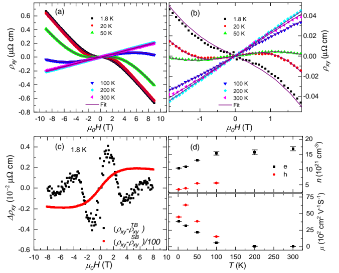
FIG. 6. Hall effect measurements on TbV 6 Sn 6 . (a) Hall resistivity, \rho_{xy} , as a function of magnetic field, measured at different temperatures. To remove mixing of transverse resistivity, \rho_{xy} is isolated as \rho_{xy} = (\rho_{xy}(H) - \rho_{xy}(-H))/2 . Fits to a two-band model below 100 K and single band model above 200 K are represented by solid lines through the data. (b) \rho_{xy} at low field at various temperatures focusing on the deviation of model at 1.8 K. (c) The anomalous Hall signal and non-linear Hall resistivity, \Delta\rho_{xy} , at 1.8 K, where the calculated resistivity using two-band (TB) and single-band (SB) models based on the linear region at high fields was subtracted to calculate \Delta\rho_{xy} . (d) Upper panel shows the temperature dependence of electron-type and hole-type carrier densities, n , obtained by the fits to the Hall data. Lower panel shows the temperature dependence of the charge carrier mobilities, \mu for each carrier type obtained from fits to the Hall data.
