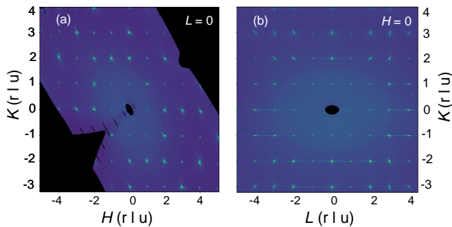
FIG. 2. Synchrotron X-ray diffraction data. (a) Bragg reflections in the (H, K, 0) scattering plane. (b) Bragg reflections in the (0, K, L) scattering plane. Axis units are plotted in r.l.u.
