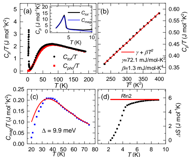
FIG. 7. Heat capacity, C_p(T) , measurements in TbV 6 Sn 6 . (a) Temperature dependence of total ( C_{tot}/T ) and phonon ( C_{pho}/T ) heat capacity observed at zero-magnetic field. The inset of (a) represents total ( C_{tot} ) and magnetic ( C_{mag} ) heat capacity around T_C . C_p(T) displays a sharp \lambda -like anomaly at 4.1 K. (b) Temperature dependence of C_p/T plotted as a function of T^2 . Solid red color line shows the fit to the Sommerfeld form C_p(T) = \gamma T + \beta T^3 in paramagnetic region above T_C . (c) Magnetic contribution to the heat capacity, C_{mag}/T , in the temperature range of 20-75 K. Solid line is a fit to a two-level Schottky anomaly as described in the text. (d) Magnetic entropy change, \Delta S , at low temperature below 9 K. The red color line represents the calculated entropy for an effective spin 1/2 system.
