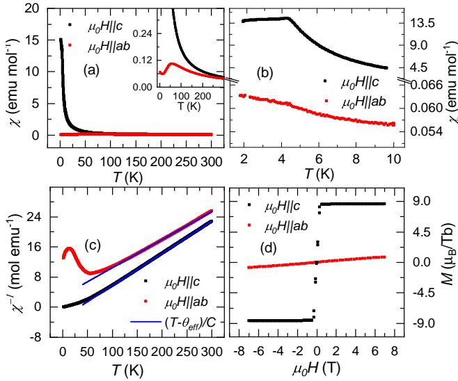
FIG. 3. Magnetic properties of \text{TbV}_6\text{Sn}_6 . Red and black squares represent the data measured with the applied field parallel and perpendicular to the (001) crystal surface. (a) Temperature dependent magnetic susceptibility, \chi , at an applied field of 100 mT. The inset of (a) displays a broad anomaly around 60 K in \chi along the (001) crystal surface. (b) Magnetic susceptibility below 10 K measured with a field of 10 mT. (c) Inverse magnetic susceptibility at an applied magnetic field of 100 mT. (d) Field dependent isothermal magnetization at 1.8 K.
