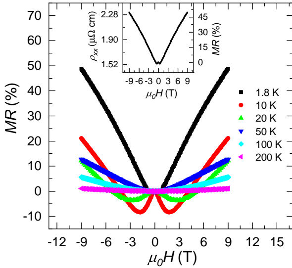
FIG. 5. Transverse magnetoresistance data. Isothermal magnetoresistance ratio (MR) increases with the decrease in temperature and it exhibits a minima at low temperature due to the coupling with the spin polarization. The inset shows the magnetoresistance data at 1.8 K. The isothermal \rho_{xx}(H) data exhibits weak asymmetry upon reversed field direction due to contamination from the Hall signal. The magnetoresistance component was isolated by averaging \rho_{xx}(H) and \rho_{xx}(-H) . At high fields, \rho_{xx} displays linear field dependence.
