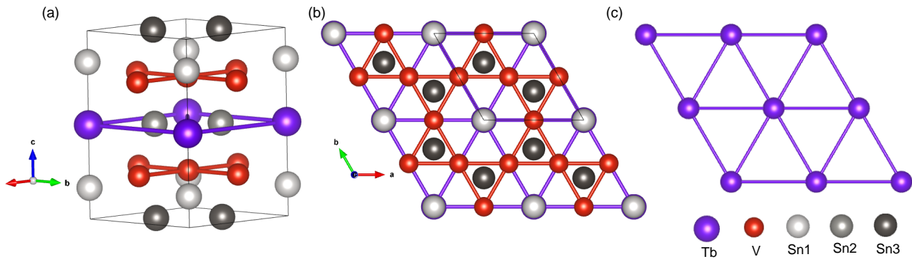
FIG. 1. Crystal structure of \text{TbV}_6\text{Sn}_6 . (a) A unit cell formed by the arrangements of Tb, V and Sn atoms. Sn atoms occupying the three different crystallographic sites are depicted by light black, medium black and dark black color spheres. (b) Top view of crystal structure, viewed along c-axis, showing the kagome layer of V-atoms and projected Sn1 and Sn3 sites. (c) Triangular lattice of Tb-ions interwoven between the kagome planes of V-ions.
