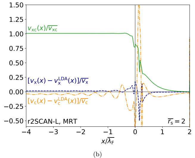
FIG. 8. The exchange and correlation potential in an \bar{r}_s = 2 jellium surface, evaluated on the same LSDA densities used previously. The present OFR2 (RPP) (top, 8a) and r 2 SCAN-L (MRT) [66] (bottom, 8b) LL-MGGA potentials are shown. The same finite difference coefficients as in Fig. 7 were used to generate these plots. As before, the edge of the uniform positive background lies at x = 0 , and x is scaled by the bulk Fermi wavelength, \bar{\lambda}_F = 2\pi/k_F . The potential is scaled by the corresponding LSDA potential evaluated at the bulk density.
