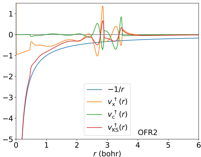
FIG. 7. OFR2 Kohn-Sham potential calculated using Eq. (33) for the up-spin channel, evaluated on the exact density, n(r) = n_\uparrow(r) = e^{-2r}/\pi ( v_{xc}^\uparrow = 0 identically for this system). A 6 th order finite difference was used to calculate the requisite divergence and Laplacian terms. Oscillations are primarily due to inclusion of the density-Laplacian.
