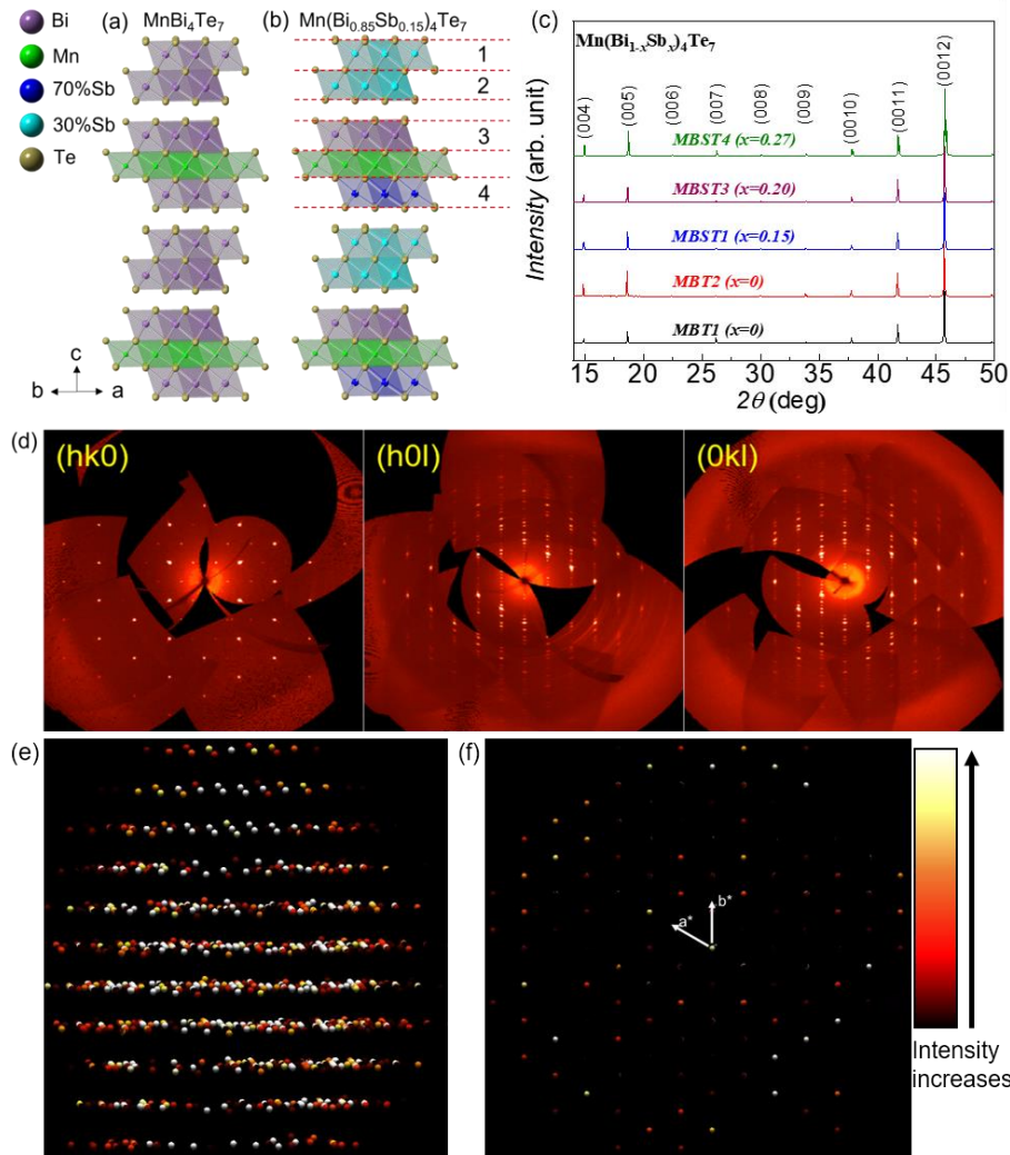
Fig. 1. Schematic crystal structures of pristine MnBi 4 Te 7 (a) and Mn(Bi 0.85 Sb 0.15 ) 4 Te 7 (b). Mn(Bi 0.85 Sb 0.15 ) 4 Te 7 shows preferential Sb occupations at different Bi sites on layers labeled by 1, 2, 3, and 4. (c) X-ray diffraction patterns of samples MBT1, MBT2, MBST1, MBST3, and MBST4. (d) Single-crystal X-ray diffraction patterns obtained on the (hk0), (h0l), and (0kl) planes. (e) Reflection intensity map in the reciprocal space, projected along a zone-axis slightly away from c*. (f) The intensity map along the c*-axis.
