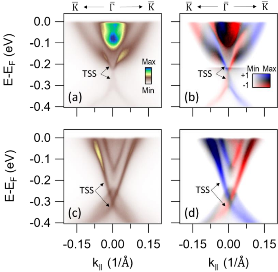
Fig 7. Electronic structures for two terminations of \text{Mn}(\text{Bi}_{0.85}\text{Sb}_{0.15})_4\text{Te}_7 (MBST1). (a) ARPES spectrum on the septuple layer (SL) termination along the \bar{\Gamma} - \bar{K} direction at 11 K. (b) Circular dichroism (CD) spectrum for the SL termination. CD is obtained by taking the difference between the two spectra using left and right circularly polarized light, normalized by the sum. We adopt a 2D color scale where the red-blue contrast represents the CD pattern, and the overall saturation represents the spectral intensity. The intensity scale is adjusted for the lower branch of the Dirac cone to account for the much weaker spectral intensity. The counterpart results for the quintuple layer (QL) termination are plotted in (c) and (d).
