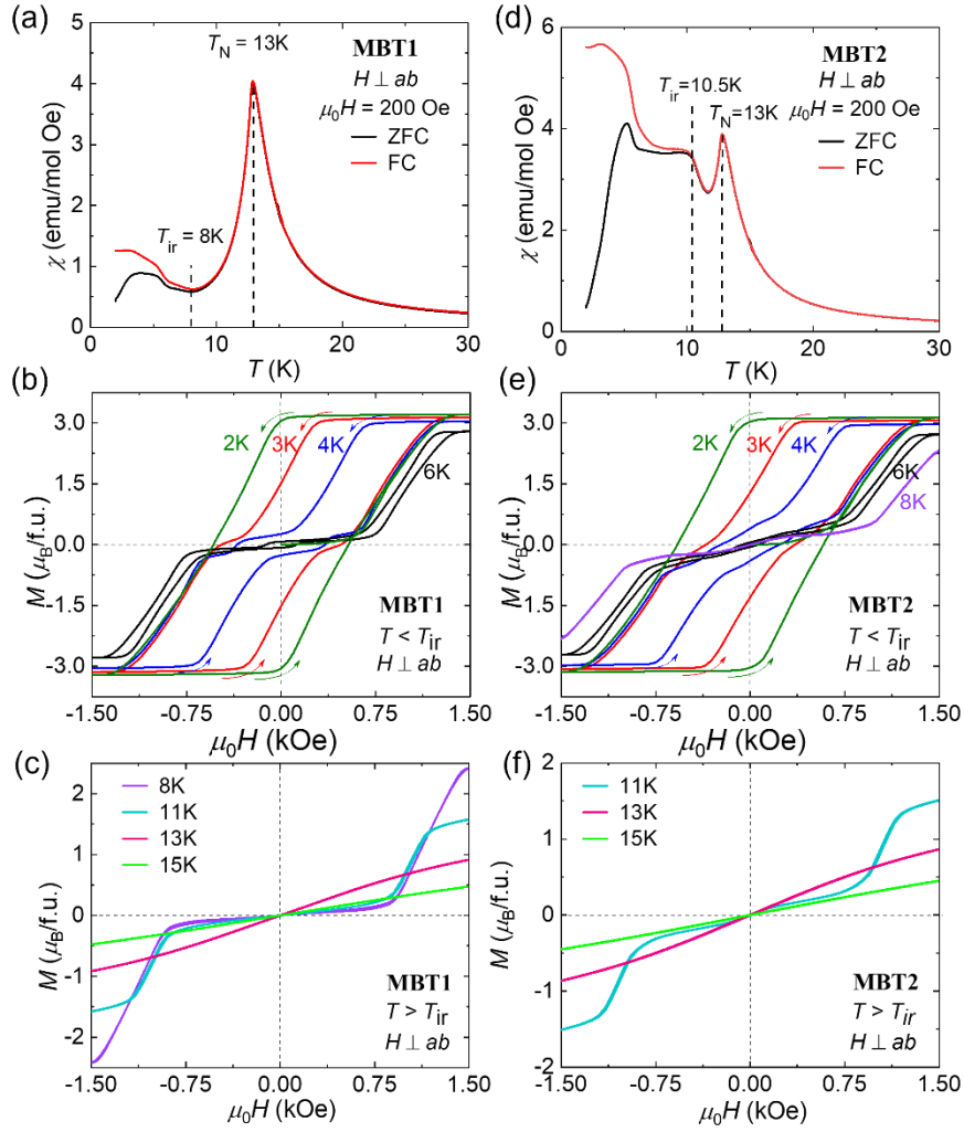
Fig. 2. (a,d) Temperature dependence of magnetic susceptibility measured under ZFC and FC histories for (a) MBT1 and (d) MBT2. Isothermal magnetization measured with H \perp ab -plane for (b,c) MBT1 and (e,f) MBT2 at temperatures below T_{ir} (b,e) and above T_{ir} (c,f).
