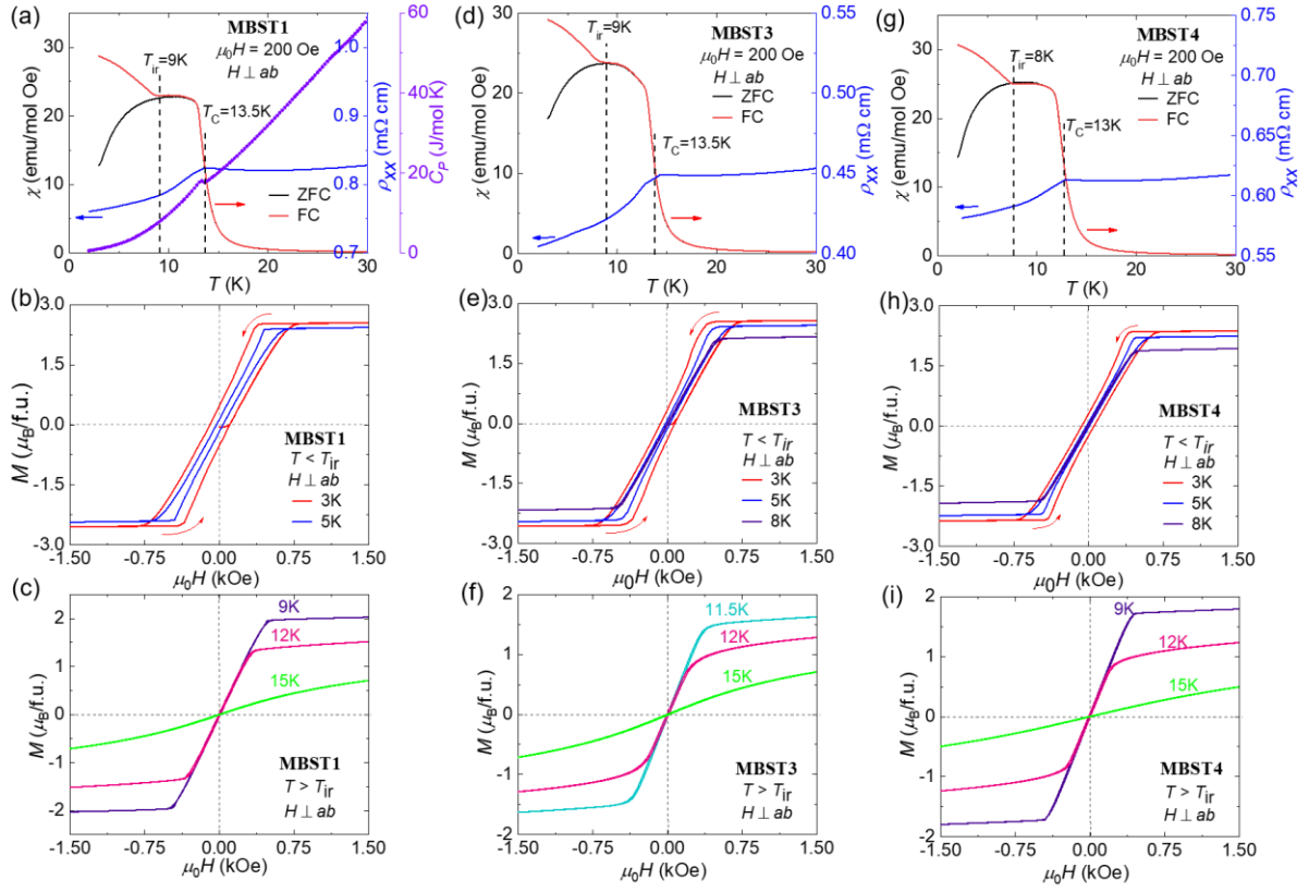
Fig. 3. (a, d, g) Temperature dependence of magnetic susceptibility measured under ZFC and FC histories for (a) MBST1, (d) MBST3 and (g) MBST4. The blue and the purple curves in (a, d, g) represent the temperature dependence of in-plane resistivity \rho_{xx} and specific heat for (a) MBST1, (d) MBST3 and (g) MBST4, respectively. Isothermal magnetization measured with H \perp ab -plane for (b, c) MBST1, (e, f) MBST3, and (h, i) MBST4 at temperatures below T_{ir} (b, e, h) and above T_{ir} (c, f, i).
