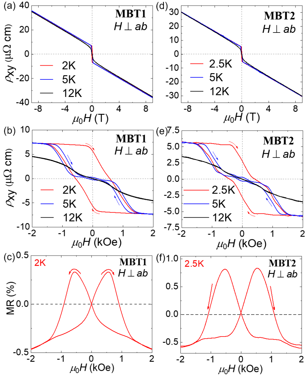
Fig. 5. (a, b, d, e) Field dependence of Hall resistivity \rho_{xy} measured with H \perp ab -plane in the -9 T – 9 T (a, d) and -2 kOe – 2 kOe (b, e) field ranges at various temperatures for MBT1 (a, b) and MBT2 (d, e). Transverse magnetoresistivity MR measured with H \perp ab -plane for (c) MBT1 and (f) MBT2 at 2.0 K and 2.5 K.
