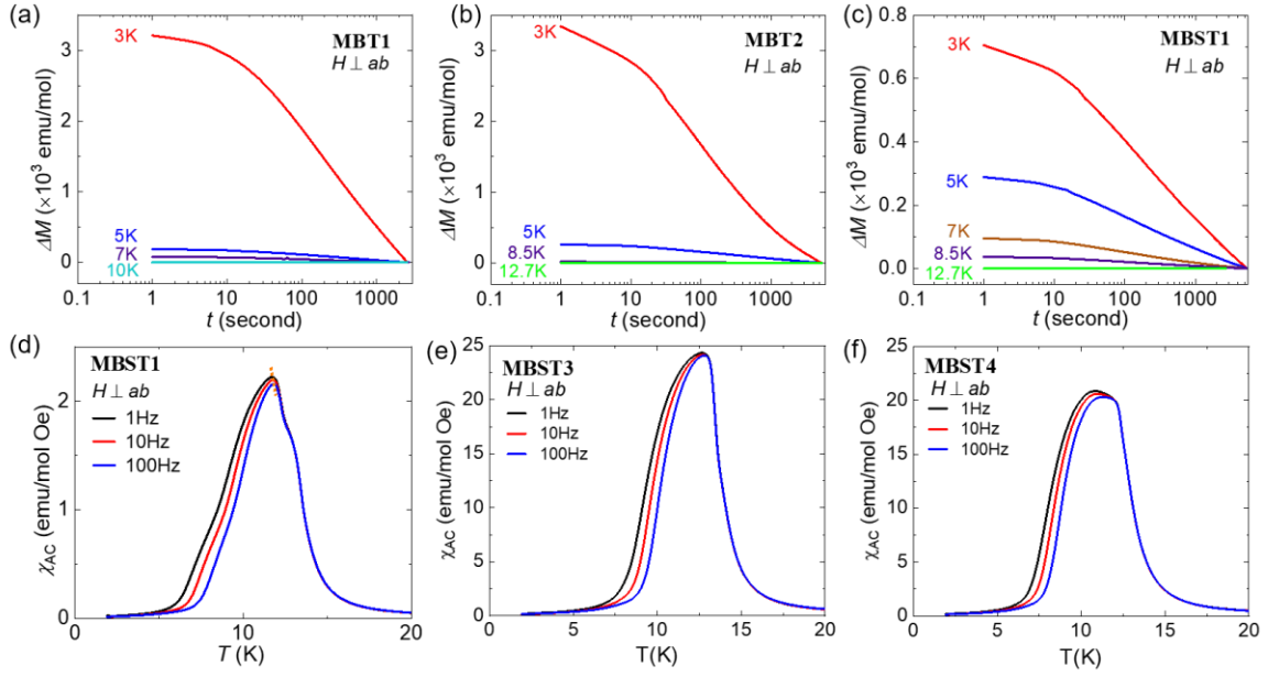
Fig. 4. Time dependence of magnetization measured right after ramping the magnetic field up to 5000 Oe ( H \perp ab -plane) and back to zero at various fixed temperatures for (a) MBT1, (b) MBT2, and (c) MBST1. Temperature dependence of AC susceptibility at various frequencies for (d) MBST1, (e) MBST3, and (f) MBST4.
