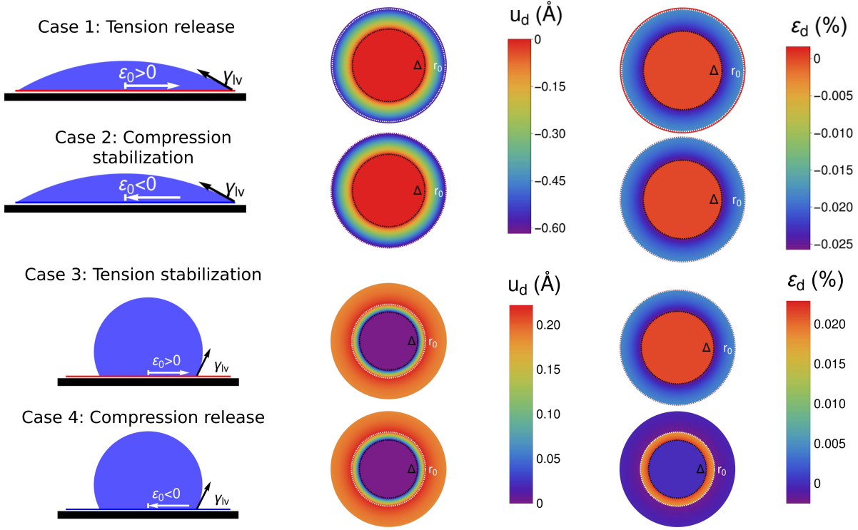
FIG. 5. Schematics, displacement and strains for a droplet on top of a strained film. For cases 3 and 4, a volume of V = 500 \mu\text{m}^3 was used; \gamma_{lv} = 0.45 \text{ MeV}^2 \mu\text{m}^{-1} and \gamma_{sl} = 0.40 \text{ MeV}^2 \mu\text{m}^{-1} were selected so that \gamma_{lv} would match that of water and the Young's angle, defined by Eqn. (8), was 110^\circ . Cases 2 and 4 use an initial strain of \varepsilon_o = -0.7\% . The white arrows indicate the direction of the displacements associated with the strain. For cases 1 and 4, the droplet has the potential to initiate decoupling of the film from the substrate. For cases 2 and 3, the droplet will likely stabilize the strain state.
