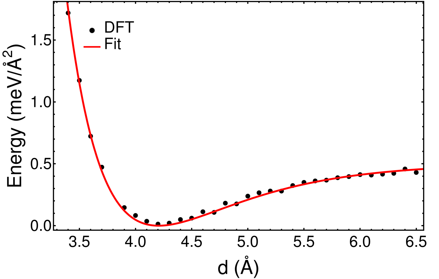
FIG. 6. Energy of \text{WSe}_2/\text{SiO}_2 system as a function of the film-substrate separation, d . The solid line is Eqn. (A3) using D_e = 0.50 \text{ meV } \text{\AA}^{-2} and \beta = 1.31 \text{ \AA}^{-1}
