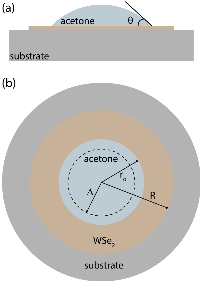
FIG. 1. A schematic of the continuum model: (a) side view and (b) top-down view. The WSe 2 sample is assumed to be circular in shape with unstrained radius R , and rigidly attached to the substrate within the radius \Delta , again defined in the unstrained material coordinate system. The material within this radius is assumed to be under the fixed biaxial strain \varepsilon_o (that arises from the synthesis process). The radius of the contact patch between the acetone and the film is taken to be r_o , also in the unstrained material coordinate system. The contact angle in Eqn. (8) is shown.
