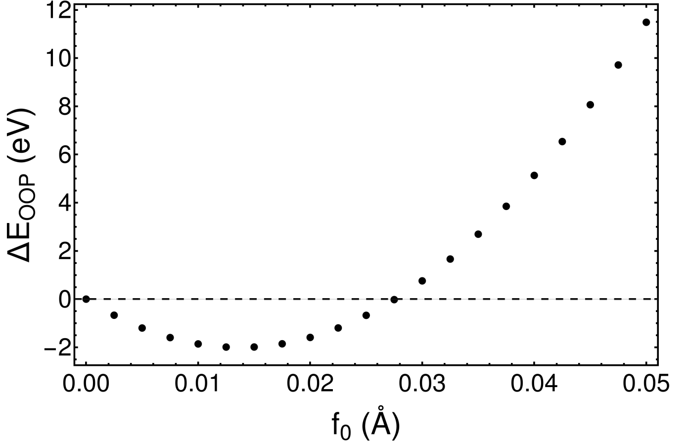
FIG. 7. Energy differences of systems with and without OOP displacement. The parameters used were those shown in Table I, V = 150 \mu\text{m}^3 , \Delta = 5 \mu\text{m} . The values for r_0 and u_0 were obtained using the formalism shown in Sec. II B.
