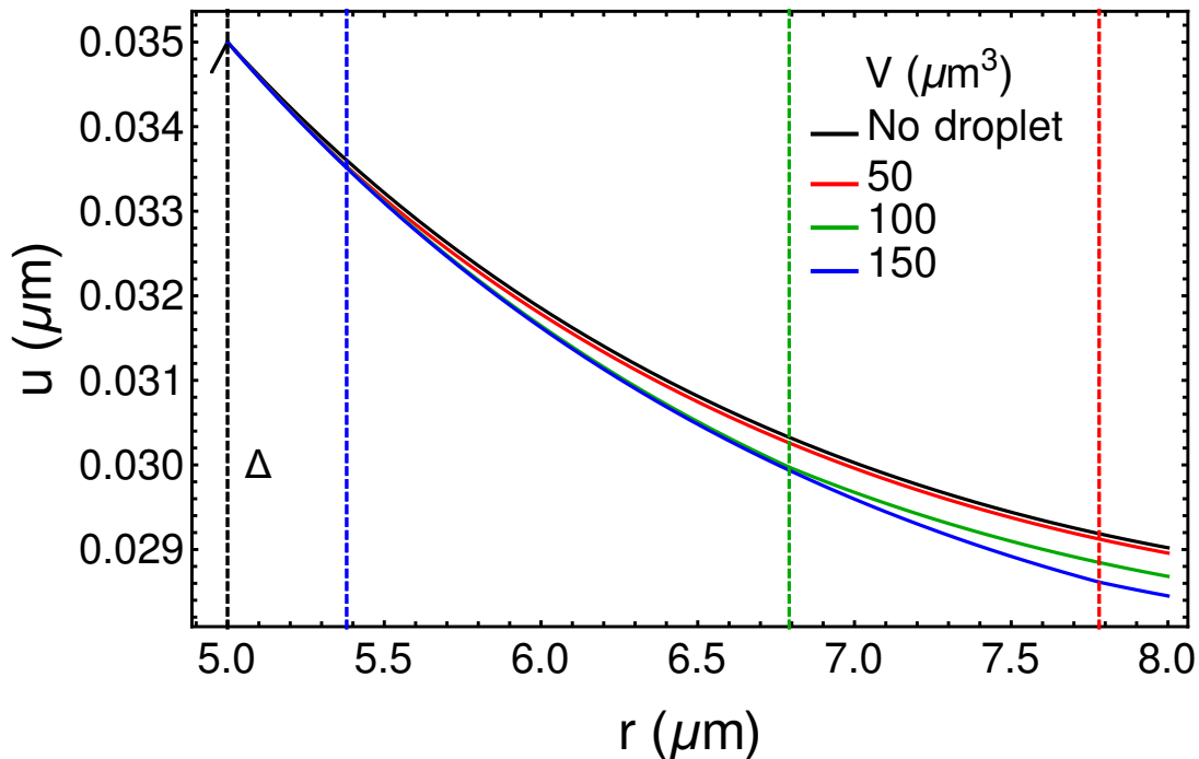
FIG. 3. In-plane displacement in the equilibrium configuration for a system with \Delta = 5 \mu\text{m} and different liquid volumes. The vertical black line corresponds to r = \Delta , while the others correspond to r = r_0 for the different values of V
