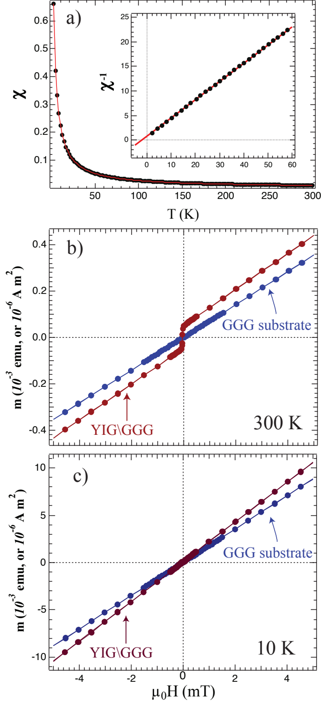
FIG. 4. a) \chi = M/H vs. T for the bare GGG substrate in \mu_0H = 10 mT vs. T from 2-300K. Inset: 1/\chi vs. T . In both the red line is a fit to the Curie-Weiss law with a small negative \theta , as expected for GGG. b) m vs. \mu_0H at 300 K for the GGG substrate and the YIG/(Gd-Y)IG/GGG sample. At this T both the large paramagnetic contribution from the GGG and the essentially ferromagnetic contribution from the YIG are obvious even without background subtraction. c) m vs. \mu_0H at 10 K, where the paramagnetic background dominates the ferromagnetic signal. The different slopes are due to a slight difference in the substrate volume.
