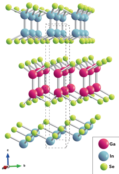
FIG. 1. (Color online) InSe/GaSe Superlattice. In, Ga, and Se atoms are represented by blue, pink, and green balls, respectively. The primitive cell has been expanded for a better representation of the layered nature of the superlattice.
