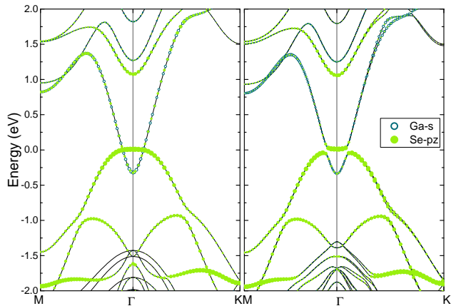
FIG. 4. (Color online) Projected band structure for InSe/GaSe superlattice under 5% tensile strain without (left) and with (right) SOC. The contribution from s-orbitals of Ga atoms and from p_z -orbital from Se atoms are represented by blue open circles and solid green circles, respectively.
