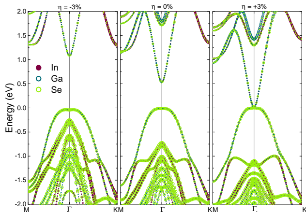
FIG. 3. (Color online) Projected band structure for InSe/GaSe superlattice with 3% compressive strain (left), fully relaxed (center), and 3% tensile strain (right). The In, Ga and Se atomic contributions to the band are represented by red, blue, and green circles, respectively.
