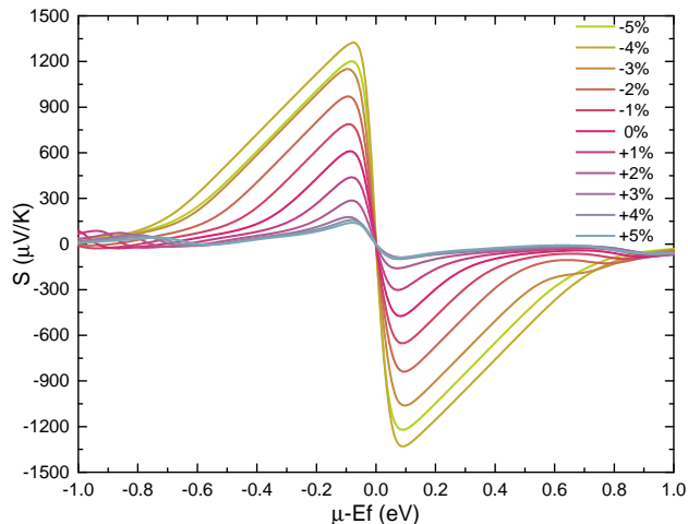
FIG. 5. (Color online) Calculated Seebeck coefficient as a function of the chemical potential for different values of strain at 500K of temperature.
