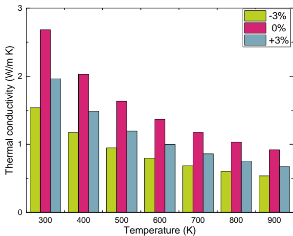
FIG. 7. (Color online) Trace of the lattice contribution to the thermal conductivity as a function of the temperature for three different strains -3\% , 0\% and +3\% .
