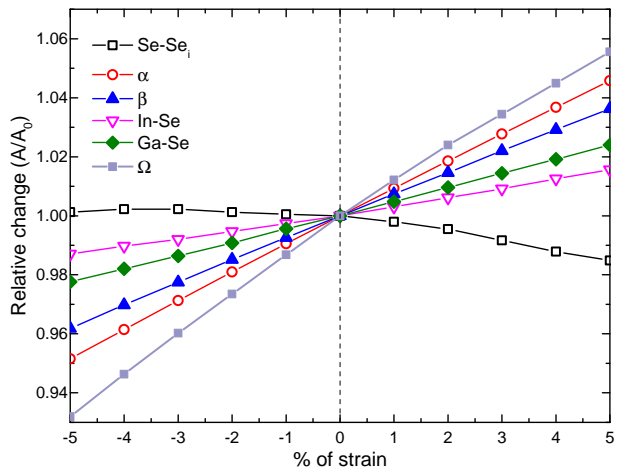
FIG. 2. (Color online) Relative change of the different distances and angles with respect to those in the fully relaxed structure. We are showing the following: Se-Se interlayer distance, Se-In-Se angle ( \alpha ), Se-Ga-Se angle ( \beta ), In-Se and Ga-Se bond length, as well as the total volume of the cell ( \Omega ).
