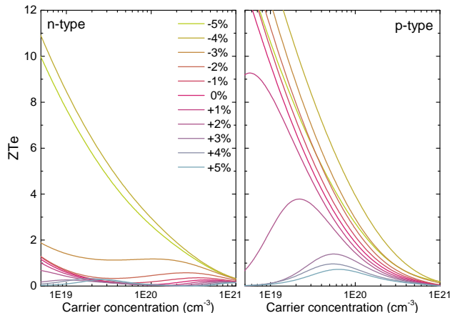
FIG. 6. (Color online) Carrier concentration dependence of the ZT_e ( [S^2(\sigma/\tau)]/(\kappa_e/\tau) ) trace for InSe/GaSe superlattice at different values of strain and 500K of temperature. The left panel shows n-type doping, while right panel shows p-type doping.
