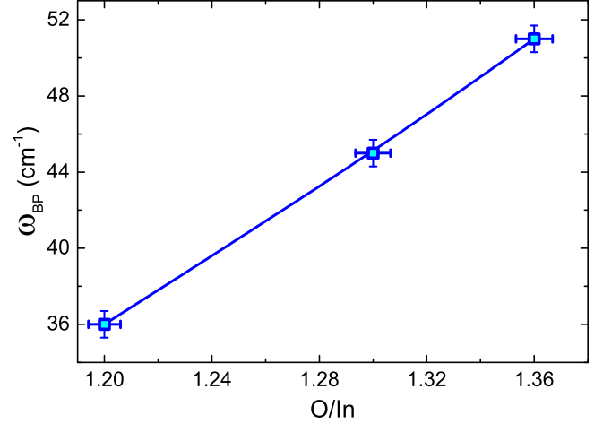
FIG. 3: The dependence of the energy of the BP maximum \omega_{BP} on the \text{In}_x\text{O} composition \text{O}/\text{In} . This is obtained through the relation between N and the oxygen/indium mass ratio studied elsewhere (Fig.6 in [19]).
