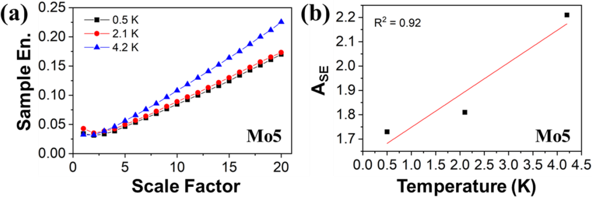
Figure 3. Results of the RCMSE analysis featuring the (a) sample entropy and (b) the area under the sample entropy curves ( A_{SE} ) for samples tested at 0.5 K, 2.1 K, and 4.2 K.
