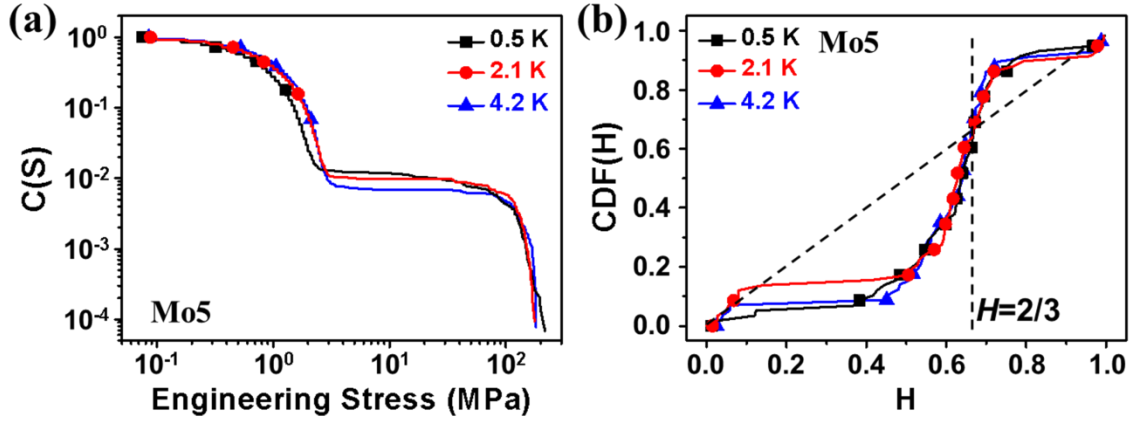
Figure 2. (a) Complementary cumulative distribution function (CCDF), C(S) , of avalanches (engineering stress) observed in the Mo5 alloy during tensile deformation at 0.5 K, 2.1 K, and 4.2 K. (b) Cumulative distribution function, CDF(H) , for the large avalanches, with sizes above 100 MPa, with respect to the H values obtained from the Bi-test. The black vertical line corresponds to H = \frac{2}{3} , and the black oblique line indicates a perfect Poisson process.
