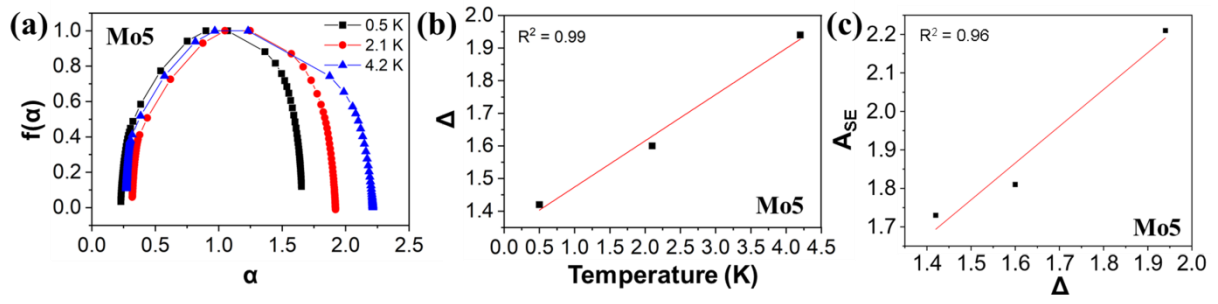
Figure 4. MFDFA results showing (a) the multifractal spectrum; (b) \Delta = \alpha_{max} - \alpha_{min} for samples tested at 0.5 K, 2.1 K, and 4.2 K; and (c) the A_{SE} vs. \Delta plot for the samples tested at the three temperatures.
