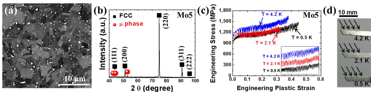
Figure 1. Initial microstructure of the Mo5 alloy: (a) SEM-BSE image and (b) XRD of the annealed Mo5 alloy. The white particles in (a) were identified as \mu precipitates. (c) Engineering stress-strain curves for the Mo5 alloy showing DPF at 0.5 K, 2.1 K, and 4.2 K. The inset in (c) reveals the enlarged and vertically shifted stress-strain curves exhibiting serrations at all three temperatures. (d) Photographs of the deformed tensile specimens at different temperatures. The black arrows in (d) point to localized shear bands.
