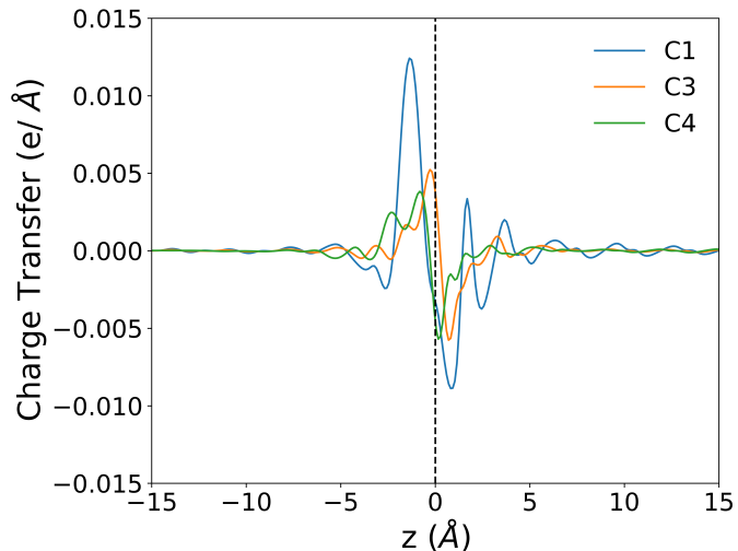
FIG. 10. Charge transfer as a function of distance from the interface for InAs/EuS with different configurations. The center of the interface is referenced to 0. The InAs is on the left side and the EuS is on the right side.
