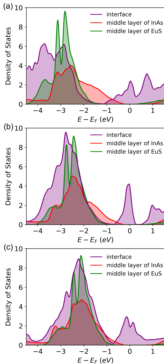
FIG. 8. Local density of states (LDOS) of (a) configuration C1, (b) configuration C3, and (c) configuration C4. The interface layer refers to the first InAs and EuS layers at the interface; The middle layer of InAs refers to the 38 th InAs layer from the interface; The middle layer of EuS refers to the 11 th EuS layer from the interface. The Fermi levels are shifted to 0 eV.
