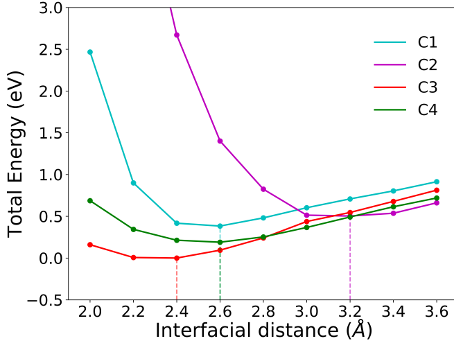
FIG. 4. Total energy change as a function of the interfacial distance for the four configurations. The lowest minimum is referenced to zero.
