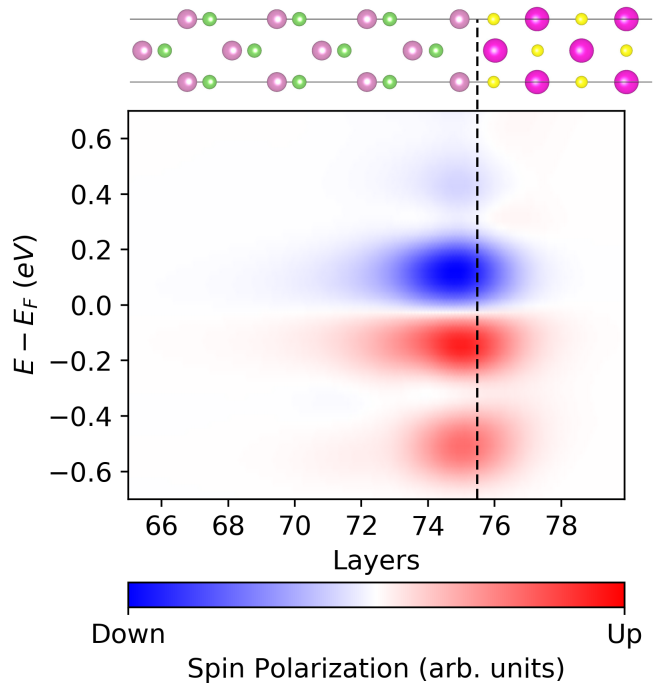
FIG. 11. Spin polarization (the difference between the majority DOS and the minority DOS) as a function of the layer index for configuration C3. Up and down refer to the spin-majority DOS and spin-minority DOS. The position of the interface is indicated by the black dashed line.
