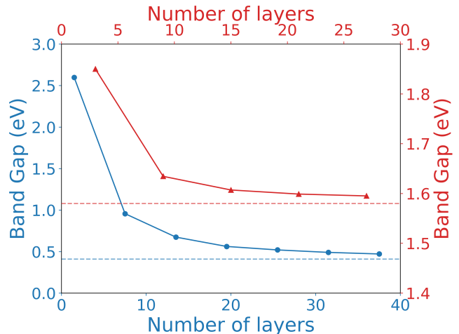
FIG. 1. The band gap of (a) InAs and (b) EuS slabs as a function of the number of atomic layers. Dashed lines denote the bulk limit of 0.41 eV for InAs and 1.58 eV for EuS.
