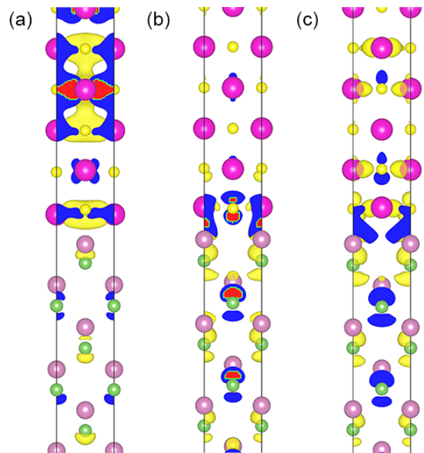
FIG. 9. The partial charges associated with the interface states of (a) configuration C1, (b) configuration C3, and (c) configuration C4 at \Gamma point. The electron charge isosurface is shown in yellow. Cross sections of the isosurface that intersect with the unit cell boundary are colored in blue and hollow cavities within the isosurface that intersect with the unit cell boundary are shown in red.
