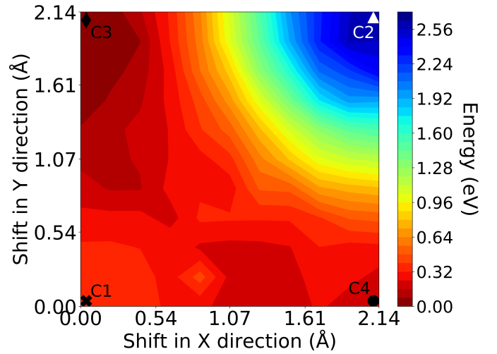
FIG. 5. PES scan at the interfacial distance of 2.4 Å
