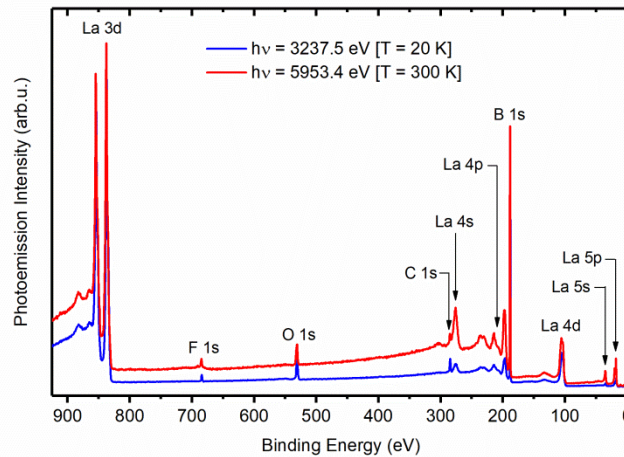
Figure 2. Survey spectra of LaB 6 , at 3237.5 eV (blue line) and at 5953.4 eV (red line) photon energies. The presence of O, C and F atoms suggests surface contamination.
