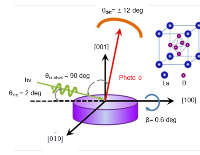
Figure 1. Experimental geometry used at BL15XU, Spring-8. The inset shows the crystal structure of \text{LaB}_6 . The crystal structure of \text{LaB}_6 is simple cubic (space group \text{Pm-3m} ), with \text{B}_6 -octahedra in body-centered positions and La atoms at the corners of the unit cell.
