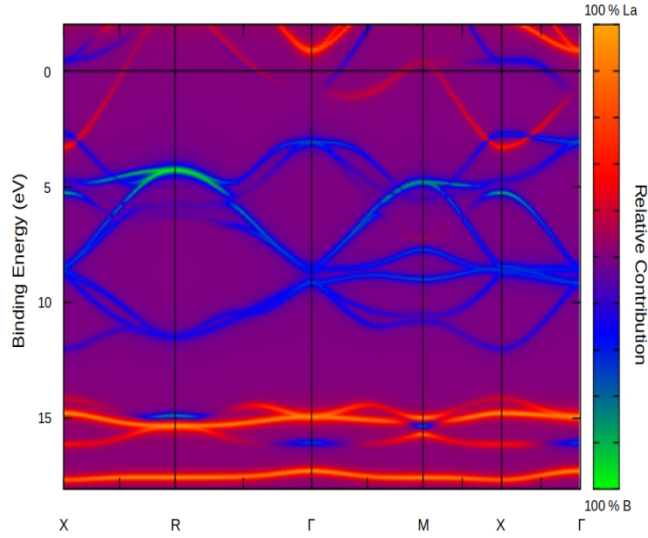
Figure 7. Calculated Bloch spectral functions projected onto La and B sites, showing mixed character of bands throughout the valence band region.
