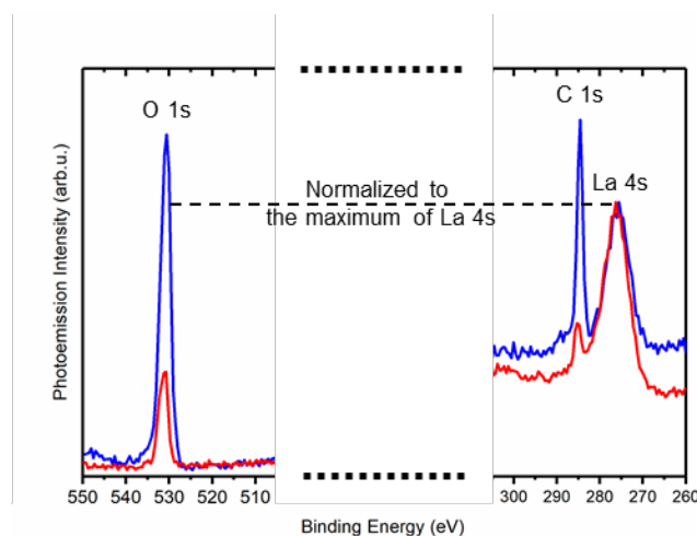
Figure 3. Core level spectra O 1s and C 1s normalized against La 4s measured at photon energies, 3237.5 eV (blue line) and 5953.4 eV (red line), respectively.
