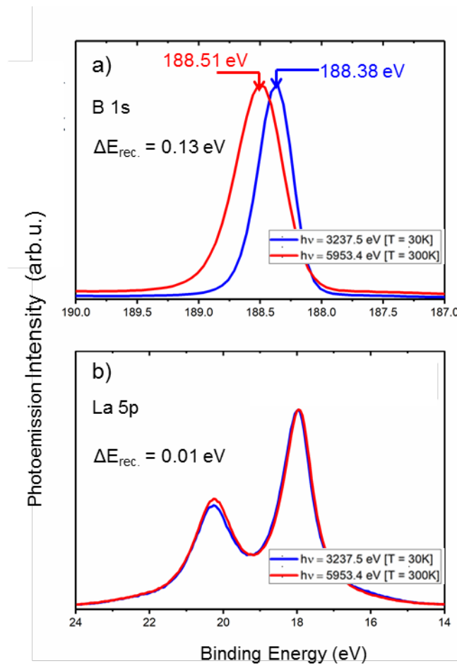
Figure 5. XPS spectra a) B 1s and b) La 5p measured at photon energies, 3237.5 eV (blue line) and 5953.4 eV (red line), respectively.
