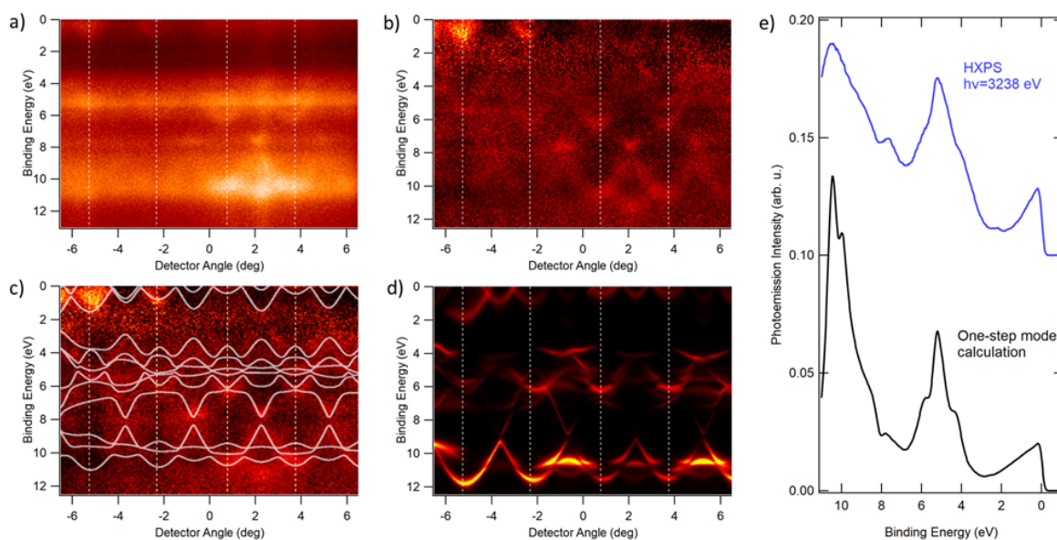
Figure 6. a) ARPES raw image collected at h\nu = 3237.5 eV and temperature 30 K; Fermi Energy is at BE = 0 eV; b) ARPES image normalized by the density-of-states (DOS) and by the x-ray
