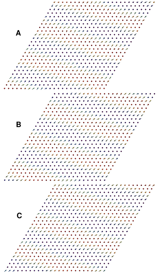
FIG. 3. A snapshot of spin spiral in a triangular AFM obtained by simulated annealing for K_{\text{eff}} = 0.4 , D_{\parallel} = 0.2 , h = 0 , and T = 0.02 on a 75 \times 75 triangular lattice with periodic boundary conditions. The letters on the left side (A, B, C) indicate the plotted sublattice. The colors indicate the orthogonal to the plane component of the spins.
