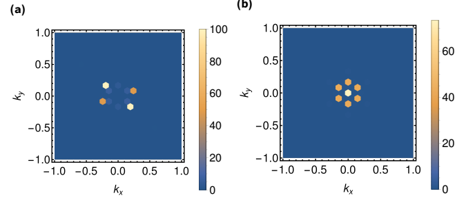
FIG. 5. Structure factor S_\parallel(\mathbf{q}) of a triangular AFM from Monte Carlo simulations. The vertical and horizontal axes represent the reciprocal space coordinates k_x and k_y in units of 1/L . The plot is for sublattice A ; those for B and C are almost identical. (a) The plot corresponds to spiral phase realizable for K = 0.4 , D_\parallel = 0.2 , h = 0 , and T = 0.02 . (b) The plot corresponds to SkX phase realizable for K = 0 , D_\parallel = 0.2 , h = 3.1 , and T = 0.02 .
