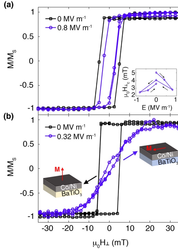
FIG. 4. Modulation of the out-of-plane magnetization in [\text{Co/Ni}]_4 multilayers controlled by a voltage applied along the [001] direction of BTO-1 (a) and BTO-2 (b). The inset in (a) shows the dependence of the out-of-plane coercive field on the electric field, which was varied in the order indicated by the arrows.
