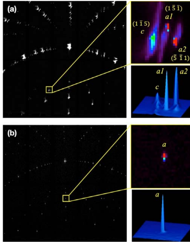
FIG. 2. Laue diffraction patterns of (a) BTO-1 and (b) BTO-2. Each spot in the Laue pattern is a reflection generated by a given crystallographic set of parallel planes which can be also defined by their normal; an arc of spots in the Laue pattern corresponds to a set of plane normals that are coplanar. The peaks marked in yellow frames are zoomed in on the top right and 3D surface plotted on the bottom right.
