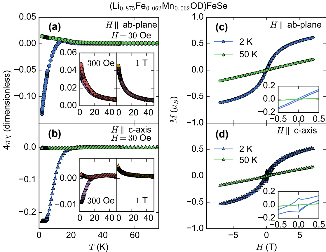
FIG. 4. Magnetic property measurements on an aligned single crystal of (Li 0.875(2) Fe 0.062(3) Mn 0.062(3) OD)FeSe. a)/b) Magnetic susceptibility data at various applied fields, aligned parallel to the crystallographic ab -plane and c -axis respectively, showing a superconducting transition at 25 K but no second magnetic transition at lower temperature. c)/d) Isothermal magnetization at 2 K and 50 K, with the same orientation convention, showing magnetic hysteric behavior superimposed on a superconducting signal at 2 K and paramagnetic behavior at 50 K. Note: (1 Oe = (1000/4 \pi ) A/m)
