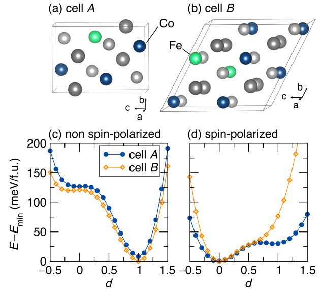
FIG. 5. Transition path energies between the hexagonal ( \text{MnFeGe} -like, d = 0 ) and orthorhombic ( \text{MnCoGe} -like, d = 1 ) structures of two different enumerated configurations of \text{MnCo}_{0.75}\text{Fe}_{0.25}\text{Ge} , (c) without and (d) with spin polarization. (a) Cell A shows a transition path landscape which is characteristic of that experienced by the majority of the enumerated cells, which remain orthorhombic after both nonmagnetic and magnetic structural relaxations. (b) Cell B is the special cell marked by an asterisk in Fig. 2, which transformed to the hexagonal structure during the spin-polarized relaxation.
