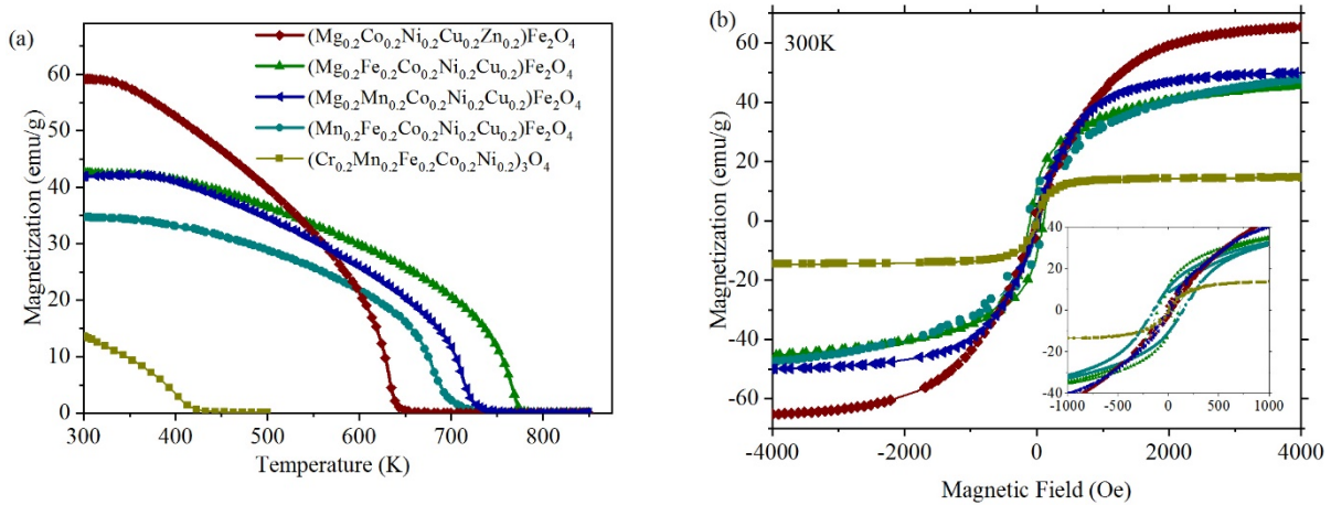
Figure 3: (a) Field cooled magnetization of ferritic HEO spinels from 300 K – 850 K with applied field of 1000 Oe and (b) magnetization as a function of applied field at 300 K with inset showing hysteretic behavior ( 1 \text{ emu} = 10^{-3} \text{ Am}^2 ). The legend in Fig (a) applies to both figures.
