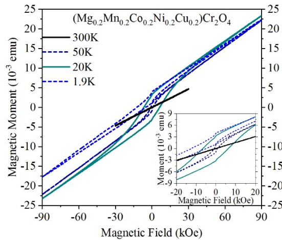
Figure 8: Magnetization with Field of (\text{Mg}_{0.2}\text{Mn}_{0.2}\text{Co}_{0.2}\text{Ni}_{0.2}\text{Cu}_{0.2})\text{Cr}_2\text{O}_4 at 300 K, 50 K, 20 K, and 1.9 K with inset better showing hysteresis.
