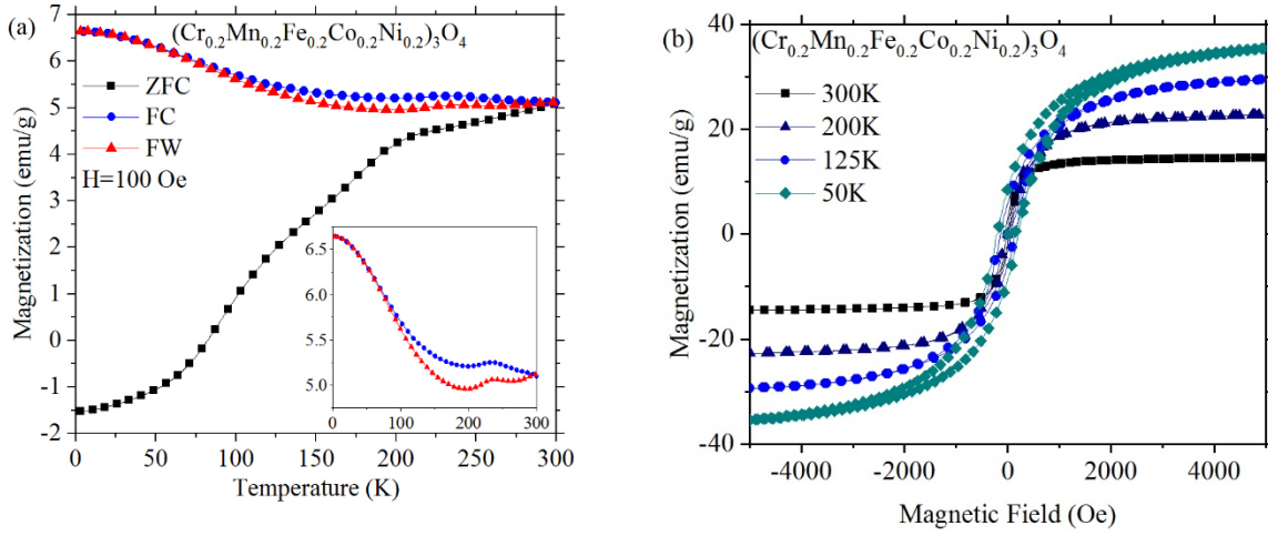
Figure 4: DC magnetization for (\text{Cr}_{0.2}\text{Mn}_{0.2}\text{Fe}_{0.2}\text{Co}_{0.2}\text{Ni}_{0.2})_3\text{O}_4 (a) as a function of temperature from 3 K - 300 K showing the zero field cooled (ZFC), field cooled, measured while cooling (FC) and field cooled, measured while warming (FW) plots; field cooled measurements were performed with an applied field of 100 Oe. (b) Magnetic hysteresis loops measured at 300 K, 200 K, 125 K and 50 K.
