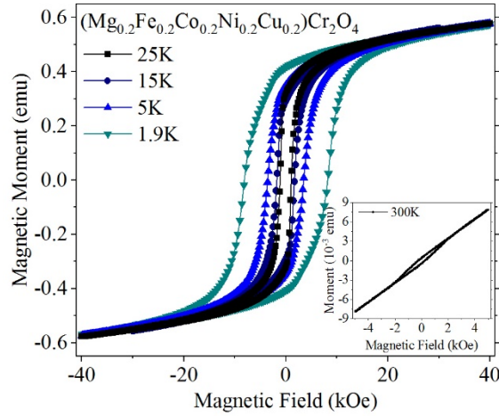
Figure 7: The hysteresis plots at 25 K, 15 K, 5 K and 1.9 K for (\text{Mg}_{0.2}\text{Fe}_{0.2}\text{Co}_{0.2}\text{Ni}_{0.2}\text{Cu}_{0.2})\text{Cr}_2\text{O}_4 with inset showing behavior at 300 K.
