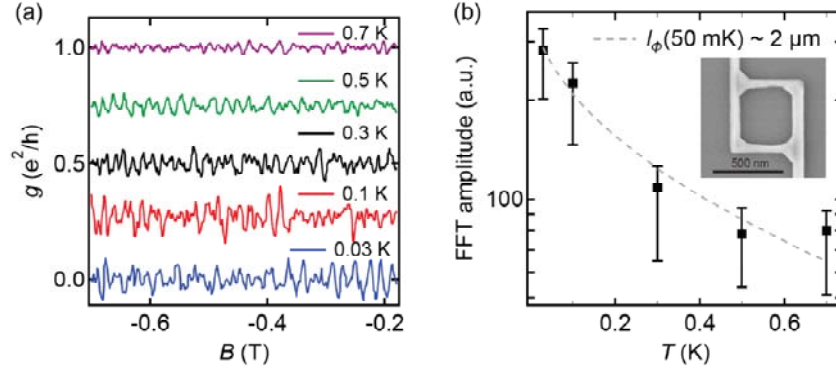
FIG 9. Measurement of the electron phase coherence length l_\phi in an AB geometry. (a) Magnetoconductance with subtracted background as a function of out-of-plane magnetic field B for different temperatures. Curves are vertically offset for clarity. (b) Integrated FFT of the oscillations plotted as a function of temperature. The fit (dashed grey line) corresponds to the amplitude decay within the diffusive regime with l_\phi \sim 2 \mu\text{m} at 50 mK. Inset: an SEM image of a grown AB loop.
