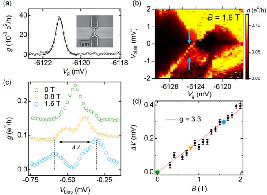
FIG 8. Measurement of the electron g-factor. (a) Coulomb peak close to pinch off in the split-gate geometry. Inset: an SEM image of the split-gate device. (b) The differential conductance g is plotted as a function of V_{\text{bias}} and V_g in the Coulomb blockade regime at an in-plane field B = 1.6 T. (c) Cuts along V_{\text{bias}} at a fixed V_g for different magnetic fields. The curves are shifted horizontally and vertically for clarity. (d) The extracted \Delta V for different in-plane fields with a linear fit to the data (red line).
