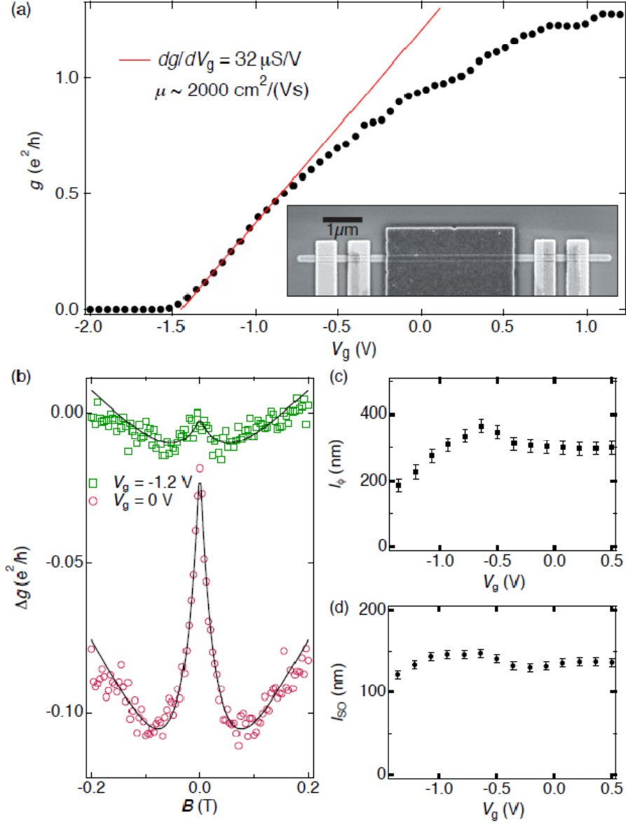
FIG 7. Transport characterization of field effect mobility and WAL. (a) Differential conductance of a selectively grown InAs NW as a function of gate voltage V_g . The solid red line is a linear fit to extract the peak in transconductance g_t . The inset shows an SEM image of the field effect mobility device. (b) Magnetoconductance \Delta g , offset to zero at zero field for two different gate voltages. The two curves are vertically offset. The WAL peaks are fitted with functions described in the main text (black lines). (c, d) Extracted phase coherence length l_\phi (c) and spin-orbit length l_{SO} (d) from WAL fits as a function of V_g .
