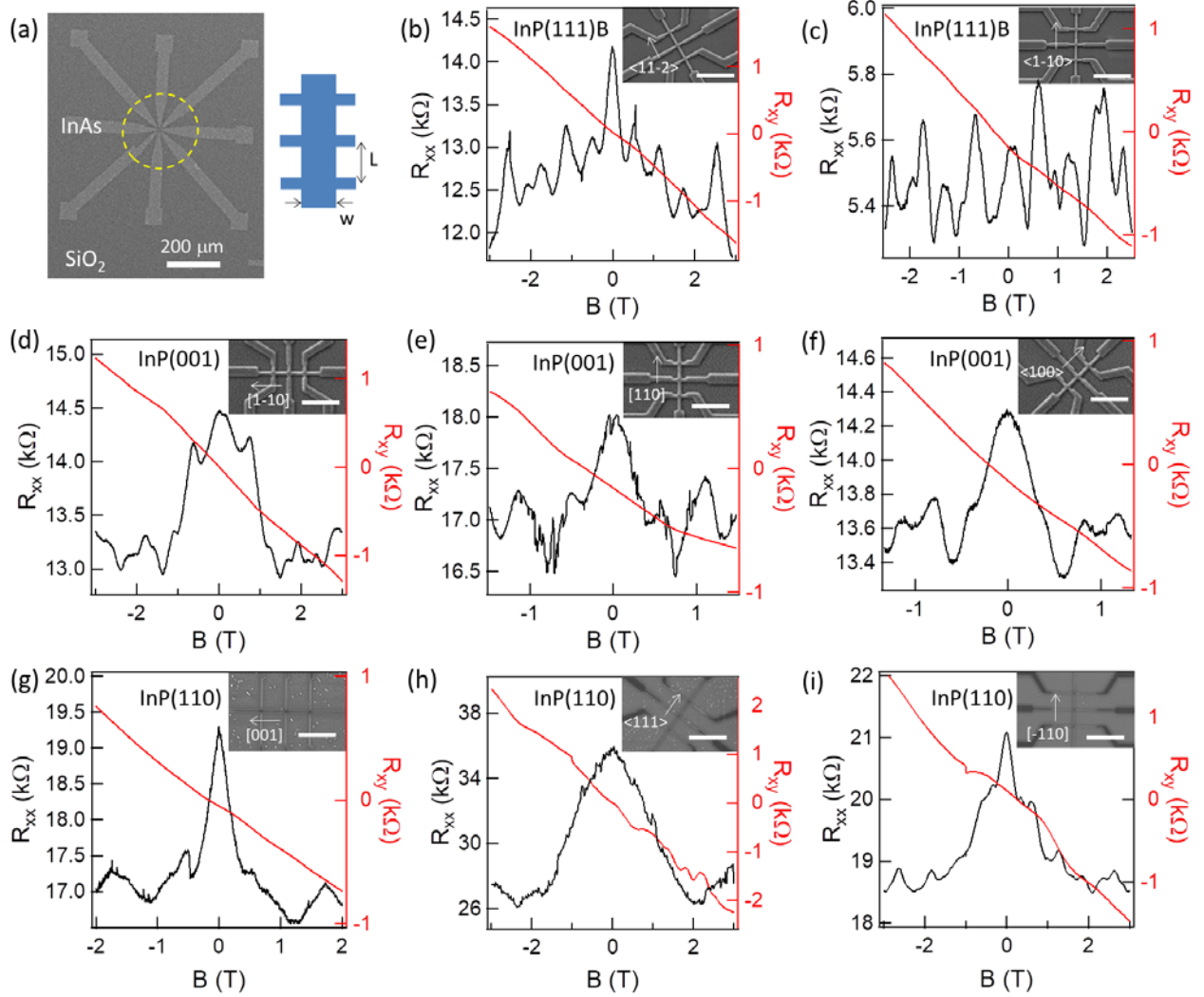
FIG 6. Hall measurements using a Hall bar geometry. (a) A low-magnification SEM image shows contact pads extended from a Hall bar, in the yellow dashed circle, illustrated as a schematic. Longitudinal resistance (black lines) and Hall resistance (red lines) were measured using Hall bar channels with various substrate orientations and channel directions: (b) along \langle 11-2 \rangle direction and (c) \langle 1-10 \rangle direction grown on an InP(111)B substrate, (d) along [1-10] direction, (e) [110] direction, and (f) \langle 100 \rangle direction grown on an InP(001) substrate, and (g) along [001] direction, (h) \langle 111 \rangle direction, and (i) [-110] direction grown on an InP(110) substrate. Insets: SEM images of measured Hall bars (scale bar: 2 \mu\text{m} ). All measurements were carried out at 2 K.
