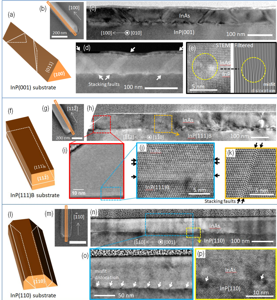
FIG 5. STEM/TEM images of NW cross-sections along the ridge direction. (a) A schematic and (b) an SEM image (b) of a NW along [100] direction grown on an InP(001) substrate. White lines in the schematic represent \{111\} planes in the NW, and the orange rectangle in the SEM image represents the position of the prepared cross-section. A conventional TEM image in (c) and an HAADF-STEM in (d) image reveal the inclined \{111\} stacking fault planes across the NW, indicated by white arrows in (d). (e) A misfit dislocation at the interface between InP and InAs is seen in an HAADF-STEM image and a filtered image. (f) A schematic and (g) an SEM image of a NW along [11\bar{2}] direction grown on an InP(111)B substrate. A conventional TEM image of the cross-section of the NW. Zoom-in images of the stacking faults near (i, j) the interface between the InP(111)B substrate and InAs and (k) a grain boundary. Black arrows represent the stacking fault planes. (l) A schematic and (m) an SEM image of a NW along [\bar{1}10] direction grown on an InP(110) substrate. (n) A HAADF-STEM image of the cross-section of the NW. (o, p) Zoom-in images show misfit dislocations at the interface between the InP(110) substrate and InAs.
