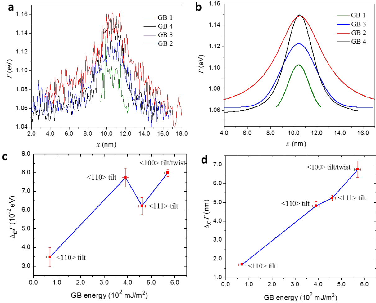
Figure 5: (a) Comparison of \Gamma profiles across all four GBs. (b) The Voigt fits, which depict the changes in \Delta_E \Gamma and \Delta_x \Gamma for the four GBs. (c) Plot of \Delta_E \Gamma as a function of GB energy. (d) Variation in measured \Delta_x \Gamma as a function of GB energy.
