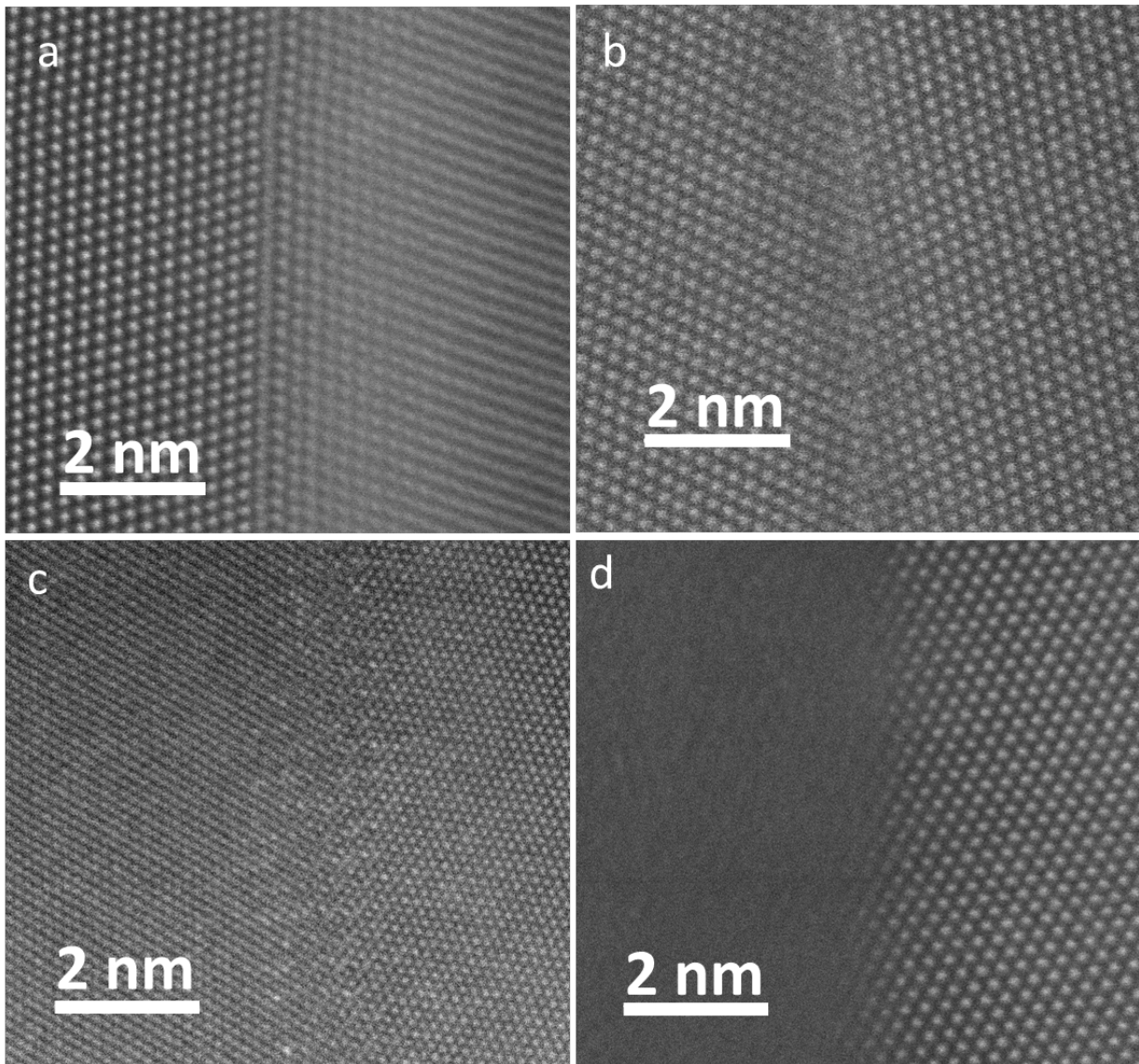
Figure 1: High-resolution STEM images of all four GBs in an edge-on position: (a) GB 1, (b) GB 4, (c) GB 3 and (d) GB 2.
