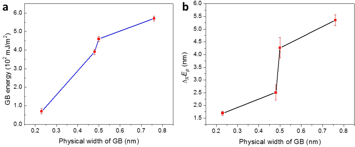
Figure 4: (a) Plot of GB energy versus physical width (measured from high-resolution STEM images). (b) Plot of measured \Delta x E_p as a function of GB physical width.
