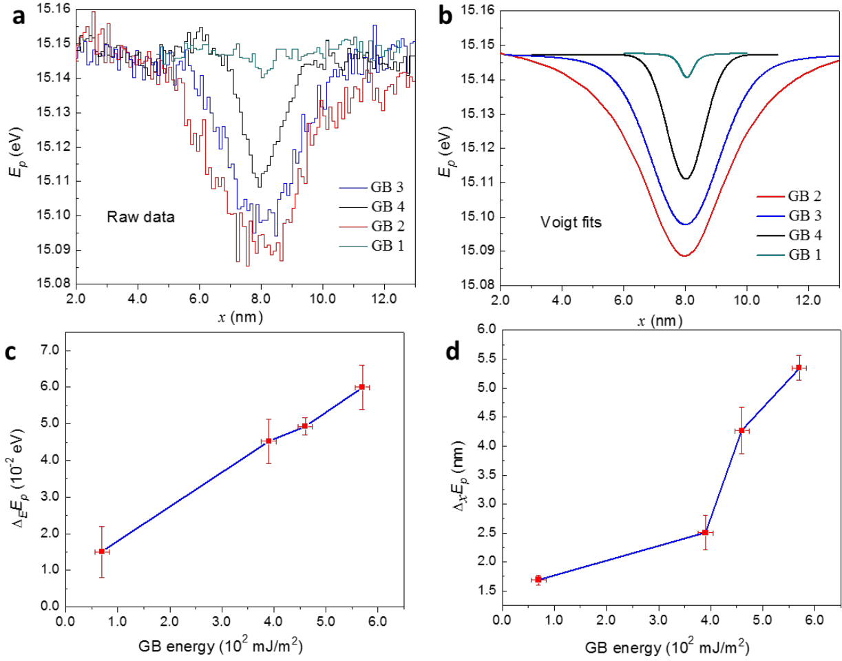
Figure 3: (a) Comparison of raw plasmon energy profiles experimentally obtained across all four GBs. (b) The Voigt fits, which depict the change in \Delta E_p and \Delta x E_p for the GBs. (c) Variation of \Delta E_p as a function of GB energy. (d) Dependence of \Delta x E_p with GB energy.
