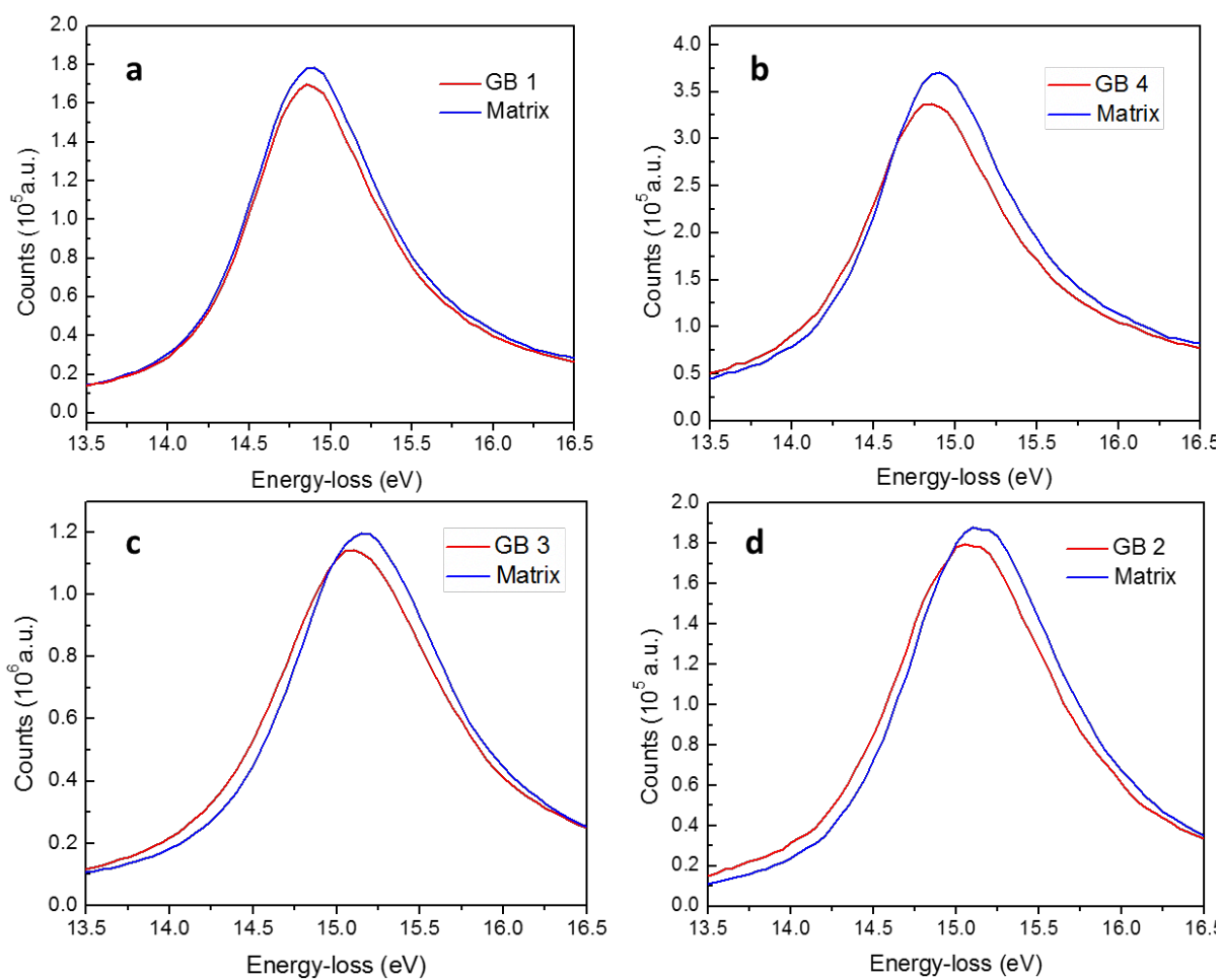
Figure 2: (a-d) Plasmon peaks from the low-loss spectra acquired from the GBs and adjacent grains (matrix) overlaid to reveal the increasing peak shifts toward lower energy with increasing GB energy.
