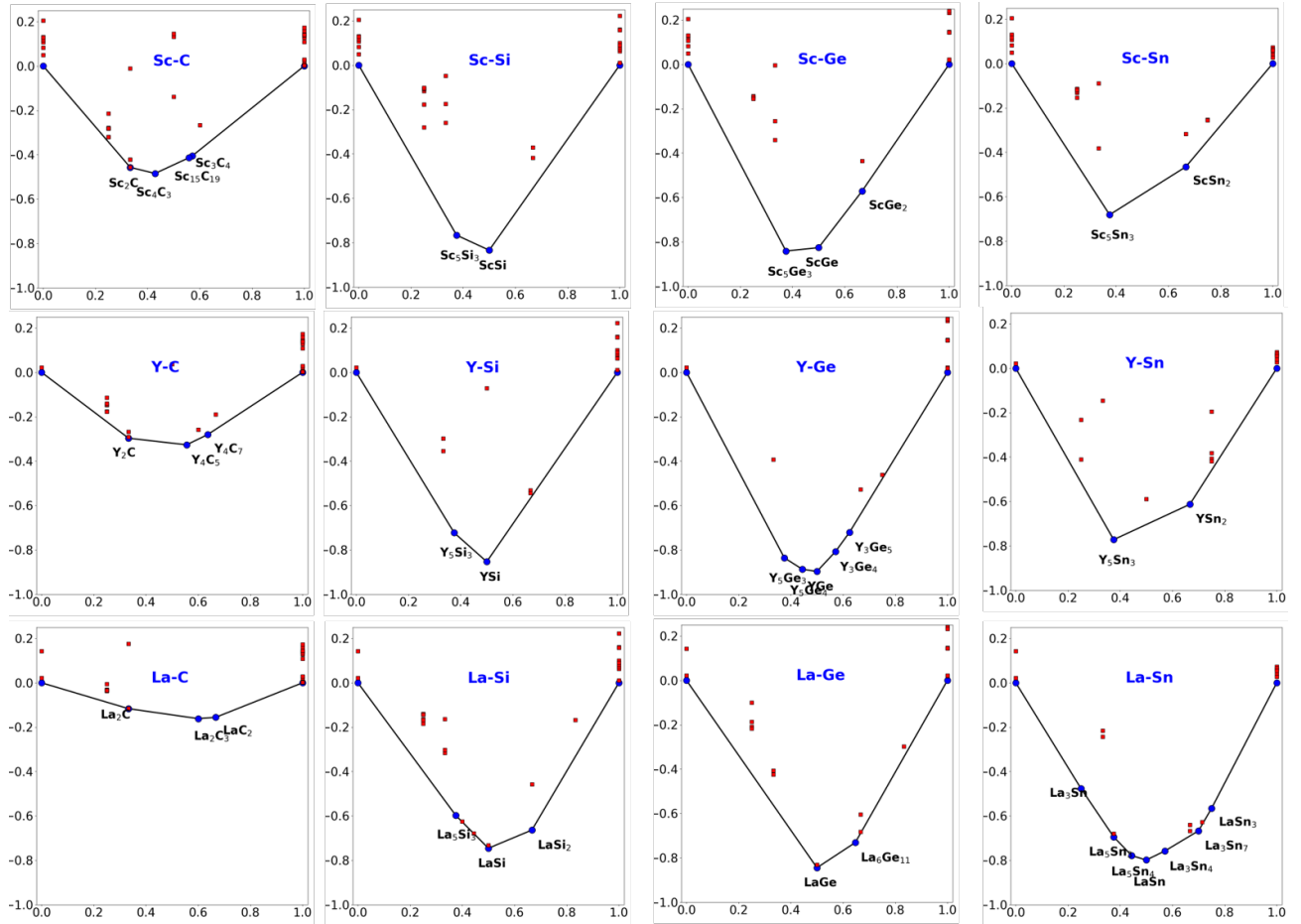
FIG. 10. The computed convex hull diagrams of group IIIB-IVA binary systems at PBE level based with the same parameters setting used in Materials Project. In each diagram, the x-axis is composition ratio, and the y-axis is the formation enthalpy in eV/atom relative to the ground states of the corresponding elemental allotropes.
