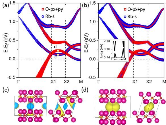
FIG. 5. Electronic band structures of \text{Rb}_3\text{O} without (a) and with (b) the SOC. The inset in (b) shows the enlarged band structure around X_1 and X_2 points with SOC. (c) and (d) show the wave functions of two eigenstates marked as c and d in the band structure (left: front view, right: side view).
