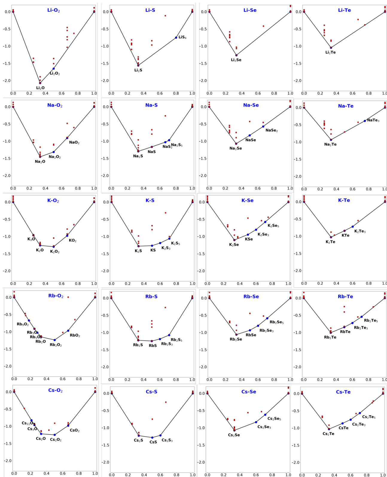
FIG. 11. The computed convex hull diagrams of group IA-VIA binary systems at PBE level based with the same parameters setting used in Materials Project. In each diagram, the x-axis is composition ratio, and the y-axis is the formation enthalpy in eV/atom relative to the ground states of the corresponding elemental allotropes.
