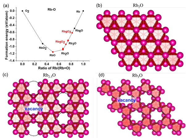
FIG. 1. (a) Convex hull diagram of the Rb-O system at opt-PBE level. Red circles denote metastable compounds; black squares represent stable compounds. The top view of monolayers in layered structures of R-3m Rb_2O (b), C2/m Rb_5O_2 (c) and C2/m Rb_3O (d), respectively.
