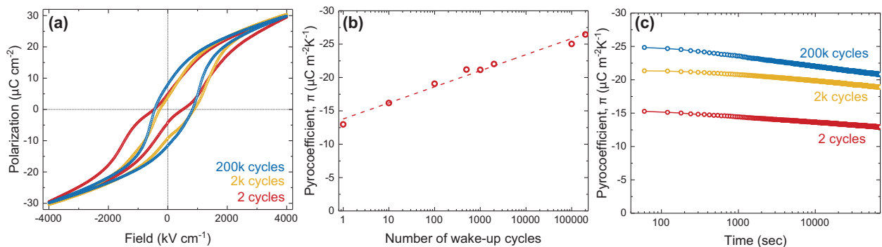
Figure 3. (a) Polarization-electric field hysteresis loop measurements conducted after electrically cycling the device for 2 (red), 2,000 (2k, yellow) and, 200,000 (200k, blue) cycles. (b) Measured pyroelectric coefficient ( \pi ) as a function of the number of wake-up cycles. The red dashed-line shows an empirical logarithmic fit to the measured data. (c) Pyroelectric-retention measurements conducted on samples after for 2 (red), 2,000 (2k, yellow), and 200,000 (200k, blue) wake-up cycles.
