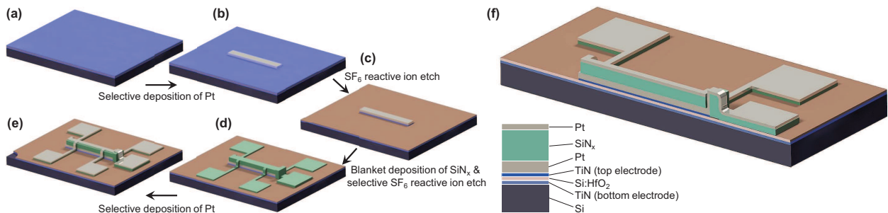
Figure 1. (a-e) Schematic illustration showing the fabrication of the electrothermal device through the various processing steps. (f) Cross-section view of the final device showing the various layers in the heterostructure.
