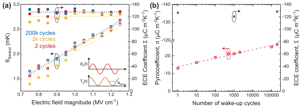
Figure 4. (a) Measured temperature change of the top metal line ( \theta_{Sensor} ; open squares, left axis) and the calculated value of the electrocaloric coefficient ( \Sigma ) (filled circles, right axis) on devices after 2 (red), 2,000 (2k, yellow), and 200,000 (200k, blue) wake-up cycles. Inset shows the schematic of the phase relationship between the applied electric field and the temperature. (b) Comparison of \pi (red circles, left axis) with \Sigma (black squares, right axis) as a function of the number of wake-up cycles.
