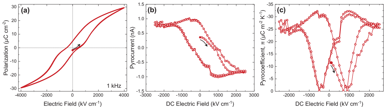
Figure 2. (a) Polarization-electric field hysteresis loop measurements showing a pinched or constricted hysteresis loop in the as-received Si:HfO 2 films. (b) Pyroelectric current ( i_p ) and (c) pyrocoefficient ( \pi ) measured as a function of background DC electric field, at 1 kHz. The black arrows and filled red data point show the direction and starting point of the measurements.
