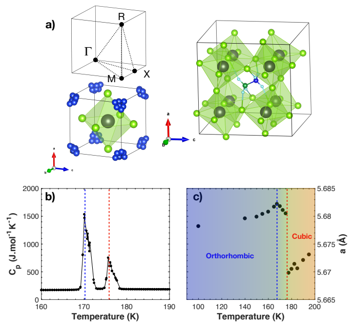
FIG. 1. (a) left: Crystallographic structure of MAPbCl 3 in the cubic phase. The Pb site is represented by the grey sphere, the Cl ions are shown in green, and the methylammonium molecules are represented in blue in their disordered state. The top figure shows the high symmetry points in the first Brillouin zone of a primitive cubic lattice. X , M and R represent \mathbf{Q} = (\frac{1}{2}, 0, 0) , (\frac{1}{2}, \frac{1}{2}, 0) , and (\frac{1}{2}, \frac{1}{2}, \frac{1}{2}) , respectively. right: Crystallographic structure of MAPbCl 3 in the orthorhombic phase. In this ordered phase, the H, N and C atoms forming methylammonium molecules are represented with light blue, dark blue and dark green spheres, respectively. (b) Heat capacity as a function of temperature for MAPbCl 3 . (c) Temperature dependence of the cell parameter a , measured on BT4 (NIST). The dashed lines indicate the two structural transitions in MAPbCl 3 .
