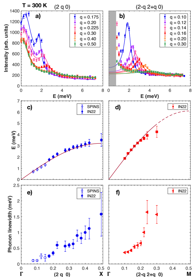
FIG. 2. (a)-(b) Constant- Q cuts through the acoustic phonon \text{TA}_1 for several Q positions from the (2\ 0\ 0) Bragg peak towards the X point and from the (2\ 2\ 0) Bragg peak towards the M point ( \text{TA}_2 mode), respectively. The grey area corresponds to the region in energy contaminated by strong scattering from aluminium. (c)-(d) Dispersion curves associated to the \text{TA}_1 mode towards the X and the \text{TA}_2 mode towards the M point respectively. The red line is a fit to a sine function. (e)-(f) Q -dependence of the \text{TA}_1 and \text{TA}_2 phonon linewidths extracted from the constant- Q cuts as described in the text.
