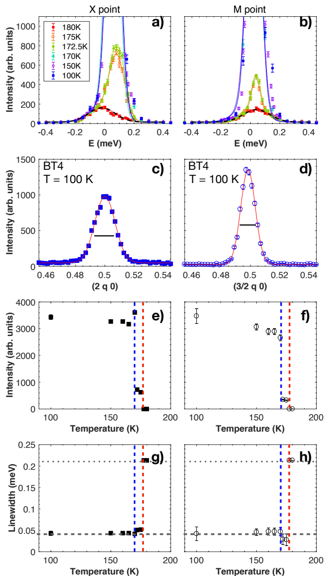
FIG. 4. (a) – (b) Energy scans measured on TASP (PSI) around X = (2, \frac{1}{2}, 0) and M = (\frac{3}{2}, \frac{1}{2}, 0) respectively, at several temperatures. (c) – (d) Momentum scans around the X and M points performed on BT4 at T = 100 K. The solid lines show the instrumental Q resolution. (e) – (f) Temperature evolution of the integrated intensity extracted from these energy scans. (g) – (h) Temperature evolution of the linewidth extracted from the energy scans. The grey dotted lines show the energy resolution extracted from the width of the incoherent line of vanadium, the grey dashed lines show the Bragg width and the colored dashed lines limit the two structural transitions of \text{MAPbCl}_3 .
