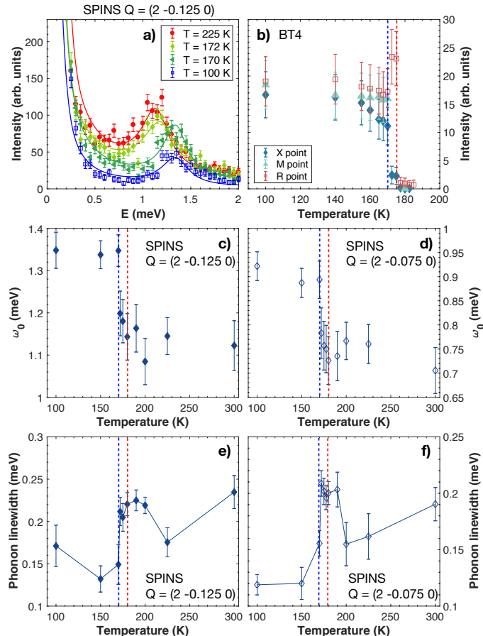
FIG. 3. (a) Constant Q = (2 -0.125 0) scans at several temperatures, measured on SPINS (NIST). (b) Temperature evolution of the integrated intensity measured with E = 0 at the X , M and R points measured on BT4 (NIST). (c) - (d) Temperature evolution of the energy position of the TA 1 mode, extracted at the Q = (2 -0.125 0) and Q = (2 -0.075 0) positions, respectively. (e)-(f) Temperature evolution of the TA 1 phonon linewidth, extracted at the Q = (2 -0.125 0) and Q = (2 -0.075 0) positions, respectively.
