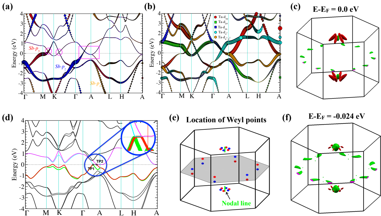
FIG. 2. (Color online) Figures (a-b) represent the electronic band structure calculated without inclusion of SOC. Projection of the Sb- p atomic orbitals is shown in panel (a) while projection of Ta- d orbitals is shown in panel (b). The magenta circles mark the location of points that belong to a Dirac nodal line centered at K-point, and magenta rectangles depicts the location of gapless nodal line present along the \Gamma - A path. Panel (d) represents the electronic band structure calculated with-SOC. The inset of panel (d) shows the enlarged view of the gapless nodal line. The locations of triple-points (TP1 and TP2) at the end of the gapless nodal line are marked by black circles. For better visibility, bands near the Fermi-level are plotted in different colors. Location of all the Weyl points present in the Brillouin zone is shown in panel (e) (For their exact locations, see Tab. I). Red (blue) spheres denote the Weyl points having positive (negative) chirality. The green lines mark the location of the gapless nodal line. Six pairs of Weyl points that appear in the shaded k_x - k_y plane are of type-I, while the other six pairs of Weyl points that surround the gapless nodal line are of type-II. Panels (c) and (f) show the Fermi-surface calculated at E - E_F = 0.0 eV and E - E_F = -0.024 eV, respectively. One can observe the formation of type-II Weyl points as touching points of electron and hole pockets along the \Gamma - A path.
