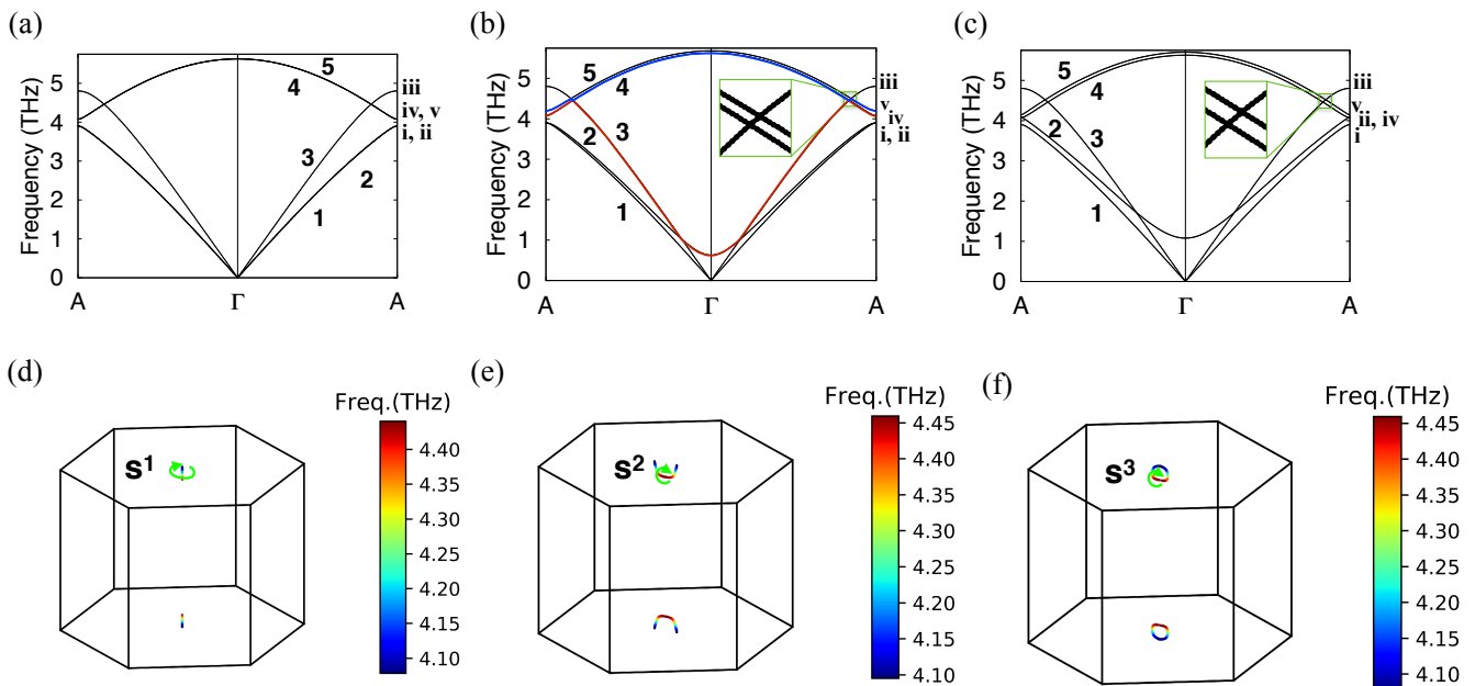
FIG. 4. (Color online) (a) The phonon spectrum of TaSb along the C_{3v} -symmetric line of the BZ: Doubly degenerate phonon bands (4,5) and (iv,v) can be seen. (b) The phonon spectrum of TaSb with the xx and yy force constants in the dynamical matrix made unequal for Ta. The degeneracy of (4,5) and (iv, v) is lifted. (c) The phonon spectrum of TaSb with the xx and yy force constants in the dynamical matrix made unequal for Sb. The degeneracy of (4,5) and (iv, v) is lifted. (d) The non-topological open nodal line formed in the BZ by bands iv and v of panel (a). The loop S^1 encircles this line, but \phi_B(S^1) = 0 . (e) The closed nodal loop formed by bands iv and v in the BZ for the case of panel (b) away from the \Gamma -A line. The contour S^2 links with this loop and \phi_B(S^2) = \pi . (f) The closed nodal loop formed by bands iv and v in the BZ for the case of panel (c). For a contour S^3 linked with this loop \phi_B(S^3) = \pi .
