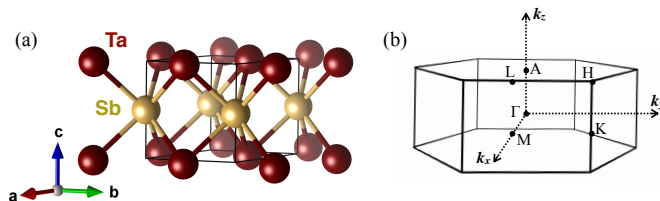
FIG. 1. (Color online) (a) Crystal structure of TaSb compound in WC-type P\bar{6}m2 space group. Ta atoms (maroon) occupy the (2/3, 0.0, 2/3) site, and Sb atoms (golden) occupy the (0.0, 1/2, 0.0) site. The unit cell contains one Ta and one Sb atom. (b) Brillouin zone (BZ) of TaSb.
