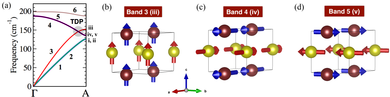
FIG. 3. (Color online)(a) Part of the phonon spectrum of TaSb. The triply-degenerate point (TDP), at which phonon bands 3(iii), 4(iv) and 5(v) meet is the topologically protected triple-point of phonons (another such point is located in the other direction in the BZ on the same C_{3v} -symmetric line). Panels (b, c, d) explicitly illustrate the atomic vibrations corresponding to the overlapping phonon modes 3(iii), 4(iv) and 5(v) correspondingly. The enumeration of phonon bands is made with numbers (1..6) and (i..vi) “before” and “after” the crossing point, to stress the change in phonon band ordering by using different number styles for ordinary and inverted phonon band orderings.
