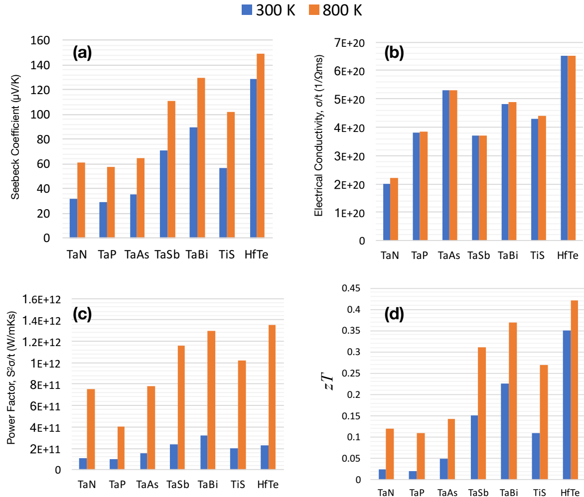
FIG. 7. (Color online) (a) Maximum of Seebeck coefficient or thermopower, (b) maximum of electrical conductivity ( \sigma/t ) obtained at 300 K and 800 K, (c) maximum power factor at 300 K and 800 K, and (d) the theoretical maximum of zT . Above data is for electron doping case.
