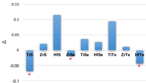
FIG. 6. (Color online) Normalized phonon frequency gap ( \Delta ) calculated near the A-point of BZ for the set of nine compounds reported in Ref. 22 . A negative value of \Delta implies the presence of phonon band-inversion. Only three compounds (marked with asterisk) show negative \Delta .
