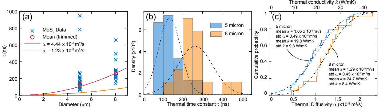
FIG. 2. (a) Thermal time constants as function of diameter. Predictions using eq. 4 are plotted with several values of k obtained from literature: k = 23.3 \text{ W}/(\text{m} \cdot \text{K}) corresponding to \alpha = 1.23 \times 10^{-5} \text{ m}^2/\text{s} , 12 and 84 \text{ W}/(\text{m} \cdot \text{K}) to \alpha = 4.44 \times 10^{-5} \text{ m}^2/\text{s} . 18 (b) Density plot of the thermal time constant for both diameter, drums with extremely large values of \tau and low resonance frequency were excluded. (c) CDF (cumulative density function) of the thermal conductivity k estimated from the values of \tau using c_p = 373.5 \text{ J}/(\text{kg} \cdot \text{K}) and \rho = 5060 \text{ kg}/\text{m}^3 .
