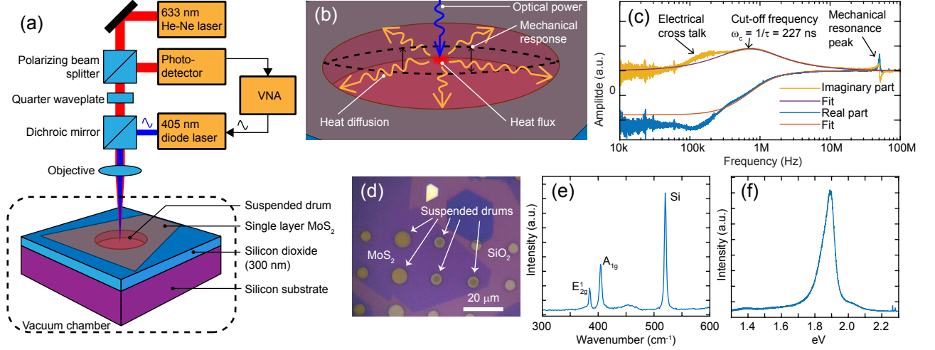
FIG. 1. (a) Schematic of the samples and the laser interferometer setup to actuate and detect the motion of the single-layer MoS 2 drum resonators. (b) Overview of the physical processes involved in measuring the transient properties of heat transport in the drum. (c) Typical experimental result of the real (in-phase) and imaginary (out-of-phase) part of the amplitude of the mechanical response of the drum. The imaginary part of the amplitude was fitted to Eq. 3 to find the thermal time constant. At lower frequencies, a feature due to electrical crosstalk becomes visible due to the low optical gain during the experiment (see Supplemental material). At higher frequencies, the fundamental resonance is clearly visible. (d) Optical image of the device showing a single-layer MoS 2 sheet on top of the substrate and several suspended drums. (e) Raman spectrum of the suspended MoS 2 . (f) Photoluminescence spectrum of the suspended MoS 2 . The A 0 peak position is found at 1.89 eV.
