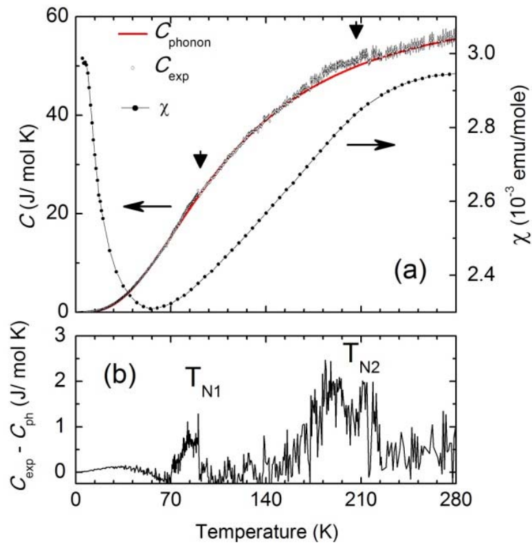
Figure 1. Temperature dependent (a) zero-field cooled dc magnetic susceptibility, \chi(T) (right-axis), under an applied field of 20 mT, and the heat capacity, C(T) (left-axis), of \beta -NaMnO 2 . The red line over the C(T) data is the calculated phonon contribution to the specific heat, C_{\text{ph}}(T) (see text). (b) The heat capacity remaining after subtracting the C_{\text{ph}}(T) contribution from the experimental C(T) depicts two anomalies assigned as T_{N1} and T_{N2} .
