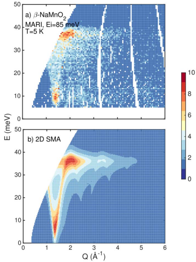
Figure 12. (a) The powdered averaged magnetic scattering in \beta -NaMnO 2 and (b) the corresponding Single Mode Approximation (SMA) heuristic model, with two-dimensional (2D) interactions. The background subtraction method to remove phonon scattering and instrument background are described in the text. Color map: indicates the powder average scattering intensity \bar{I}(\vec{Q}, \hbar\omega) (see text for details).
