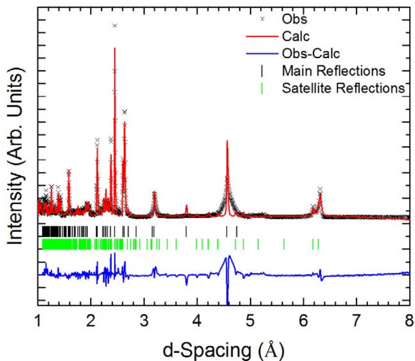
Figure 8. Rietveld plot at 100 K of the \beta - \text{NaMnO}_2 structure in C_{a2'}/c'(\alpha 0 \gamma)00 superspace group, with cell parameters a = 5.7108(2) \text{ \AA} , b = 12.6394(9) \text{ \AA} , c = 5.5397(4) \text{ \AA} , \beta = 120.96(7)^\circ , and \mathbf{q} = (0, 0, 0.078(1)) . Observed (black crosses), calculated (red line) and difference (blue line) patterns are reported. The tick marks indicate the calculated position of the main (black ticks) and satellite reflections (green ticks).
