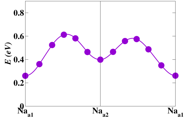
FIG. 7. Computed energy path diagram for Na-ion vacancy migrations in bulk \text{Na}_3\text{SbS}_3 corresponding to nearest neighbor hops between \text{Na}_{a1} and \text{Na}_{a2} sites. The symbols represent directly calculated configurations while the lines are smooth interpolations between NEB images. The zero of energy is set at the energy of a Na-ion vacancy at a \text{Na}_{a3} site.
