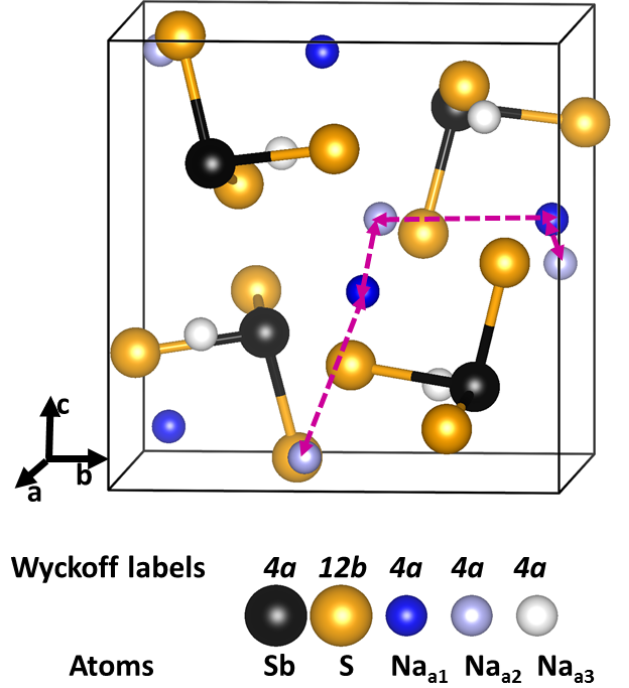
FIG. 3. Ball and stick model of \text{Na}_3\text{SbS}_3 in its P2_13 crystal structure, using black and orange balls to indicate Sb and S sites, respectively. Inequivalent Na sites are indicated with bright blue, pale blue, and white balls. The violet arrows illustrate possible vacancy migration paths between nearest neighbor Na ions on alternating a_1 and a_2 sites.
