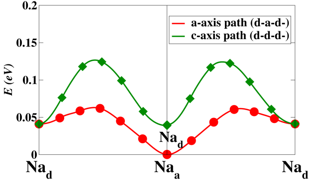
FIG. 5. Computed energy path diagram for Na-ion vacancy migrations in \text{Na}_3\text{SbS}_4 corresponding to the nearest neighbor hops indicated in Fig. 1 for migration along the a or b axes (red symbols and line) and along the c axis (green symbols and line). The symbols represent directly calculated configurations while the lines are smooth interpolations between NEB images. The zero of energy is set at the energy of a Na-ion vacancy at a \text{Na}_a site.
