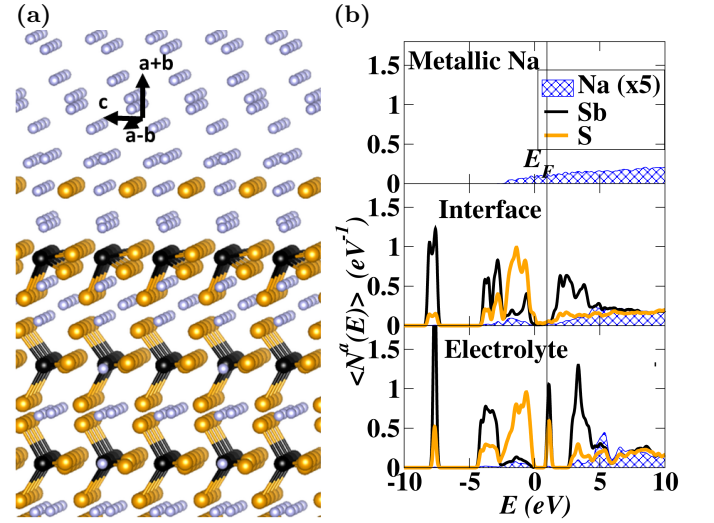
FIG. 11. (a) Ball and stick model of the simulated relaxed structure of a \text{Na}_3\text{SbS}_4 surface oriented along the (110) direction and interfaced with Na metal. The ball conventions for Sb and S is the same as in Fig. 1 and light blue balls represent both ionic and metallic Na. The indicated axes reference the \text{Na}_3\text{SbS}_4 lattice. (b) Corresponding partial densities of states analysis of this system, separately indicating the interior of the electrolyte, the interface region, and the metallic region in the bottom, middle, and top panels, respectively.
