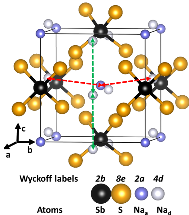
FIG. 1. Ball and stick model of \text{Na}_3\text{SbS}_4 in the tetragonal P4_21c structure, using black and orange balls to indicate Sb and S sites, respectively. Inequivalent Na sites are indicated with blue and white balls. The red arrows illustrate possible vacancy migration paths between neighboring a and d sites, while the green arrows illustrate possible vacancy migration paths between neighboring d sites.
