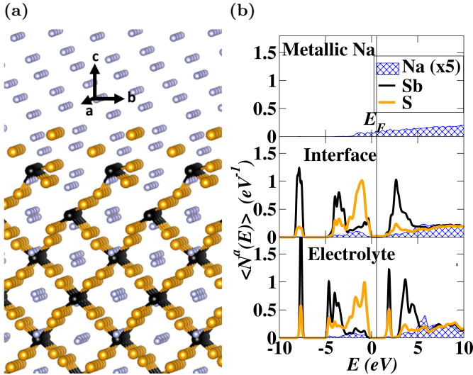
FIG. 10. (a) Ball and stick model of the simulated relaxed structure of a \text{Na}_3\text{SbS}_4 surface oriented along the (001) direction and interfaced with Na metal. The ball conventions for Sb and S is the same as in Fig. 1 and light blue balls represent both ionic and metallic Na. The indicated axes reference the \text{Na}_3\text{SbS}_4 lattice. (b) Corresponding partial densities of states analysis of this system, separately indicating the interior of the electrolyte, the interface region, and the metallic region in the bottom, middle, and top panels, respectively.
