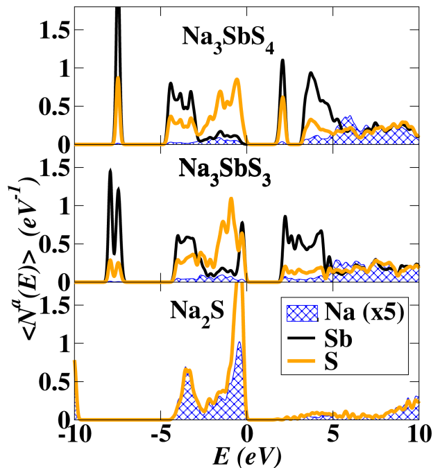
FIG. 4. Partial densities of states for the ground state structures of \text{Na}_3\text{SbS}_4 , \text{Na}_3\text{SbS}_3 , and \text{Na}_2\text{S} . The zero of energy in these plots is taken as the top of the valence band of each material.
