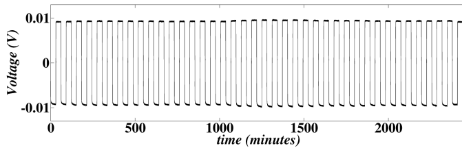
FIG. 8. Experimentally measured voltage versus time plot for a Na/Na 3 SbS 4 /Na symmetric cell cycled 40 times with a current density of 0.1 mA/cm 2 and holding the positive and negative voltages for 30 minutes.
