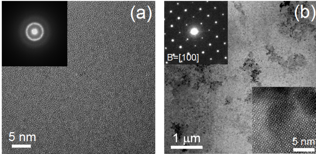
FIG. 2. Bright-field transmission electron microscopy (TEM) images of the (a) as quenched Al-10at.%Sm melt-spun ribbons, and the (b) \epsilon\text{-Al}_{60}\text{Sm}_{11} in Al-10at.%Sm annealed at 470 K for 9 min. Inset: corresponding selected area diffraction (SAD) pattern and high-resolution high angle annular dark field (HAADF) image.
