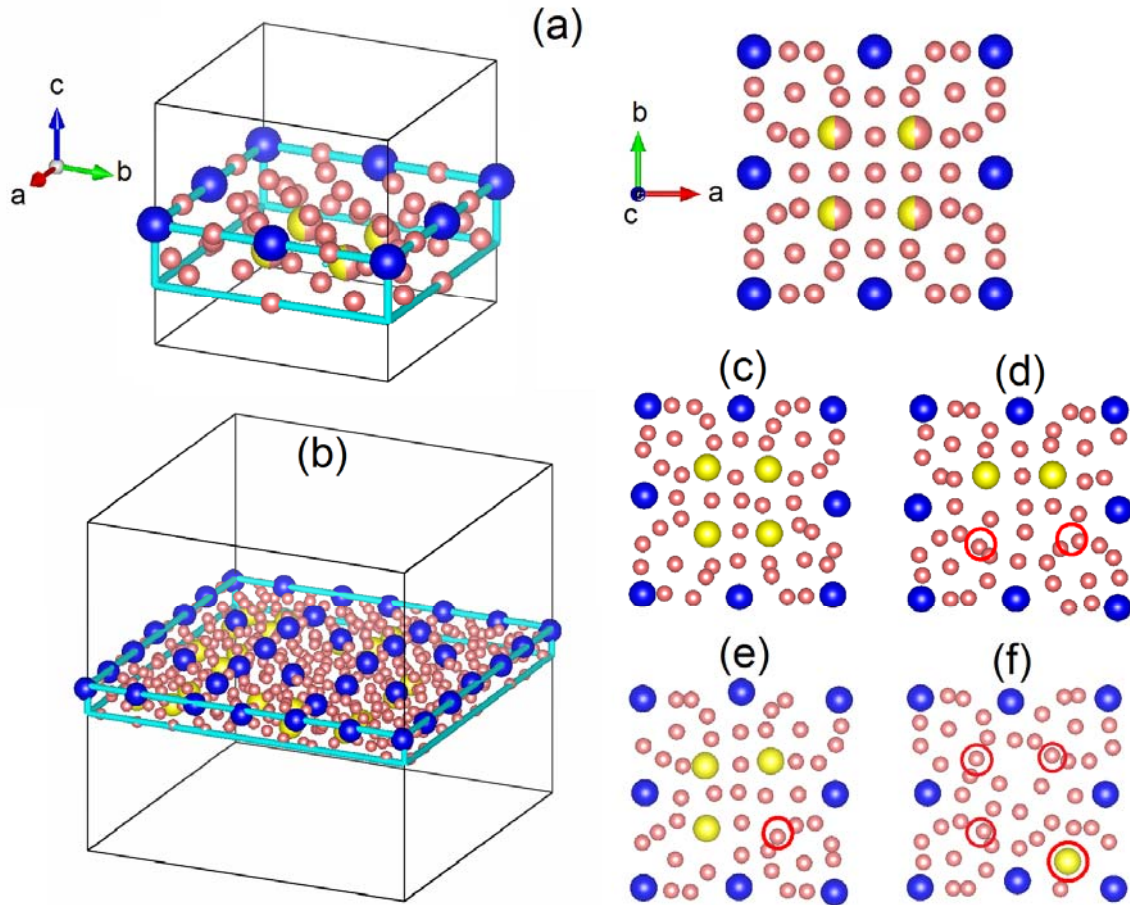
FIG. 6. A comparison of defects suggested by Rietveld analysis and by MD simulations. (a) A slice with a thickness of \frac{1}{2} of the structure suggested by Rietveld analysis. (b) A slice with the same thickness from the grown \epsilon -Al 60 Sm 11 supercell structure. (c)-(f) Different locations in the slice shown in Fig. 6(b) to provide a close look of the 16f defects as marked in red circle.
