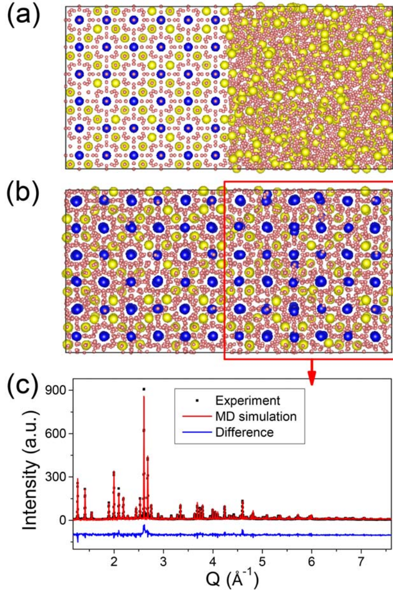
FIG. 5. MD simulation results. (a) Refined structure \epsilon\text{-Al}_{60}\text{Sm}_{11} in Fig. 4 serves as a seed (left part) to grow the crystalline structure from undercooled Al-10%Sm liquids (right part). (b) The \epsilon\text{-Al}_{60}\text{Sm}_{11} (bcc) structure is fully grown within 300 ns. The Sm atoms (blue) outline the cubic frame, with randomly distributed Sm-Al anti-sites (yellow). (c) The XRD pattern of the grown structure compared with experiment.
