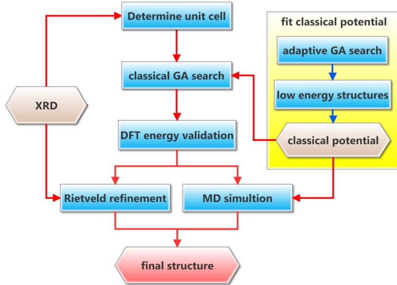
FIG. 3. A schematic flow diagram of our integrated approach.
