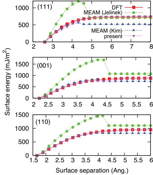
FIG. 4. Energy versus separation for rigid block separation across the (111), (110), and (100) surfaces of bulk Al, as computed via DFT, two MEAM potentials, and the present NN potential. These structures are included in the training data.
