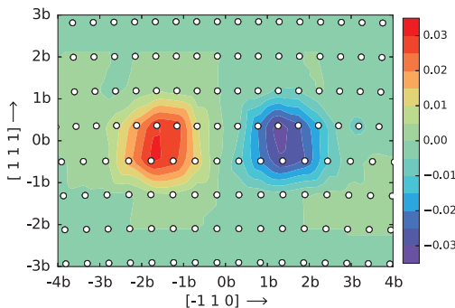
FIG. 3. Nye tensor distribution of the screw component of the Burgers vector for the dissociated edge dislocation core in pure Al; the result agrees well with direct DFT 28,29 x - and y -axes are in units of the Burgers vector b = 2.86 \text{ \AA} . This structure is not in the training data.
