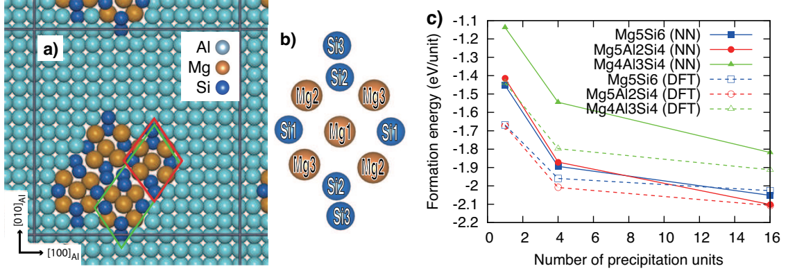
FIG. 7. a) Typical simulation cell of Mg 5 Si 6 precipitate of N_{\text{FU}} = 4 in Al matrix, which corresponds to 7 \times 7 \times 1 FCC Al cell. The system is periodic in z -direction, [001]_{\text{Al}} . The green rectangle indicates a monoclinic cell of Mg 5 Si 6 . b) Formation unit of Mg 5 Si 6 indicated in the red rectangle in a). In case of Mg 5 Al 2 Si 4 , Si 3 sites in Mg 5 Si 6 are replaced by Al, while Mg 1 site is also replaced by Al in Mg 4 Al 3 Si 4 . c) Size dependency of the precipitation energy of Mg 5 Si 6 , Al 2 Mg 5 Si 4 and Al 3 Mg 4 Si 4 obtained by the NN potential and the DFT (from D. Giofré et al. 19 ) These structures are not in the training data set.
