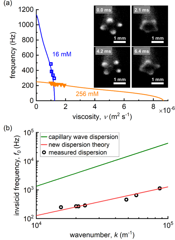
Figure 2. (a) Pattern oscillation frequencies measured using high-speed imaging (inset) for various solution viscosities and ionic strengths. (b) The inviscid frequency f_0 for \nu = 0 and wave number k were extrapolated using equation (4) for various values of ionic strength. Extrapolated inviscid frequencies are compared to the traditional capillary wave dispersion and equation (5).
