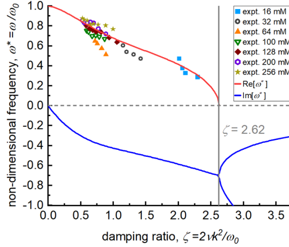
Figure 4. The physical roots of equation (6) as a function of \zeta consist of a frequency component, \text{Re}[\omega^*] plotted in red, and a damping rate, \text{Im}[\omega^*] plotted in blue. Non-dimensionalized frequency data, for various values of solution viscosity and ionic strength, collapse onto the real part of the root of equation (6).
