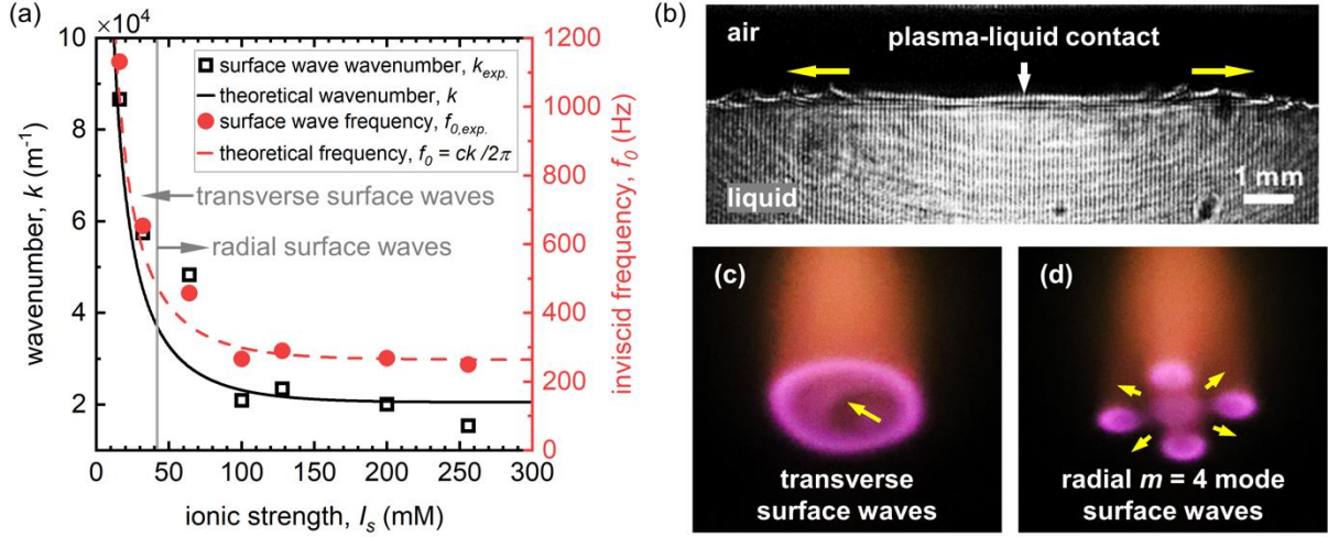
Figure 3. (a) Extrapolated wavenumbers k (black open squares) and inviscid frequencies f_0 (red solid circles) as a function of ionic strength. Curves depict theory based on equation (1) for k and f_0 = ck/2\pi , where the empirical values for j_\infty and b in equation (3) were used from [15]. Plasma parameters of n_0 = 2.35 \times 10^{18} \text{ m}^{-3} and I = 26.2 \text{ mA} were used for the theoretical lines. (b) Side-view still frame of the plasma impinging on the liquid surface, inducing surface waves propagating radially outward at a measurable phase velocity c . Photographs of (c) a deformed ring with induced transverse waves at 32 mM and (d) the four spots with radial waves at 48 mM. The yellow arrows indicate the propagation direction of the waves.
