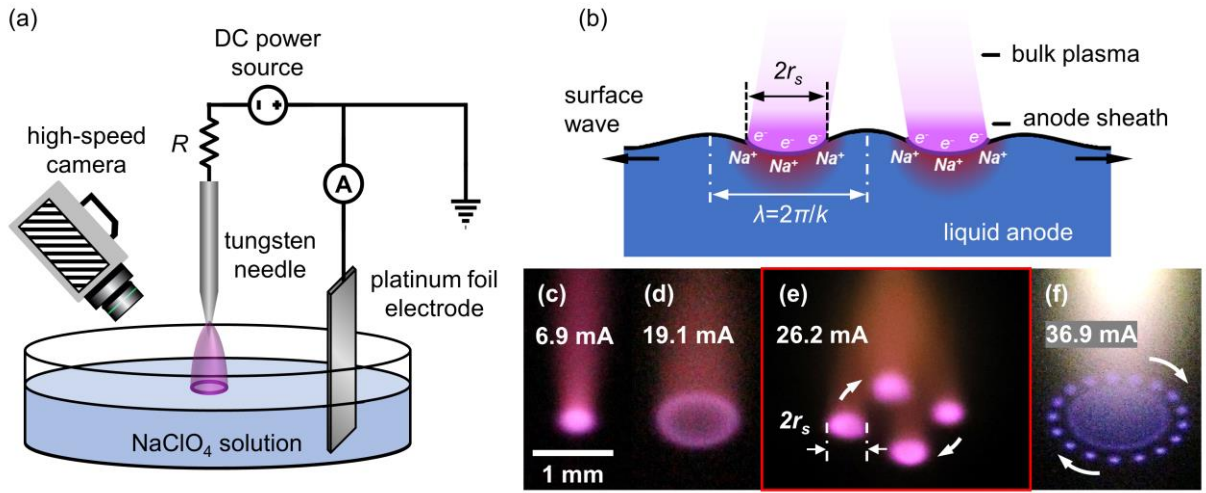
Figure 1. (a) Schematic of liquid anode glow discharge system. The discharge is generated by applying DC voltage through a ballast resistor R to a needle cathode suspended above a liquid surface with a submerged, grounded counter-electrode. (b) Illustration of the electrostatics of the plasma-liquid interface. The space charge field in the plasma's anode sheath induces waves on the liquid surface, whose wavelength is determined by the reaction and diffusion of electrons in the anode sheath. (c)-(f) show patterns for a 128 mM \text{NaClO}_4 solution. As the current increases in the system, the plasma progresses from a uniform spot (c) to a continuous annular ring (d). At higher currents, the annular ring breaks into four spots (e) and oscillates between the two conditions. At still greater currents, a more complex pattern (f) is observed.
