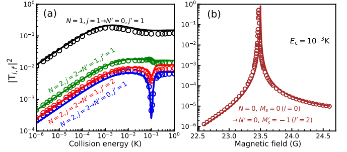
FIG. 4. (a) Collision energy dependence of transition probabilities between the different fine-structure levels of {}^{14}\text{NH} in ultracold collisions with \text{Mg} atoms. Solid lines – MQDT-FT calculations, open circles – exact CC results obtained using the recoupling FT. All results are for a single incident s -wave component ( l = 0 ) and summed over all final l' . (b) Magnetic field dependence of the spin relaxation probability in cold \text{Mg} + {}^{14}\text{NH}(N = 0) collisions. Solid line – MQDT-FT calculations, open circle – exact CC results. The quantum numbers for the initial and final states involved in each transition are indicated next to the corresponding curves.
