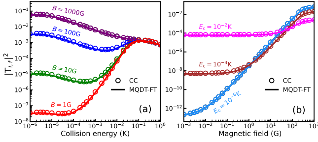
FIG. 1. Probabilities for the spin relaxation transition M_S = 1 ( l = 0 ) \rightarrow M'_S = 0 ( l' = 2 ) in cold Mg + ^{14}\text{NH} ( N = 0 ) collisions plotted as a function of collision energy (a) and magnetic field (b). Solid lines – MQDT-FT calculations, open circles – exact CC results.
