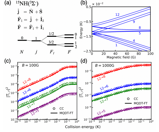
FIG. 2. Hyperfine energy levels of ^{15}\text{NH} ( N = 0 ) at zero field (a) and as a function of magnetic field (b). State-to-state transition probabilities |T_{il,f'l'}|^2 plotted as a function of collision energy at B = 100 G (c) and B = 1000 G (d) for Mg + NH ( N = 0 ) collisions for l = 0 and l' = 2 . Solid lines – MQDT-FT calculations, open circles – exact CC results. The initial and final states of NH are indicated next to each curve as i \rightarrow f [see panel (b)].
