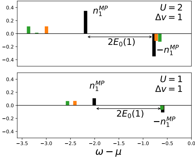
FIG. 2: Spectral function differences \Delta A_{11}(\omega) with \mu = U/2 and t = 1/2 . Exact (black), one-shot (orange), and 2psGW (green). The separation of the SP and MP poles is twice the energy of the one-particle groundstate, but GW introduces an erroneous interaction dependence.
