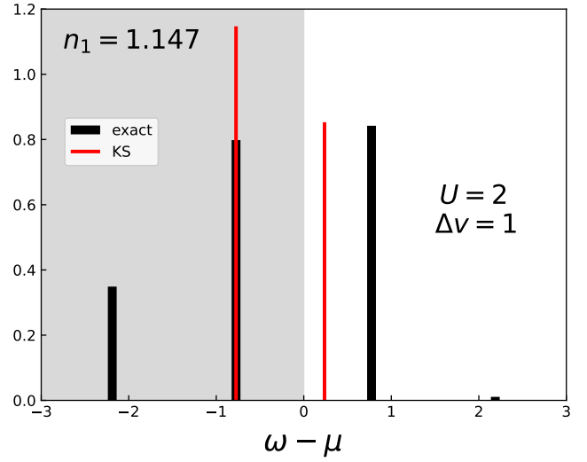
FIG. 1: Hubbard dimer local spectral functions A_{11}(\omega) (black) and A_{\text{s},11}(\omega) (red). Here \mu = U/2 and t = 1/2 . The spectral weight below 0 sums to n_1 = 1.147 , and above to n_2 .
