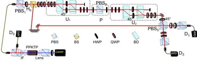
FIG. 1. Experimental setup. Heralded single photons are created via type-II spontaneous parametric down-conversion in a PPKTP crystal. The polarizing beam splitter PBS 1 and the half-wave plate (HWP) H 0 are used to generate initial polarization states |H\rangle and |V\rangle . After photons pass through a 50 : 50 beam splitter (BS), the transmitted photons enter the evolution path, and the reflected photons act as reference photons and interfere with the transmitted photons at PBS 3 . The evolution process involves nonunitary evolutions U_1 and U_2 realized by two beam displacers (BDs) and sets of wave plates and the projector P is realized by two HWPs and PBS 2 . The measurement part involves PBS 3 , two quarter-wave plates (QWPs) and two HWPs. Finally, photons are detected by avalanche photodiodes (APDs), and recorded by the coincidence counts of D 0 , D 1 and D 0 , D 2 , respectively.
