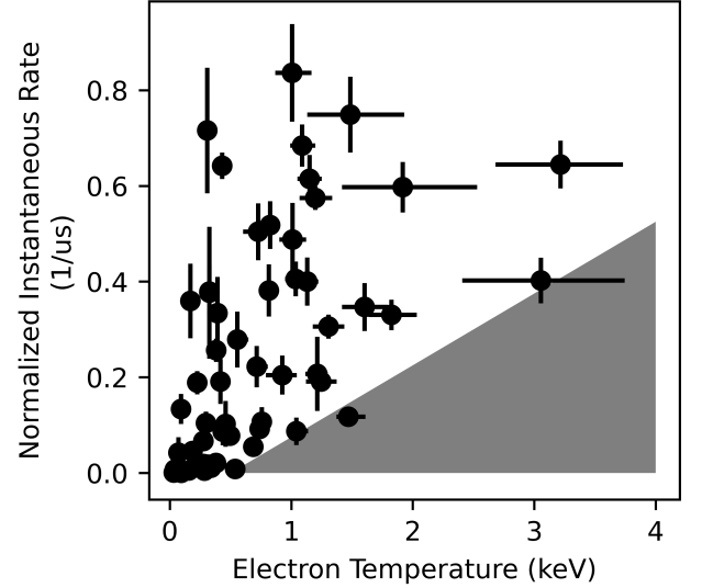
FIG. 5. Plot of the normalized instantaneous neutron production rate versus the T_e measurements. The values for rate are calculated by integrating a 200 ns window of the SPMT signal centered around the Thomson laser trigger. The triangle at bottom right indicates the region of parameter space characterized by low neutron production and high T_e , which is not observed experimentally.
