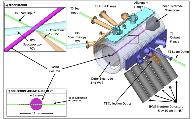
FIG. 1. The Z-pinch Assembly Region of the FuZE device and TS system, featuring three dedicated vacuum flanges for the TS system. The assembly region of the device extends from the upstream nosecone down to the endwall. Also shown are views of the UV spectroscopy measurement for T_i as well as placement of the axial SPMT array, at bottom right. a) Detail of the probe region and collection region, which is indicated by the dashed square in the main figure; b) end-on view of the idealized plasma column and radial extent of the TS collection volumes. Vertical displacements of the plasma column results in TS collection volumes that do not coincide with the Z-pinch plasma axis.
