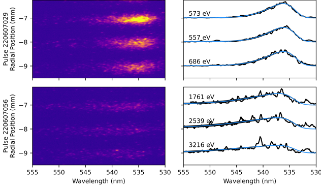
FIG. 2. Raw Thomson data (left column) and fits (right column) for three representative fibers from two FuZE pulses: pulse 220607029 on the top row and pulse 220607056 on the bottom row. The fitted T_e values are displayed in the right column for each chord.
