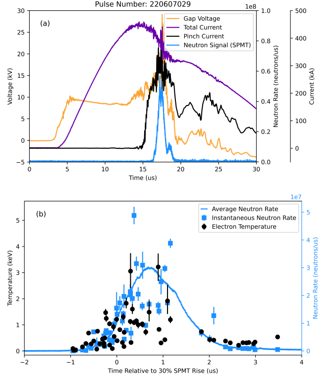
FIG. 3. (a) A typical FuZE pulse taken during this campaign. The total plasma current in the accelerator is measured at the upstream anode/cathode gap[18] and is plotted in purple; the current that makes it into the pinch is black; the voltage drop across the anode - cathode, V_{\text{gap}} , is orange; and the neutron production rate as measured by a SPMT detector is blue. The peak in V_{\text{gap}} is coincident with the peak in pinch current as well as the onset of neutron production. (b) Reconstruction of the temporal evolution of the electron temperature over many pulses on the same time scale as the neutron production rate. (The TS delay is reported with respect to the rise time of the SPMT signal, defined as 30% of peak signal.) The solid blue line is averaged over all the of relevant pulses. The blue dots are the instantaneous neutron production rate for each pulse, integrating over a 200 ns window. We observe temporal coincidence of T_e and the neutron production rate.
