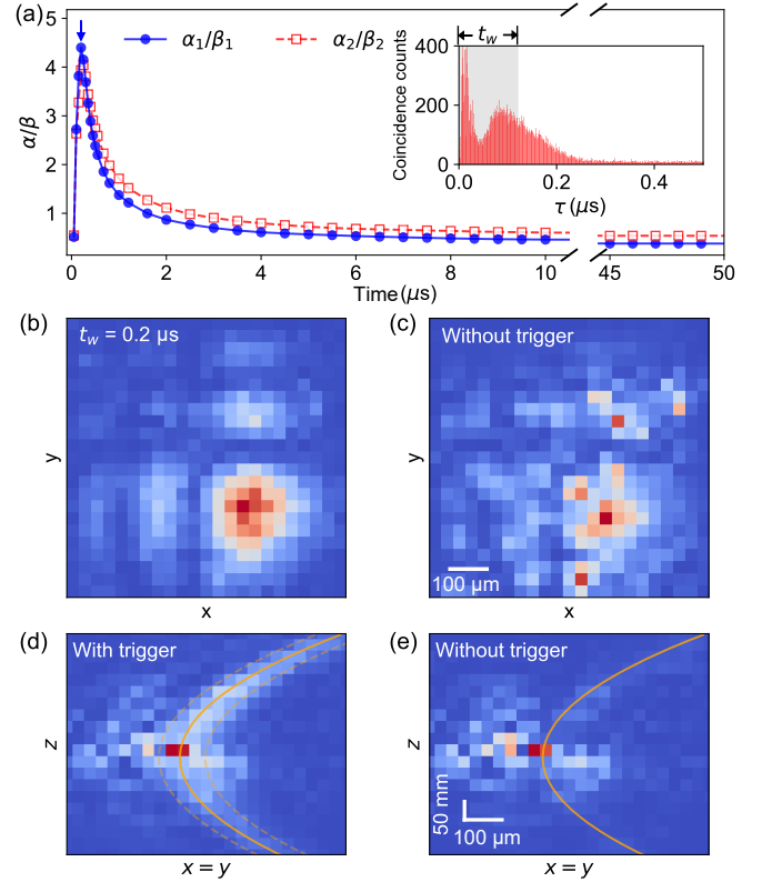
FIG. 4. Concealing correlated nondiffracting photons in classical light noise. (a) Airy to noise ratio \alpha/\beta as a function of time window t_w . Blue and red lines show two measurements with different classical noise powers. The inset depicts a typical biphoton waveform for a Gaussian pump. The blue arrow corresponds to image (b) for t_w = 0.2\mu\text{s} of collecting heralded photons, and (c) is the concealed photon pattern when no trigger was used. (d) Propagation of nondiffracting correlated Airy photons over classical noise. When triggering of Stokes photons is used the self-bending of Airy photons is clearly visible. (e) Propagation of uncorrelated thermal Airy photons over classical noise. Without triggering the strong noise masks the Airy light. The overlaid theoretical curves indicate the peak (solid) and the half-maximum (dashed).
