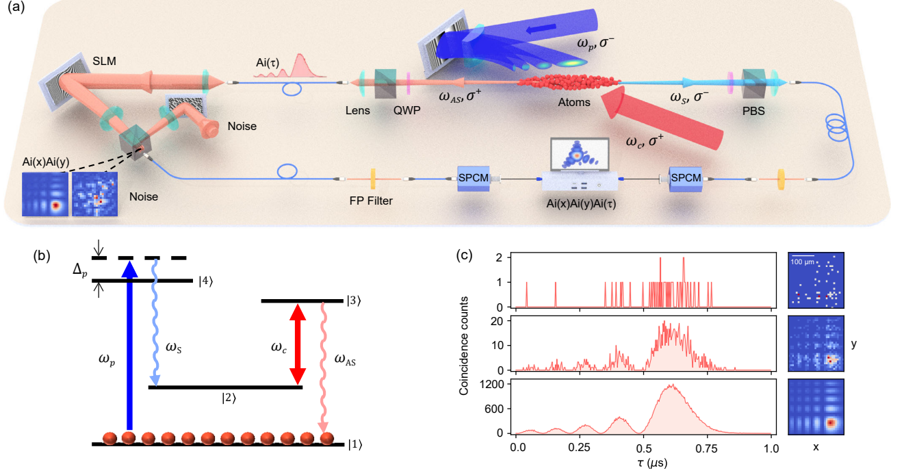
FIG. 1. Experimental scheme for the observation of spatiotemporal Airy biphotons. (a) Optical setup. Two classical circularly polarized ( \sigma ), counter-propagating beams with frequencies \omega_p (Airy) and \omega_c (Gaussian) generate circularly polarized Stokes, \omega_s , and anti-Stokes, \omega_{AS} , entangled photons via spontaneous four-wave mixing. A space-to-time mapping generates nonclassical temporal Airy biphotons Ai(\tau) . The \omega_{AS} photons are subsequently shaped into a nondiffracting Airy wave packet to form a three-dimensional spatiotemporal photon, Ai(x)Ai(y)Ai(\tau) . Single-photon counting modules (SPCM) register the photons that have been filtered by Fabry-Pérot (FP) cavities. A classical noise pattern is superimposed for correlated photon concealing. (b) Double- \Lambda configuration for spontaneous four-wave mixing. The 780 nm 1D-Airy pump beam, \omega_p , has a detuning of \Delta_p = 120 MHz, while the 795 nm coupling beam, \omega_c , is on resonance. The twin photons \omega_s (780 nm) and \omega_{AS} (795 nm) are spontaneously emitted. (c) Simulated formation of spatiotemporal quantum Airy wave packets as the photon number is increased. The temporal (left) and the spatial (right) wave packets emerge simultaneously.
