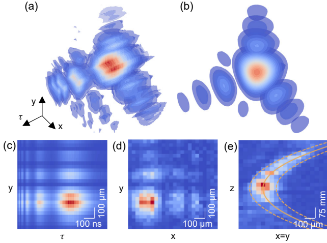
FIG. 3. A three-dimensional spatiotemporal Airy photon. Isosurface of (a) the experimentally observed |\psi_{xy\tau}|^2 of the Airy biphotons, and (b) the corresponding theoretical wave packets. The isosurfaces range from 0.1 to 1.0. The vector lengths represent x, y , and \tau scales of 100\mu\text{m} , 100\mu\text{m} , and 200\text{ns} respectively. A projection of the photon probability density (c) for the temporal \tau and spatial y distribution along the x -axis, and (d) for the two-dimensional spatial x, y -distribution along the time axis \tau . (e) Observation of the z -propagation of the spatially self-bending nonclassical Airy photons along the diagonal ( x = y ). The theoretically expected parabolic trajectories (solid for the maximum and dashed for the half-maximum) are overlaid.
