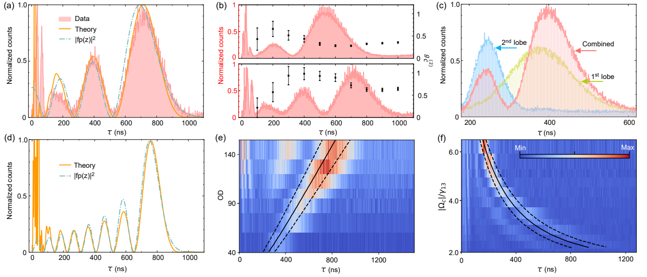
FIG. 2. Observation of temporal Airy biphotons. (a) Temporal Airy biphoton. Normalized counts of the observed biphotons (shaded pink), numerically predicted waveform (orange solid line) for OD = 150 and \Omega_c = 2\pi \times 10 MHz, and analytical prediction, from Eq. 1, (dash dotted green line) for a pump having a beam profile f_p(z) = Ai(z/z_0) \exp(az/z_0) , with z_0 = 18.7 mm, and a \approx 0.1 . (b) (top) Two- and (bottom) three-lobe Airy waveforms (shaded pink) and their corresponding self-correlations, g_c^{(2)}(\tau) (black squares). The biphoton generation rate for the two- and three-lobe waveforms during the SFWM is 470\text{ s}^{-1} and 374\text{ s}^{-1} . The error bars are calculated from the one standard deviation of the photon counts. (c) Locally probing the biphoton phase. Observed normalized counts when the Airy pump is imposed as a whole (shaded pink), with only the first lobe (shaded green), and only the second lobe (shaded blue). (d) Simulated (dash dotted green line), and analytical (orange solid line) Airy waveforms for high optical depths ( OD = 500 ). Experimentally obtained (e) temporal waveform density |\psi(\tau)|^2 as a function of OD and fixed \Omega_c = 2\pi \times 10 MHz, and (f) temporal waveform as a function of the normalized coupling Rabi frequency |\Omega_c|/\gamma_{13} for OD = 150 . The curves overlaid on the experimental data highlight the maximum (solid) and the half-maximum as determined by numerical simulations. The same colormap is used throughout the paper.
