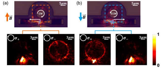
FIG. 4. Magnetically tuned single photon routing on-chip. (a), (b) Emission captured at the image plane of the device under positive and negative magnetic fields, respectively, where upper panels show the unpolarized image overlapped with the optical microscope picture of the device, and lower panels show the polarized emissions according to two photon spins. In (a), only the CW mode propagates in the microring, resulting in a strong output at the left grating coupler (upper). The result is consistent with the polarized emissions, as the CW mode carries opposite transverse spins of \sigma_+ at the outer sidewall and \sigma_- at the inner sidewall. Direct emission confirms the quantum emitter at the outer sidewall to be \sigma_+ -polarized (lower left), which can couple into the CW mode and subsequently lead to the \sigma_- -polarized ring-shaped emission from the angular grating at the inner sidewall (lower right). In (b), a strong output is observed at the right grating coupler, confirming the magnetic switching of the circulating mode to CCW and thus routing to the right direction in the bus waveguide (upper). Consequently, direct emission shows the quantum emitter to be \sigma_- -polarized (lower right) and the ring-shaped emission is \sigma_+ -polarized (lower left), consistent with excitation of the CCW mode that carries \sigma_- at the outer sidewall and \sigma_+ at the inner sidewall.
