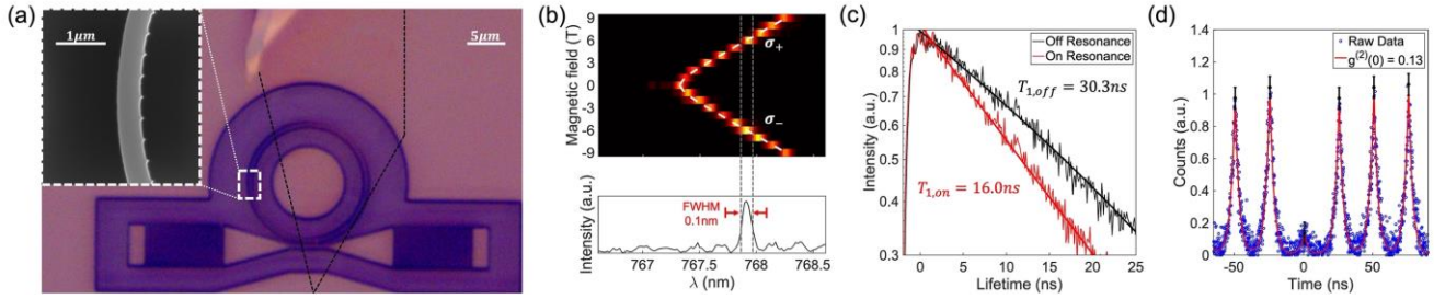
FIG. 2. Characterization of quantum light emission. (a) Optical microscope image of the device: a microring coupled with a bus waveguide connected with two grating couplers fabricated on a \text{Si}_3\text{N}_4 -on- \text{SiO}_2 platform. A monolayer \text{WSe}_2 flake is transferred on top to form the quantum emitter on the ring, marked by the black dotted line. Inset shows the scanning electron microscope graph of the microring resonator where equidistant scatterers ( M = 92 in total) are inscribed at the inner sidewall. (b) Spontaneous emission spectrum of the quantum emitter under an external magnetic field from -9 T to 9 T (upper panel) versus the cavity resonance spectrum measured with a broadband input from a grating coupler and signal collection from the angular grating (lower panel). The comparison evidently shows, at B = 6.0 T or -6.0 T, the \sigma_+ or \sigma_- emission branch can be tuned on resonance, respectively, with the cavity mode centered at 767.9 nm (corresponding to the resonance order of N = 99 ) with a full width at half maximum (FWHM) of 0.1 nm. (c) Measured time-resolved photoluminescence spectra show a photon lifetime reduction from 30.3 ns to 16.0 ns when the quantum emitter is tuned from off-resonance (black) to on-resonance (red). (d) Second-order photon correlation histogram (blue dots) and its data fit (red curve) exhibit pronounced antibunching with g^{(2)}(0) = 0.13 \pm 0.06 .
