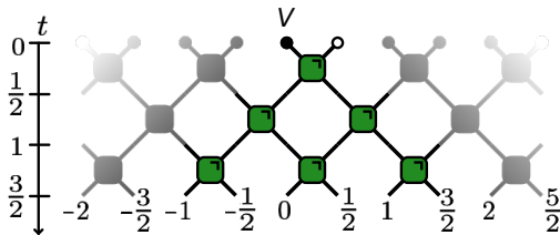
FIG. 1. Brickwork circuit models of dynamics consist of repeated 2-site unitaries on a one dimensional lattice. Time goes from top to bottom, and the lightcone for a single-site operator V is shown in green.
