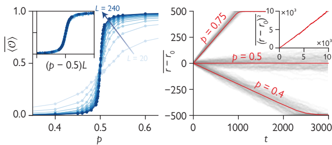
FIG. 2. Classical transition. (left) Realization-averaged order parameter \langle \mathcal{O} \rangle for various system sizes. The crossing near p = 0.500(1) is where the transition occurs. (Inset) Collapse indicates that \nu = 1.00(2) . (right) The position of the FDW initialized at L/2 for L = 1000 in the controlled phase ( p = 0.75 ), the uncontrolled phase ( p = 0.4 ) and at the transition ( p = 0.5 ). Gray curves are all 1000 realizations and red curves are averages. (Inset) At p = 0.5 we see random walk behavior in four orders of magnitude for r^2 = t and a fit confirms z = 2.04(8) .
