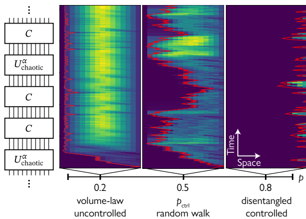
FIG. 1. Control transition. The quantum transition is seen in the dynamics of single trajectories, shown above for L = 16 . (left) A realization of the stochastic quantum circuit composed of unitary dynamics U_{\text{chaotic}}^\alpha and a nonunitary control map C . (right) The phase diagram as a function of the control probability p (black horizontal line). For p < p_{\text{ctrl}} , the domain wall between controlled and uncontrolled regions (red) is swept left; entanglement (color scale with brighter colors indicating higher entanglement) grows behind it in a volume-law fashion. For p > p_{\text{ctrl}} , the domain wall is pinned to the right edge, and the region to its left is controlled and disentangled. At p = p_{\text{ctrl}} , the domain wall undergoes an unbiased random walk and the entanglement grows to an O(1) value.
