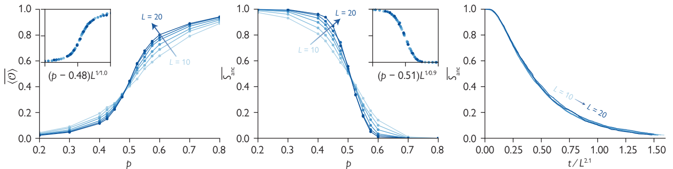
FIG. 3. Quantum transition. (left) Order parameter \langle \mathcal{O} \rangle at t = 2L^2 averaged over initial states and circuit realizations. Inset shows scaling collapse assuming \nu = 1.0(1) and p_{\text{ctrl}} \approx 0.48(1) . (middle) Ancilla entanglement order parameter S_{\text{anc}} (in units of \ln 2 ) at time L^2/2 averaged over initial states and circuit realizations. Inset shows scaling collapse assuming \nu = 0.9(1) and p_{\text{ctrl}} \approx 0.51(1) . (right) Dynamics of \overline{S_{\text{anc}}} collapsed as a function of rescaled time t/L^z near the control transition ( p = 0.5 ) with z = 2.1(1) . Data are averaged over 2000 realizations for L = 10, \dots, 16 , and 1000 realizations for L = 18, 20 . (For \overline{S_{\text{anc}}} data, 500 realizations are used for L = 20 .) All points have error bars indicating standard error of the mean; where not visible, they are smaller than the points.
